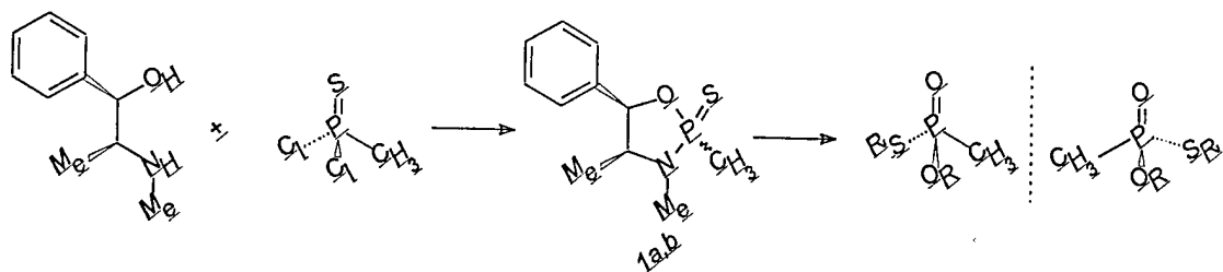
Scheme 1 - Original
