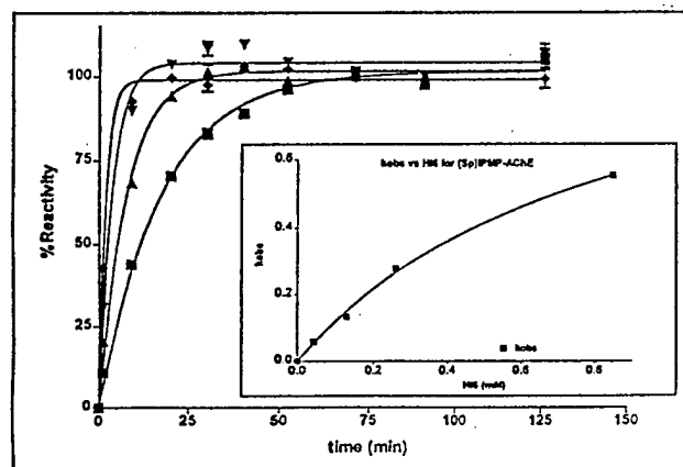
Fig. 3: Reactivation of S_p -IPMP-AChE by varying concentrations of HI-6, 0.0425mM, \blacktriangle , 0.128mM; \blacktriangledown , 0.25mM; \blacklozenge , 0.85mM. Inset shows the concentration dependence for the rate constant of reactivation.
