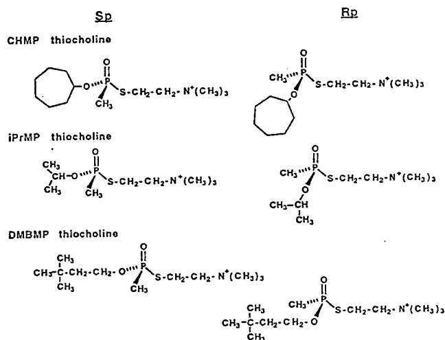
Fig. 2: Structures of the cationic compounds employed. CHMP, iPrMP and DMBMP refer to cycloheptyl-, isopropyl- and 3,3-dimethylbutyl-methylphosphonyl.
