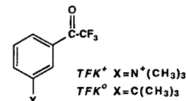
FIGURE 1: Structures of ligands used in the analysis. The leaving group is denoted by X, and the alkyl substituent is denoted by R for the alkyl phosphonates.
