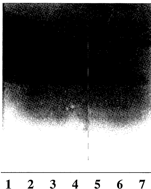
Fig. 3. Electrophoretic analysis of native and deglycosylated mAChE. SDS-PAGE (15% resolving/5% stacking gel, 20 cm \times 20 cm) under reducing conditions: lanes 1 and 6, purified mAChE; lanes 2 and 7, BSA (66 kDa); lanes 3 and 4, mAChE deglycosylated with PNGaseF; lane 5, BSA treated with PNGaseF. The thin band at the bottom of the gel corresponds to PNGaseF (36 kDa, lanes 3, 4, and 5).
