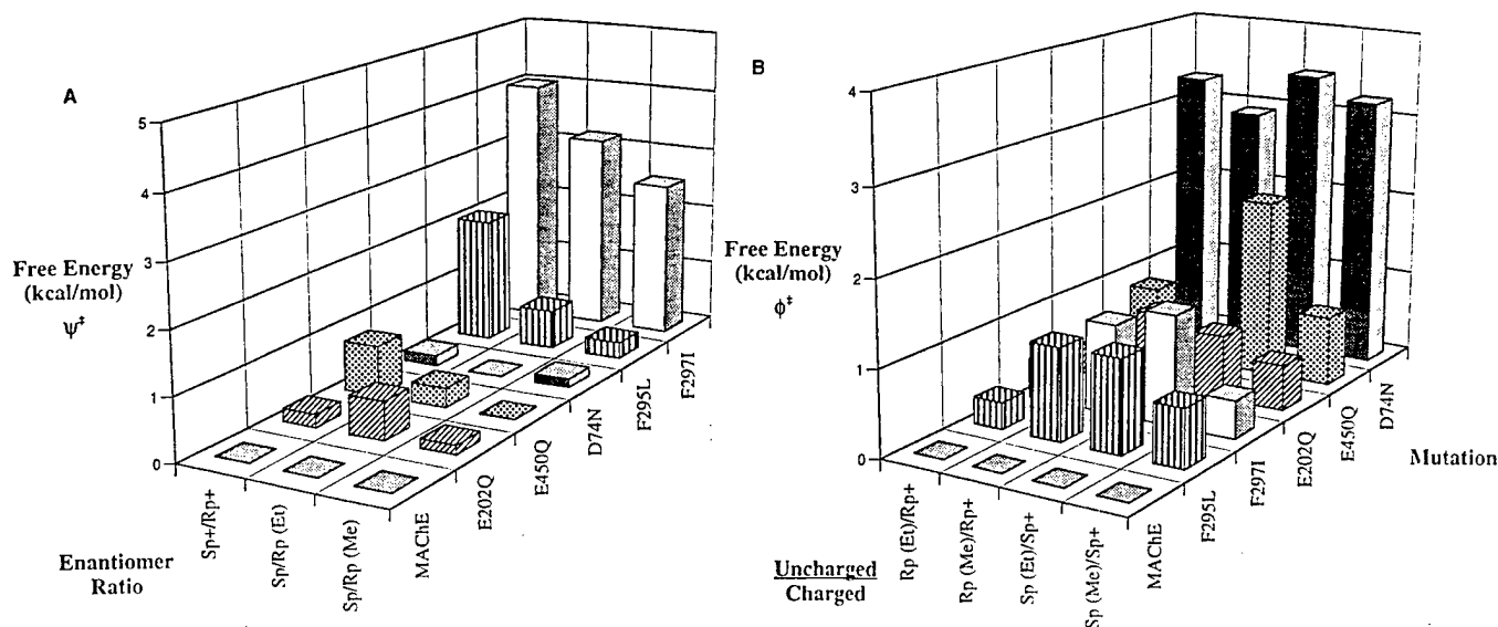
Fig. 1: Relationship between the change in free energy of activation, selected mutations in acetylcholinesterase, and structures of cycloheptyl methylphosphonyl thioates. (A) Selectivity for the S_p and R_p enantiomers. (B) Selectivity for charged and uncharged phosphonates: +, cationic cycloheptyl methylphosphonyl thiocholine; Me, uncharged cycloheptyl methylphosphonyl thiomethane; and Et, uncharged cycloheptyl methylphosphonyl thioethane. The scheme for the thermodynamic mutant cycle analysis is shown in Hosea et al., 1996, appendix.
