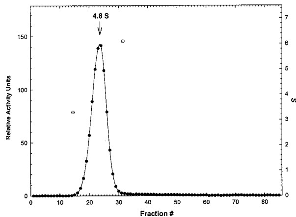
Fig. 2. Hydrodynamic analysis of mAChE-containing harvested culture media. The sample (100 \mu L), supplemented with sedimentation standards, was centrifuged in a 3–20% sucrose gradient in the presence of Triton X-100, then fractionated as described in the text. Sedimentation positions of two standards, carbonic anhydrase (3.3 S) and alkaline phosphatase (6.1 S), are shown as dotted open circles.
