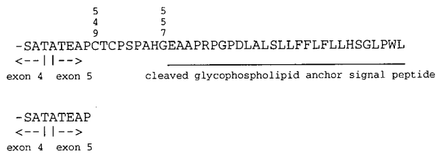
Fig. 1. Carboxyl-terminal sequences of native and truncated mouse AChE. The signal for the attachment of the hydrophobic glycopospholipid to Gly 557 in the processed native enzyme (top sequence) has been eliminated by insertion of a stop codon in place of the Cys 549 codon. The resulting enzyme, mAChE, is monomeric and devoid of a carboxyl-terminal hydrophobic segment (bottom sequence). Sequence Ser-Ala-Thr is encoded by the end of exon 4; sequence Ala-Thr-Glu is encoded by the beginning of exon 5 (Li et al., 1993). Mouse AChE residue numbering is used.
