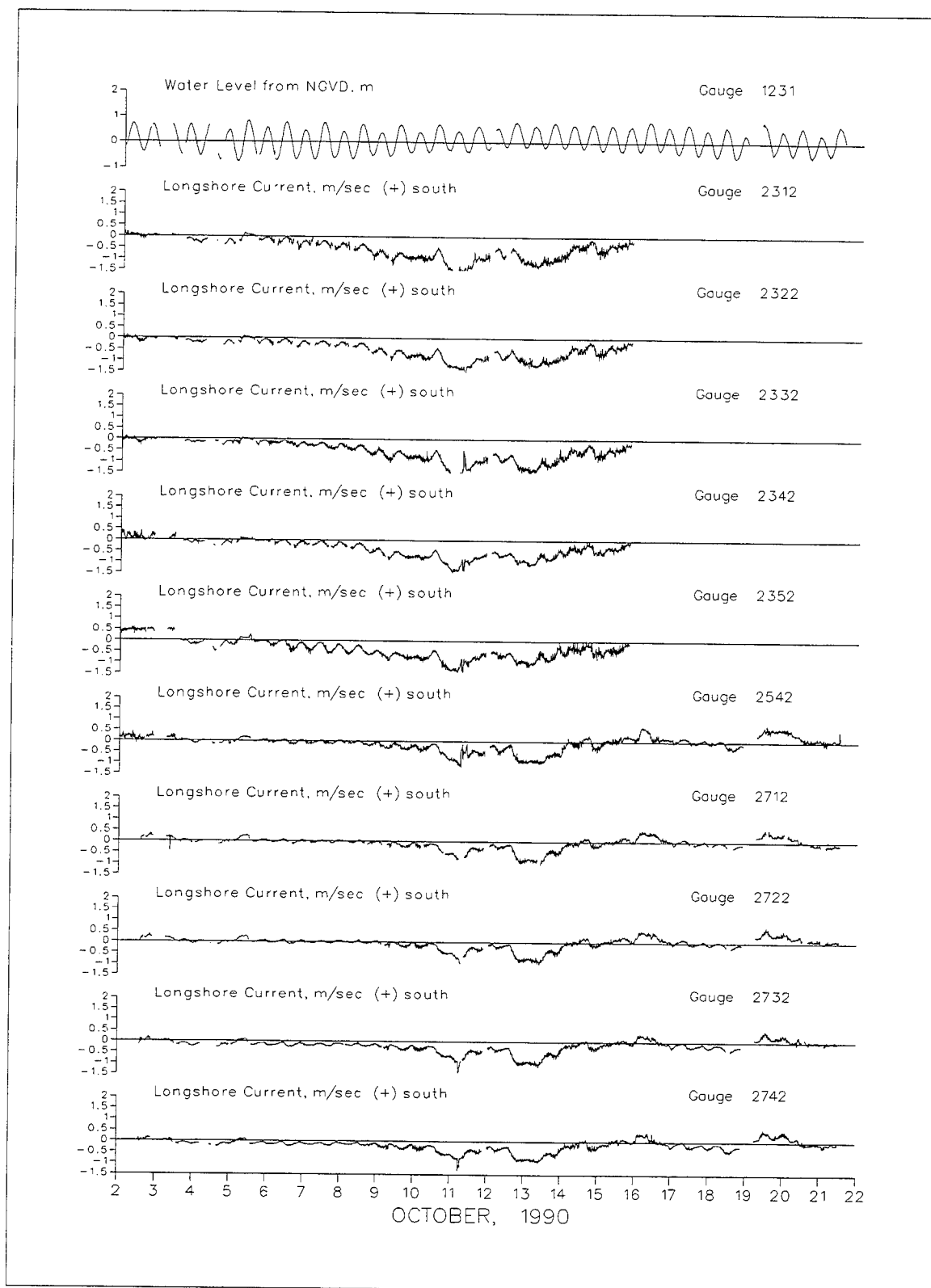
Figure E9. Long shore currents, trough and crest subarrays
