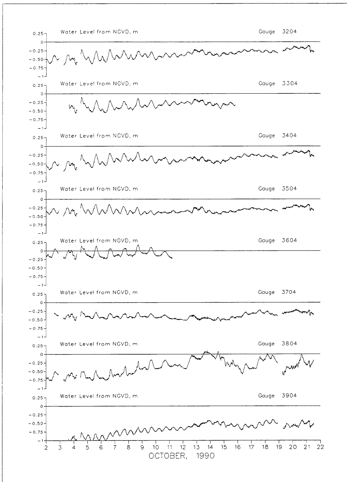
Figure E4. Changes in water levels for current meters resulting from comparison to 8-m array Paroscientific pressure gauge 231
