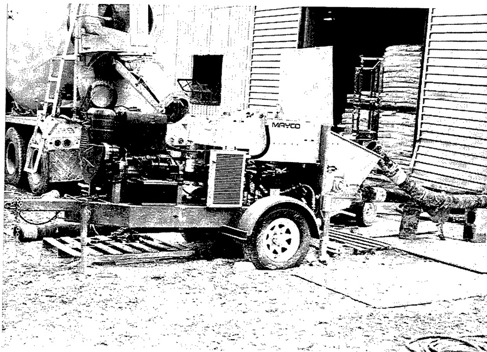
Figure 8. View of reciprocating two-cylinder pump used for pumping mud
