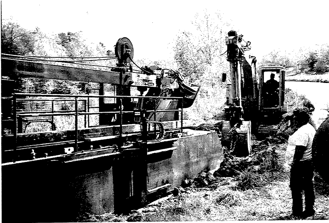
Figure 20. Dry DREdge™ being dragged towards lake
