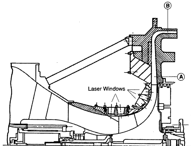
Figure 1: Centrifugal Compressor Flow Path With Laser Windows.
