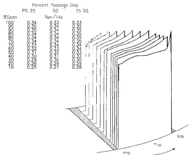
Figure 7: Distribution of through-flow velocities measured on a plane located at 5% of main blade chord
