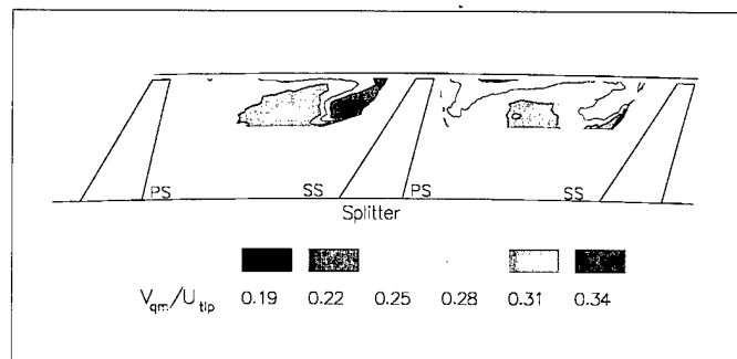
Figure 14: Contours of through-flow velocity measured on a plane located at 84% of main-blade chord
