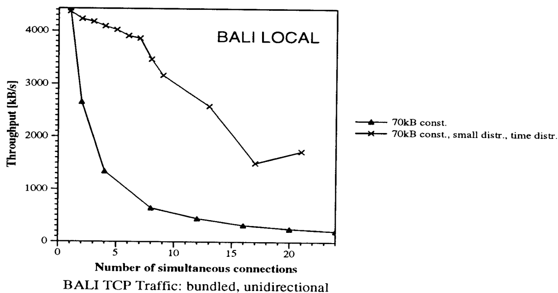
Figure 21 - Impact of Unidirectional Bundling of Connections on the Throughput of Connections with Constant TSDU and Interarrival Times on ATM LAN
