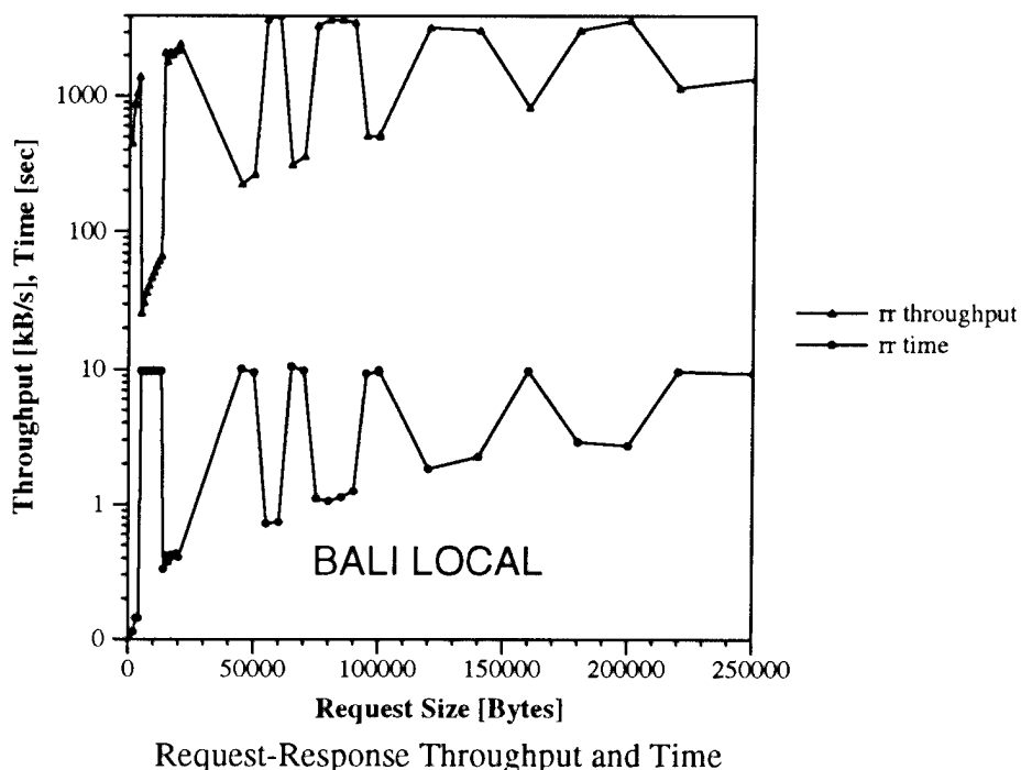
Figure 19 - Impact of TCP Specific Slowstart Mechanisms on the Response Time of Transaction Oriented Applications on ATM LAN
