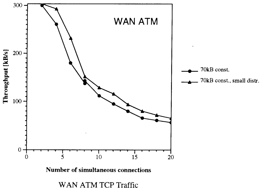
Figure 24 - Impact of Bidirectional Bundled Connections on Throughput in ATM WAN
