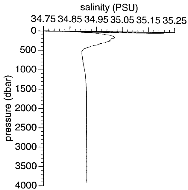
Figure 3.3.d. CTD salinity profile at Station 13.
