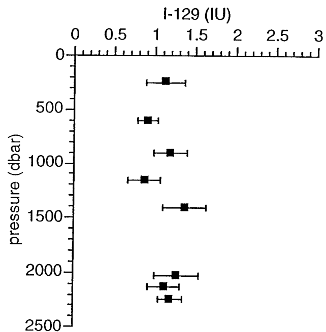
Figure 3.9.a. ^{129}\text{I} profile at Station 6, on the western flank of the Reykjanes Ridge.
