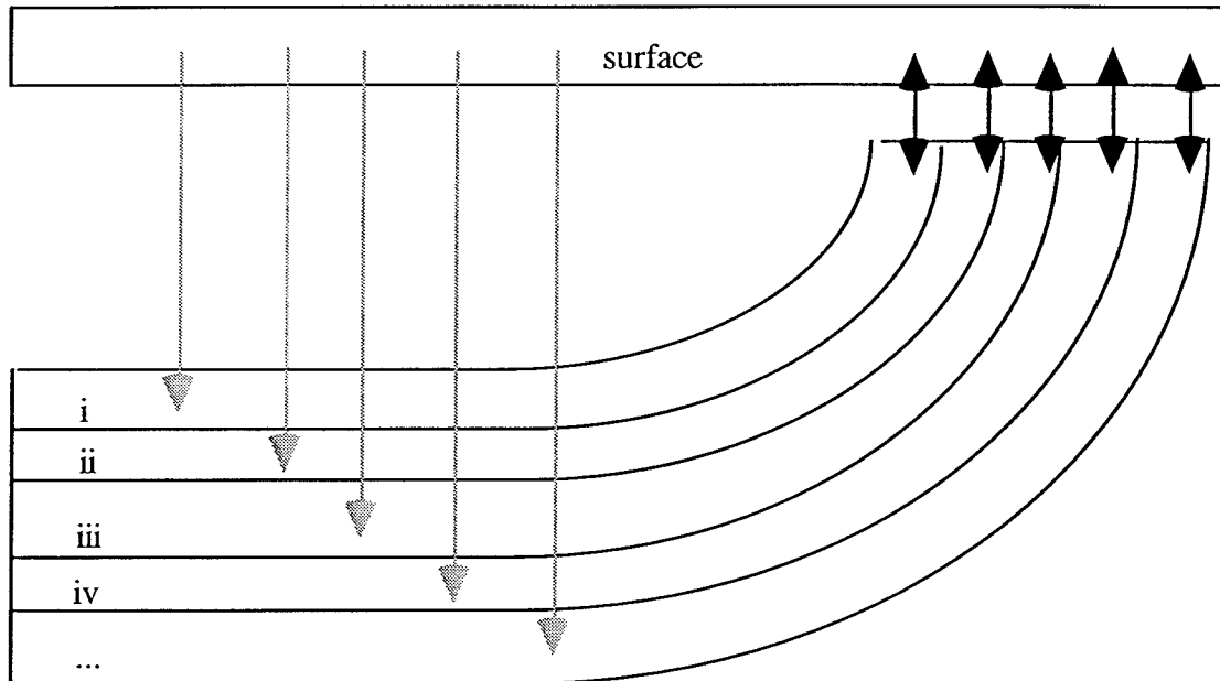
Figure 4.11. Schematic drawing of the ventilated thermocline box model, after Sarmiento et al. (1990). As in the previous models, gray arrows represent particulate fluxes. Thermocline boxes represent isopycnal surfaces (described in Tables 4.3 and 4.4). There is no mixing across isopycnals.
