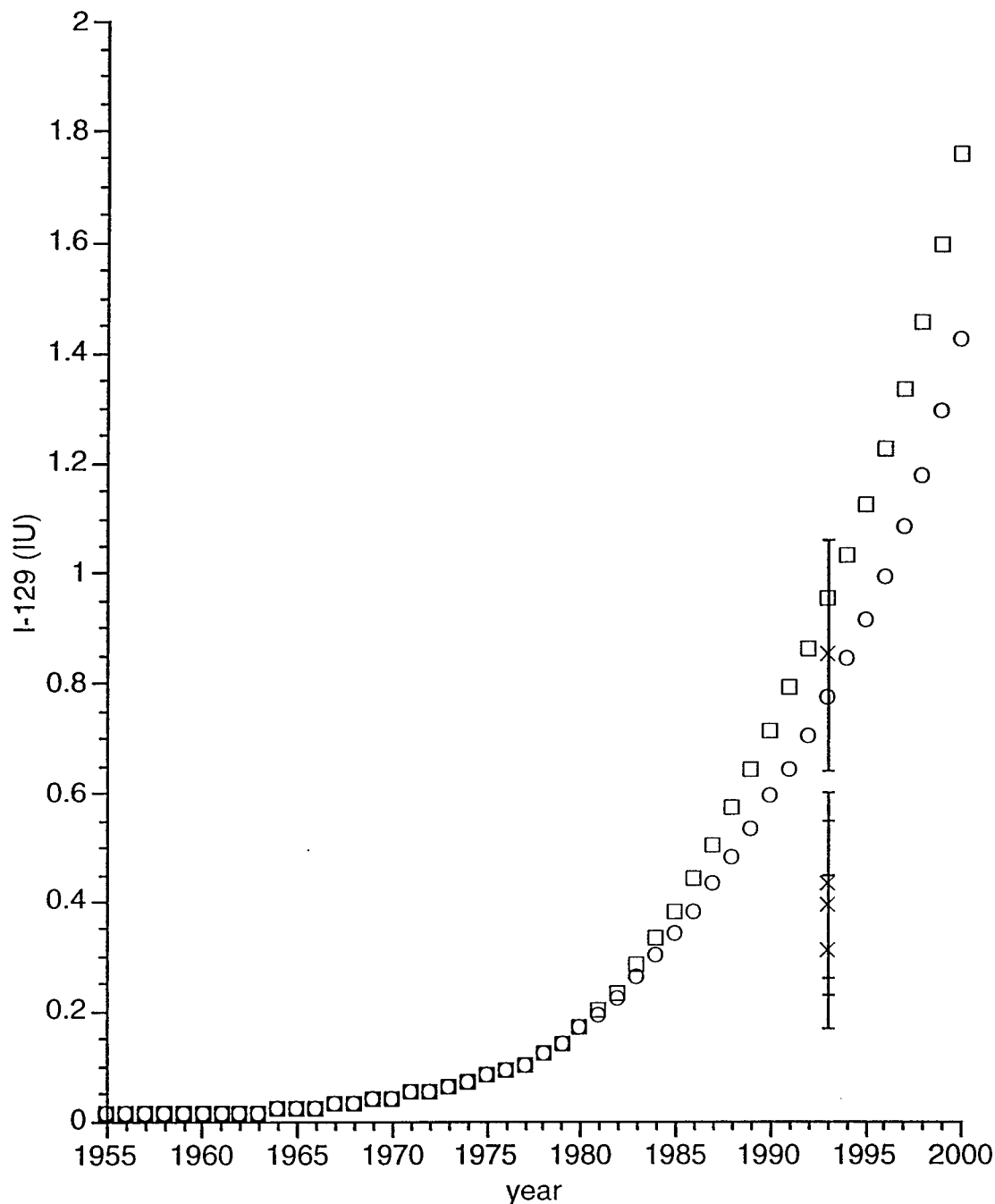
Figure 4.4. Modeled I-129 concentrations in Norwegian Sea Deep Water, with constant (squares) and reduced (circles) GSDW formation, compared with observations made in 1993 (x's, Hudson Station 13, Chapter 3).
