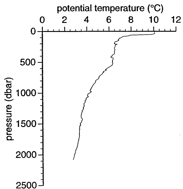
Figure 3.8.c. CTD temperature profile at Station 5.
