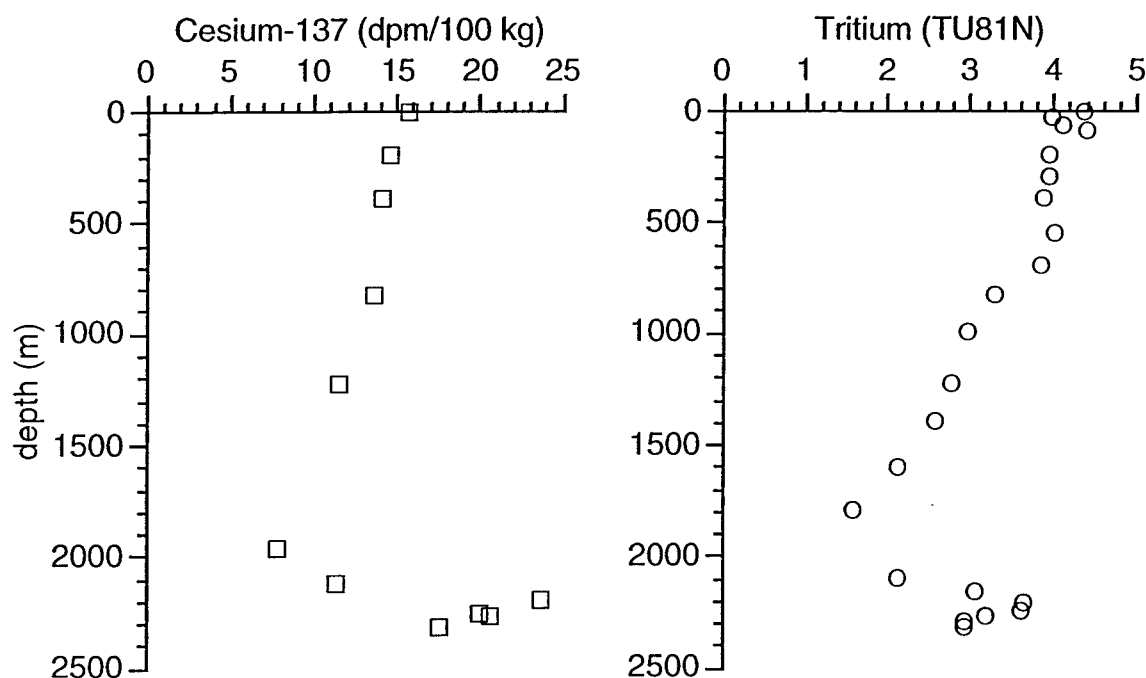
Figure 3.15. Cesium-137 and tritium (decay-corrected to 1/1/81) profiles at TTO Station 167 south of the Denmark Straits, 64°4.5'N 33°19.6'W, 8/13/81. The data are from Livingston et al. (1985).
