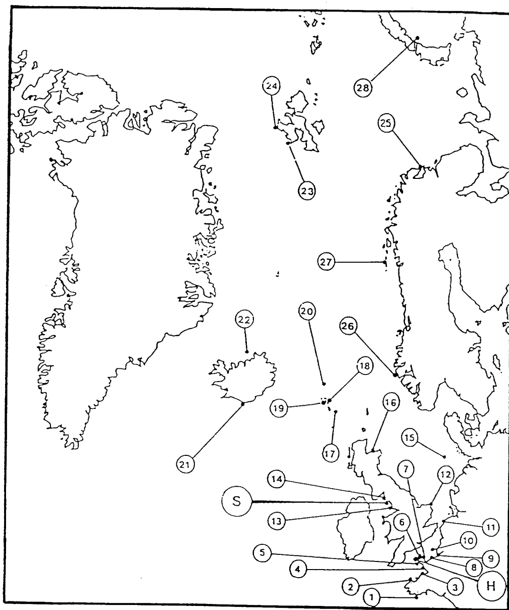
Figure 1.3. Locations of ^{129}\text{I} measurements made in seaweed and seawater by Raisbeck et al. (1995b). S and H indicate the reprocessing plants at Sellafield and Cap de la Hague, respectively. The ^{129}\text{I}/^{127}\text{I} data are presented in Table 1.4.
