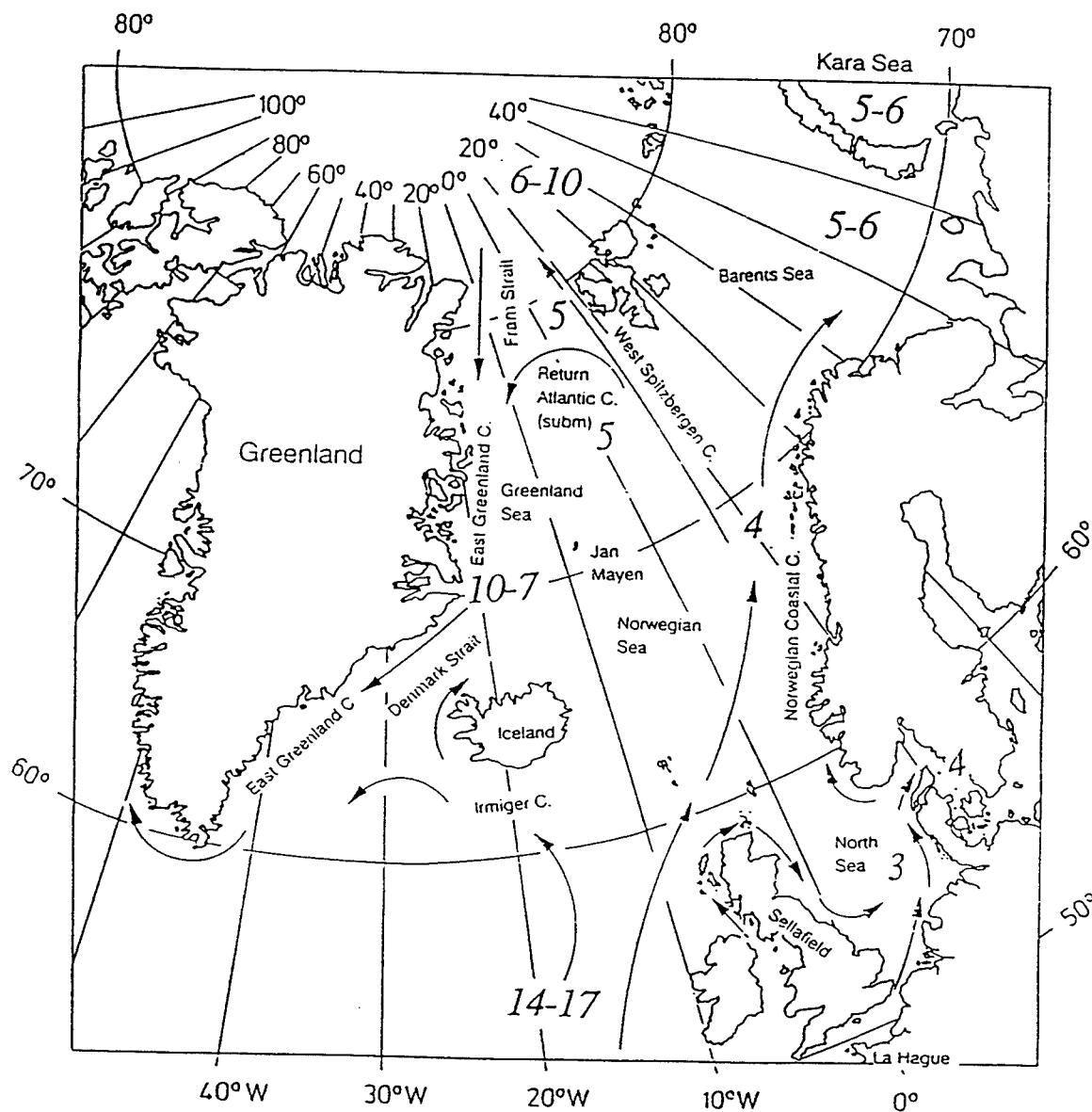
Figure 1.1. Circulation routes and transit times from Sellafield to various regions of the high latitude North Atlantic and Arctic Oceans. From Dahlgaard et al. (1995).
