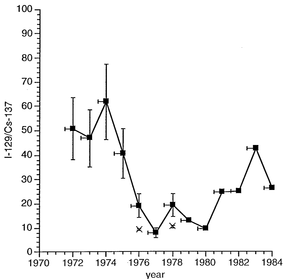
Figure 2.3. Predicted (squares) and measured (x) I-129/Cs-137 atom ratios on the northern coast of Scotland. Predicted values are simply the release ratio from Sellafield, with an estimated two years transit time to the north of Scotland. Actual transit times are probably somewhat shorter, as indicated by the x-error bars. Y error bars indicate the estimated uncertainty in Sellafield discharges prior to 1977 (Yiou et al., 1995).
