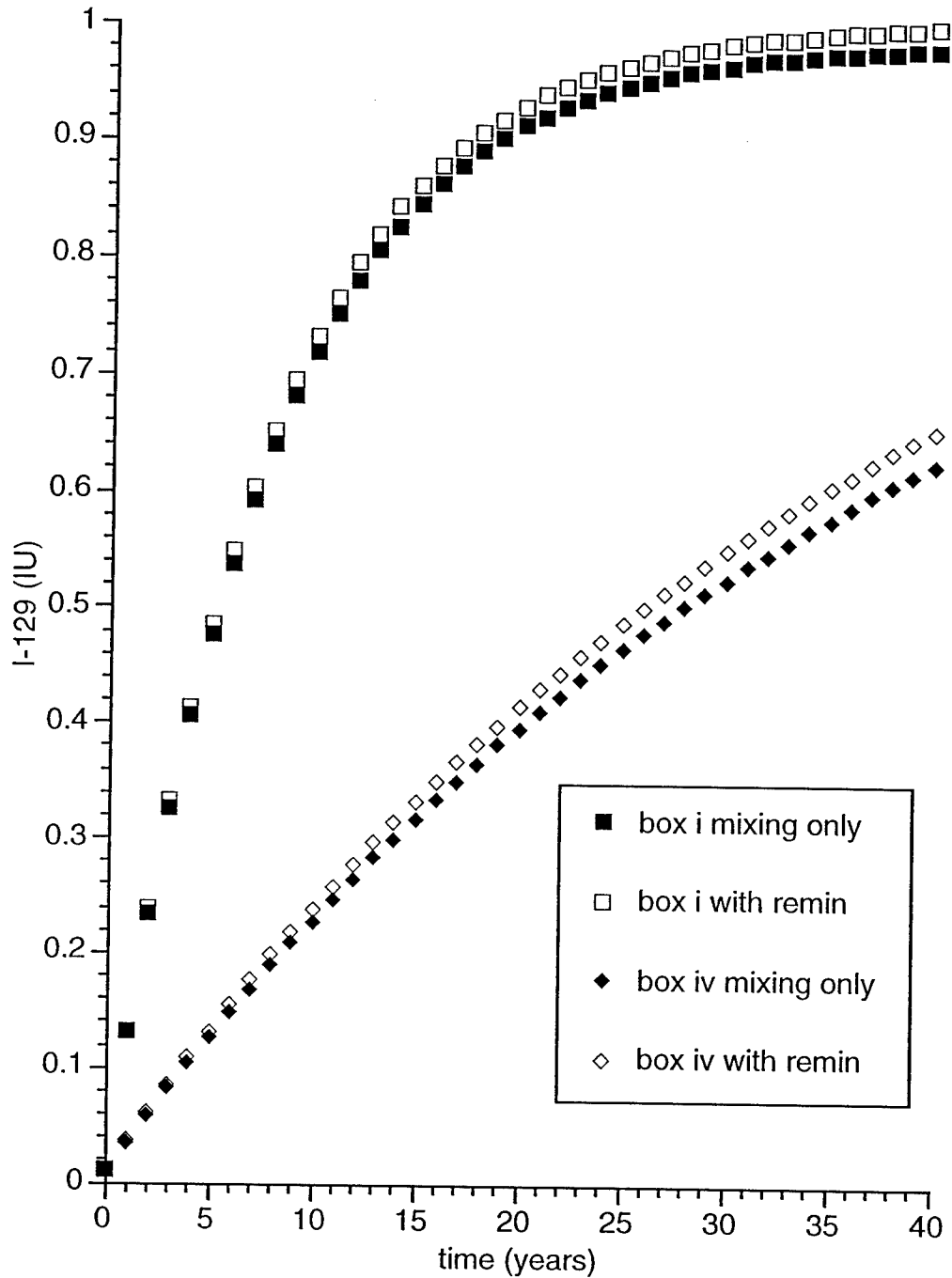
Figure 4.13. The evolution of I-129 concentrations in the ^{228}\text{Ra} -calibrated four box thermocline model of Sarmiento et al. (1990). Only boxes i ( \sigma_\theta = 26.5 ) and iv ( \sigma_\theta = 27.4 ) are shown. Closed symbols are mixing-only case, open symbols include particulate fluxes.
