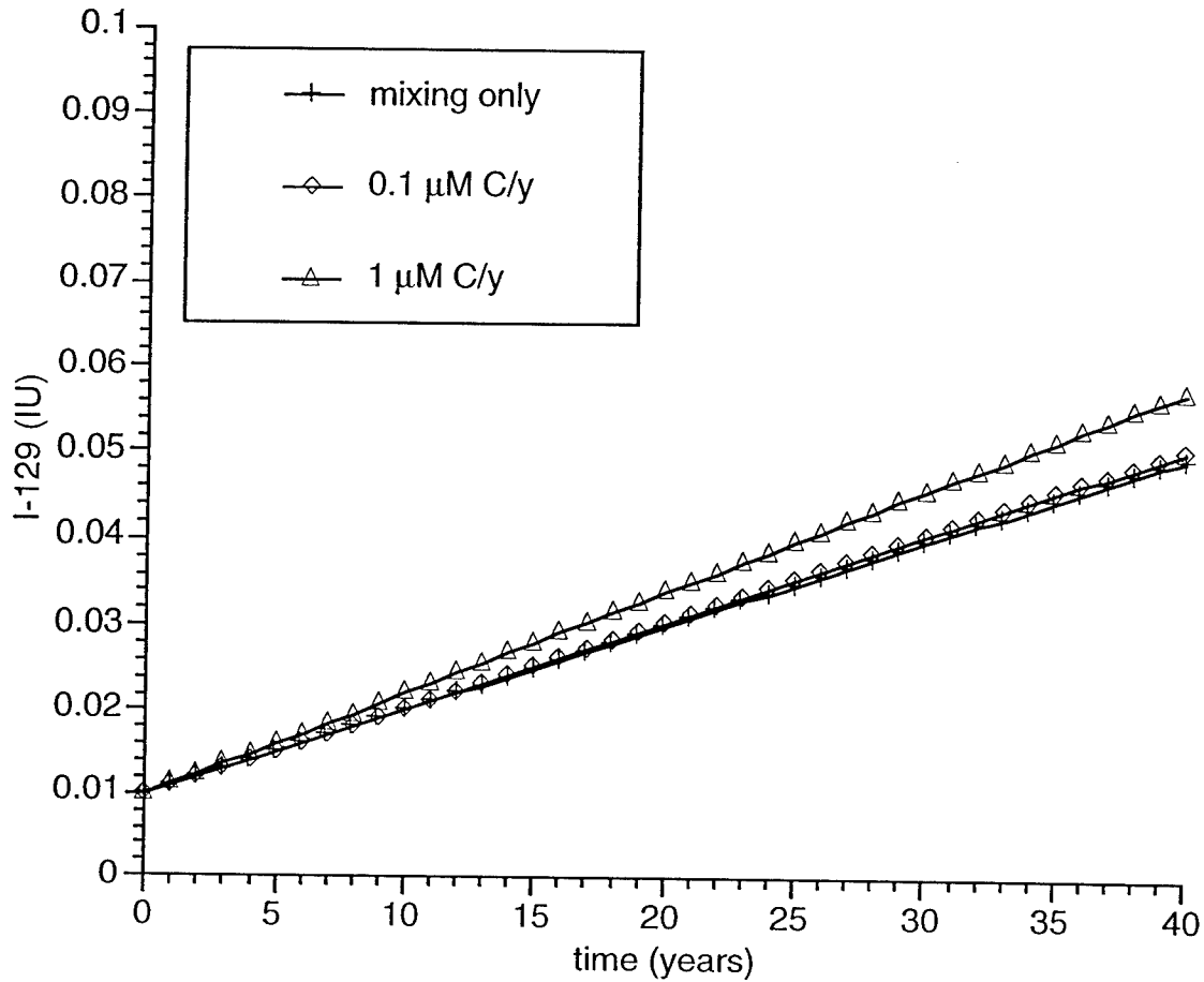
Figure 4.10. Evolution of deep water I-129 concentration in the two-box model depicted in Figure 4.9, for three cases: +, mixing only; ◇, with 0.1 μM C/year remineralization; and Δ, with 1 μM C/year remineralization.
