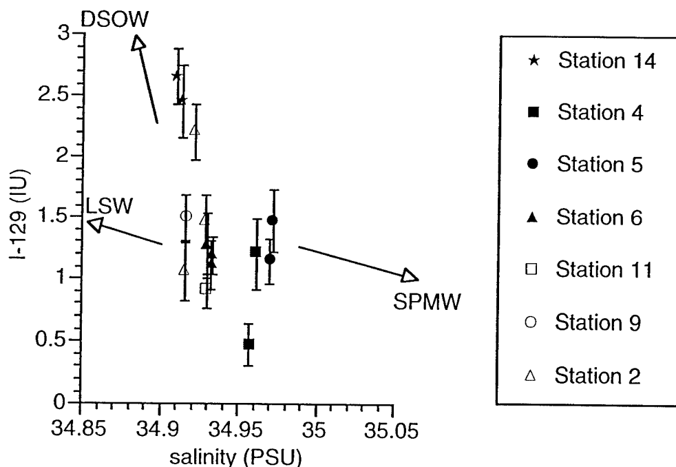
Figure 3.29. Iodine-129 versus salinity for Faroe Bank Channel overflow (Station 14), Iceland Scotland Overflow Water (Stations 4 and 5) and Northeast Atlantic Deep Water (Stations 6, 9, 11, and 2), illustrating a complex history of mixing with SPMW, LSW, and DSOW.
