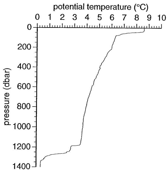
Figure 3.14.c. CTD temperature profile at Station 11.
