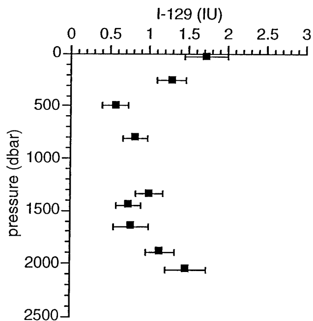
Figure 3.8.a. ^{129}\text{I} profile at Station 5, on the eastern flank of the Reykjanes Ridge.
