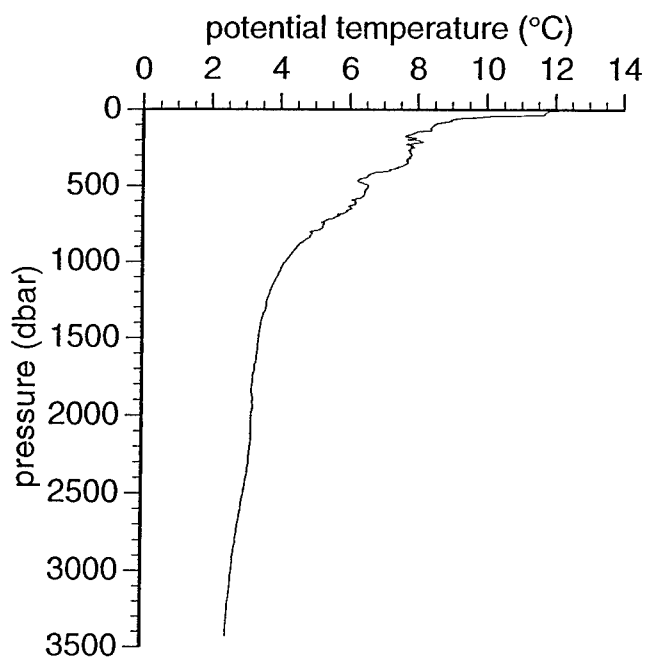
Figure 3.11.c. CTD temperature profile at Station 4.
