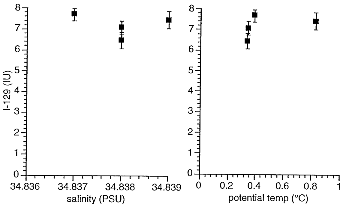
Figure 3.16. I-129 versus salinity and potential temperature in the Station 11 DSOW core.
