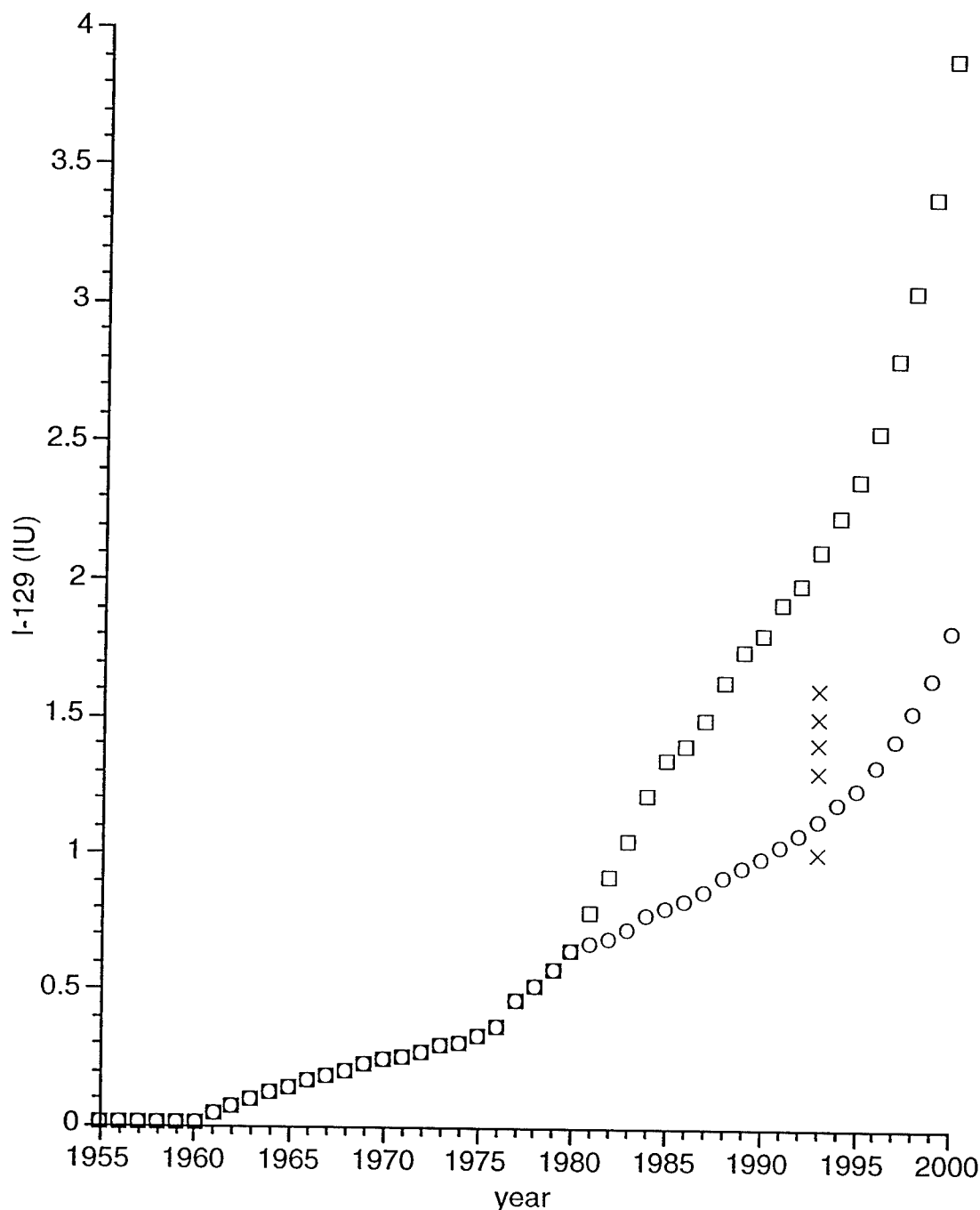
Figure 4.3. Modeled I-129 concentration in Greenland Sea Deep Water box, without remineralization terms. Squares, indicate GSDW I-129 resulting from a constant GSDW formation rate, while circles represent the results when GSDW is reduced by 80% beginning in 1980. X's are observed concentrations in 1993 (Zhou et al., submitted manuscript).
