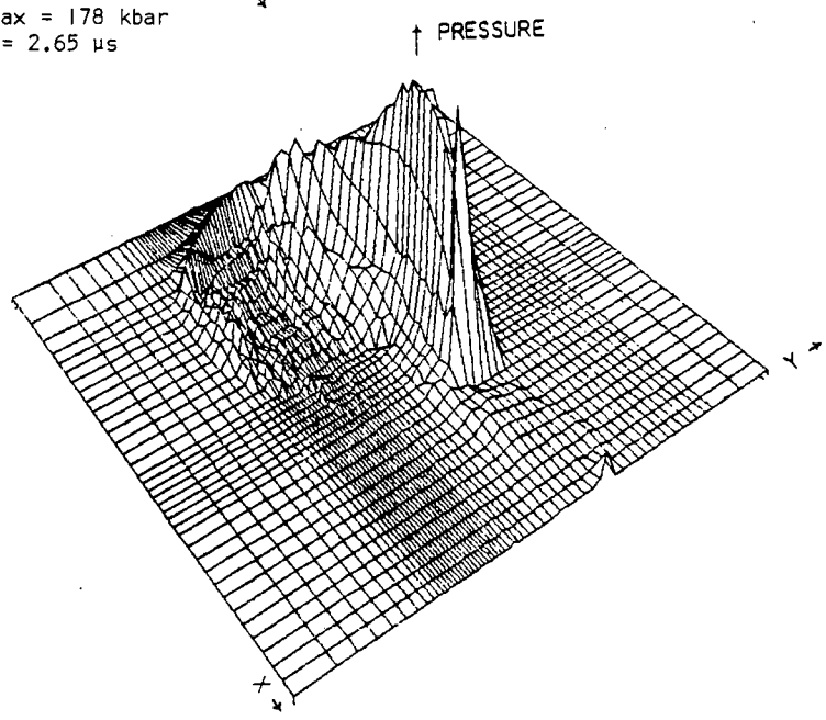
Figure 50. Density and Pressure Fields
