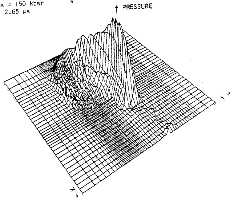
Figure 51. Density and Pressure Fields
