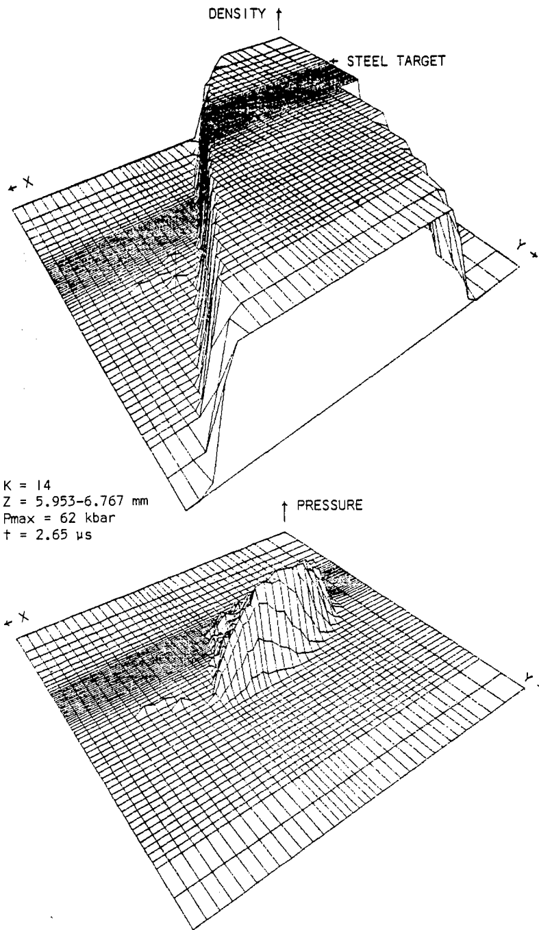
Figure 44. Density and Pressure Fields
