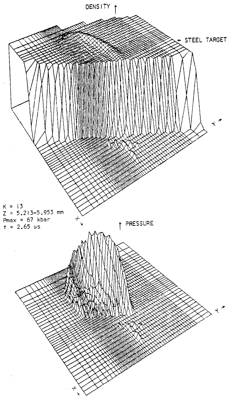
Figure 56. Density and Pressure Fields
