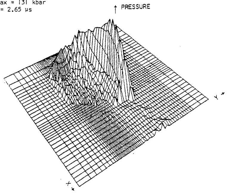
Figure 52. Density and Pressure Fields
