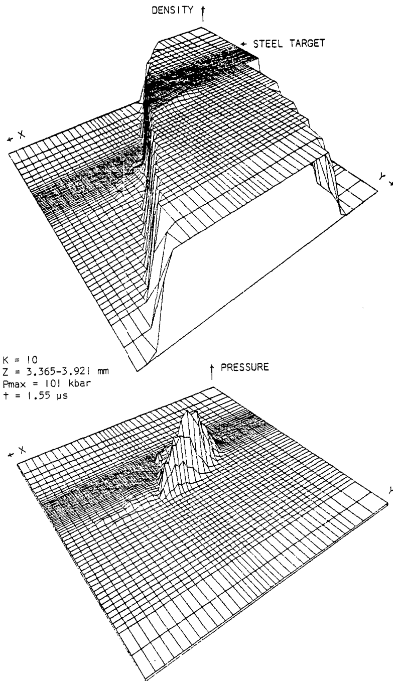
Figure 13. Density and Pressure Fields
