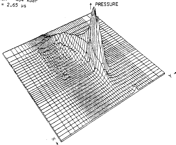
Figure 47. Density and Pressure Fields
