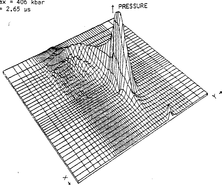
Figure 46. Density and Pressure Fields
