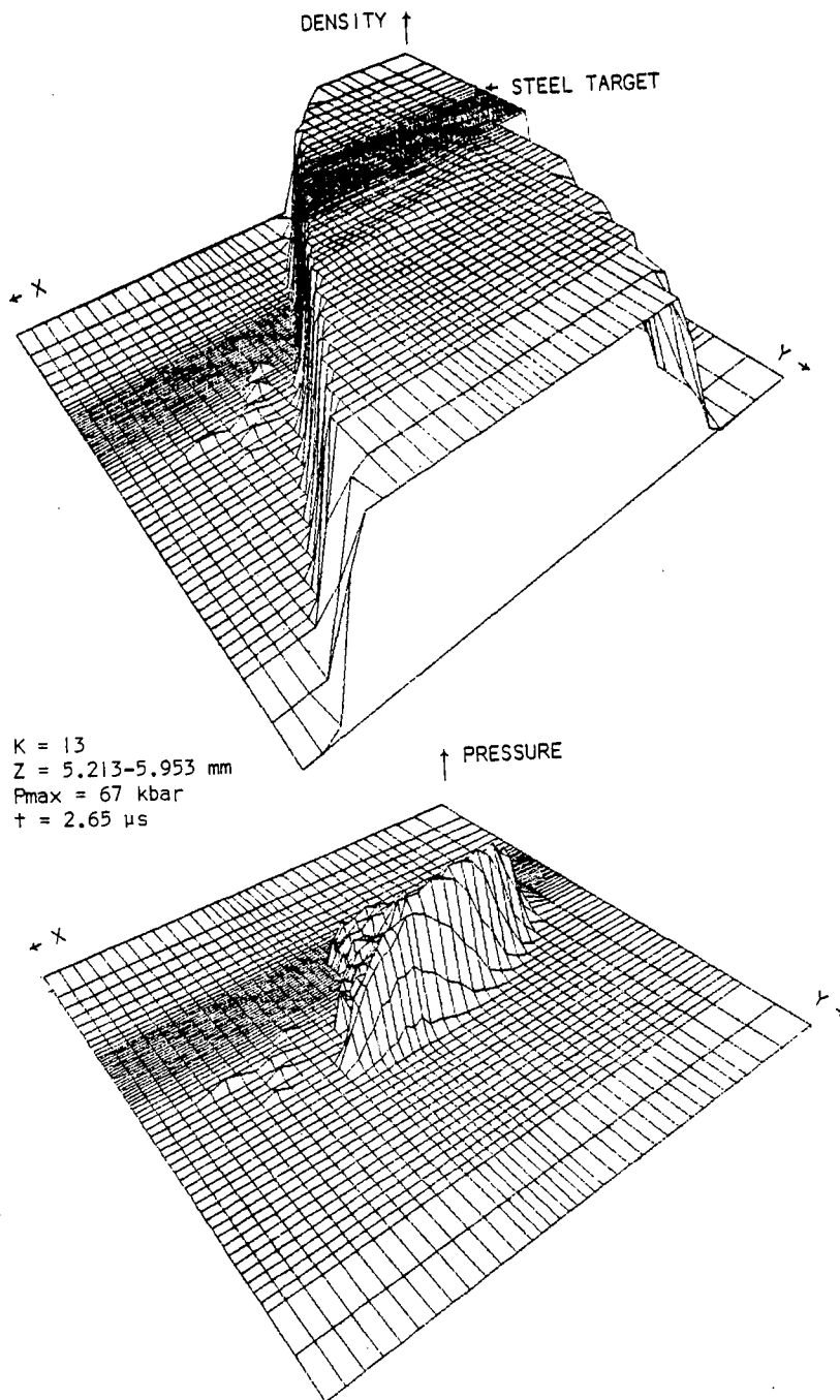
Figure 43. Density and Pressure Fields
