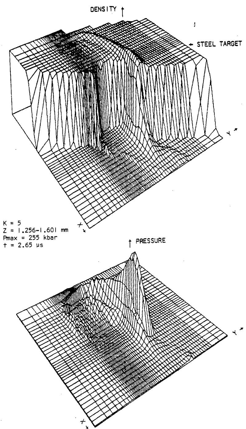
Figure 49. Density and Pressure Fields
