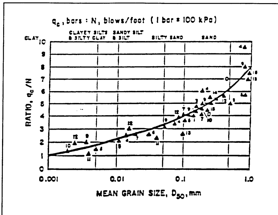
Figure 9. Relationship between q_c/N_{SPT} and medium grain size D_{50} numbers next to data points indicate various sources of data (Robertson et al. 1983)
