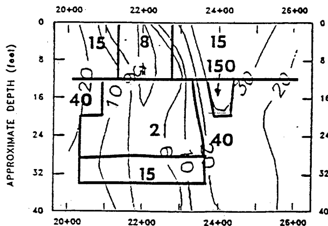
FIGURE 3. DIPOLE-DIPOLE RESISTIVITY PROFILE.
