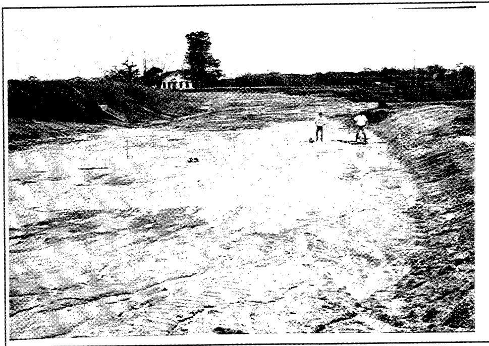
Figure 2. Site of spread footing settlement prediction experiment and full-scale tied-back wall at TAMU sand sub-site
