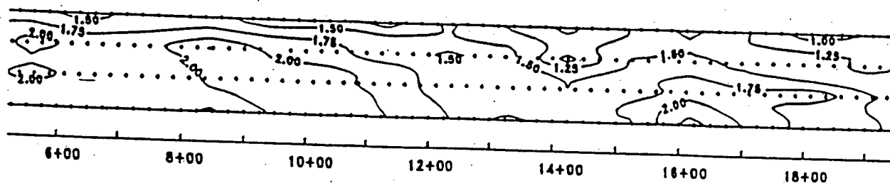
RESISTIVITY RATIO PSEUDOSECTION (HP/LP) (Contour Interval = 0.25)
