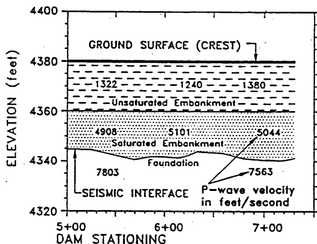
FIGURE 1. P-WAVE REFRACTION PROFILE.
