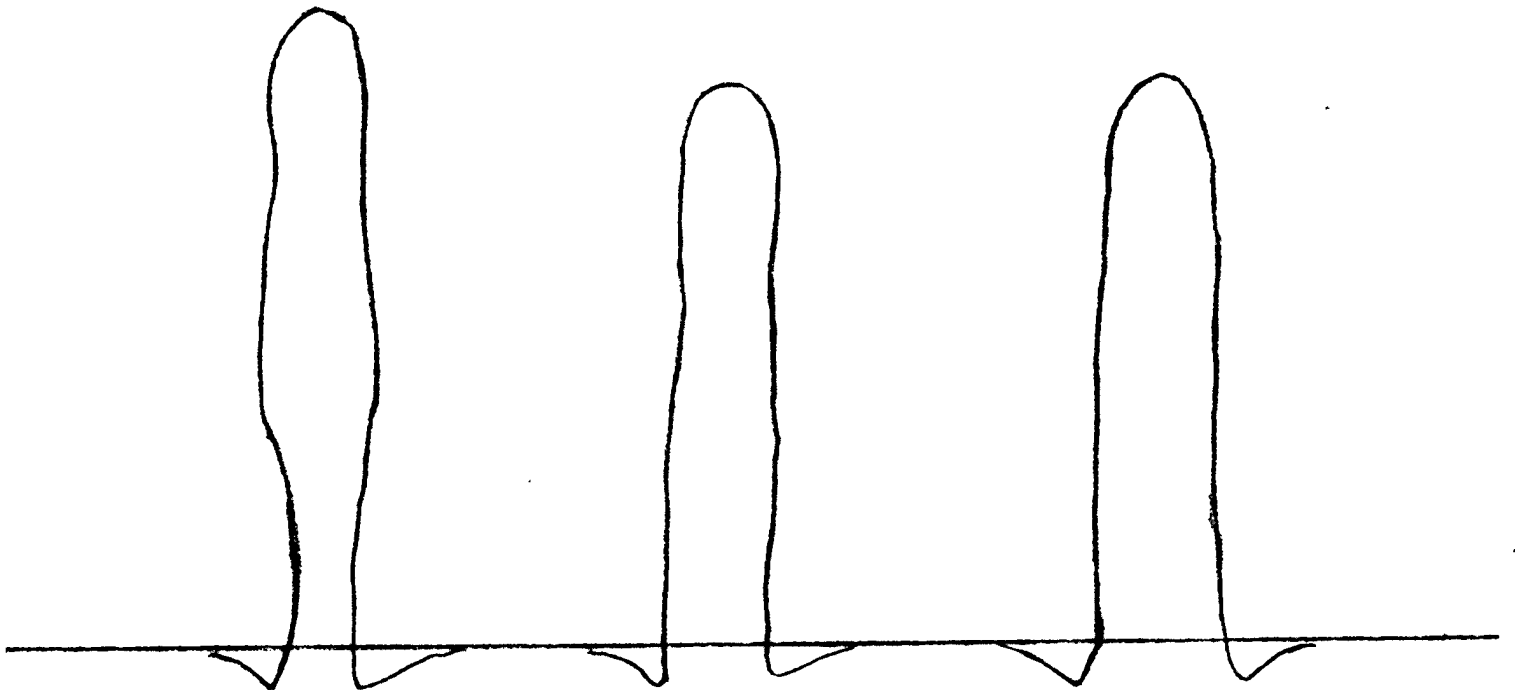
Figure 7. WHA Nose-Shape Projectile Semi-Infinite Penetration Channels.
