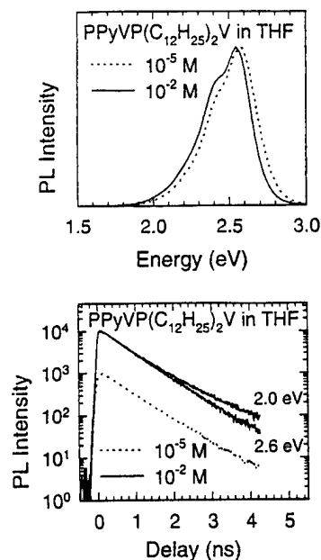
FIG. 4. PL spectrum (upper) and PL decays (lower) of 10^{-5} M (dotted lines) and 10^{-2} M (solid lines) PPyVPV(C 12 H 25 ) 2 V in THF. For the concentrated solution, PL decays are shown for 2.0 and 2.6 eV emission. Dilute solution PL decay is for 2.6 eV emission.
