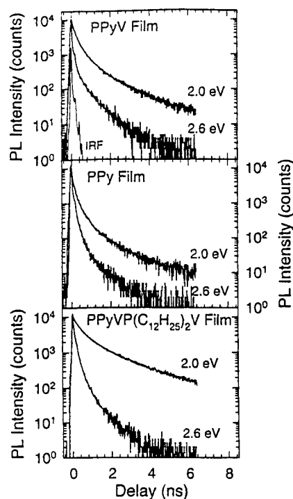
FIG. 10. PL decays of PPyV (upper), PPy (middle), and PPyVPV (lower) films excited at 2.8 eV. Decays are shown for 2.0 and 2.6 eV emission, as indicated. Instrument response (IRF) is shown in the upper portion of the figure.
