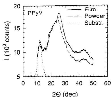
FIG. 13. X-ray-diffraction spectrum of PPyV powder (dashed) and film (solid). Dotted line represents background due to off-axis Si substrate. X-ray wavelength is 0.154 nm ( \text{Cu } K\alpha ).
