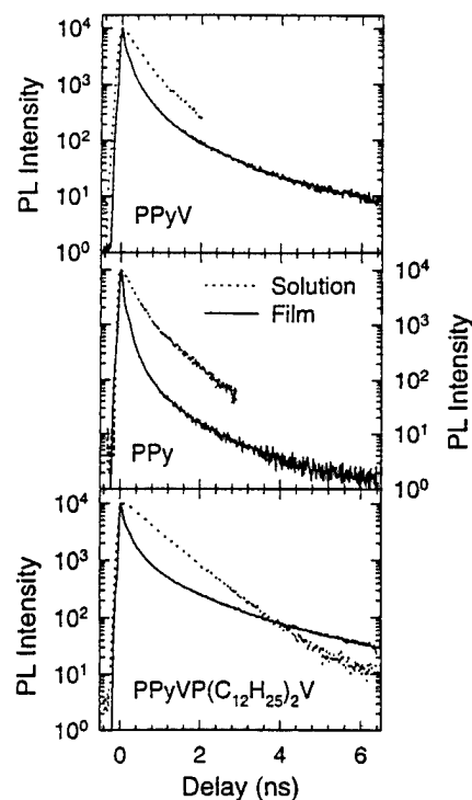
FIG. 11. Energy-integrated PL decays for PPyV (upper), PPy (middle), and PPyVPV (lower) films (solid lines) excited at 2.8 eV. Solution decays (at PL maximum) are shown for comparison (dotted lines).
