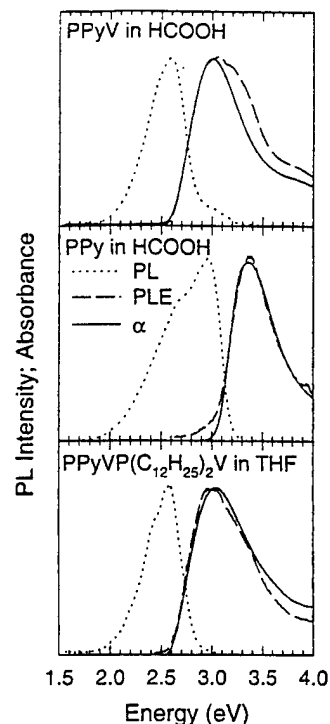
FIG. 2. Absorption (solid), photoluminescence (PL, dotted) and PL excitation (PLE, dashed) spectra for dilute solutions ( < 10^{-5} M) of PPyV in HCOOH (upper), PPy in HCOOH (middle), and PPyVPV in THF (lower).
