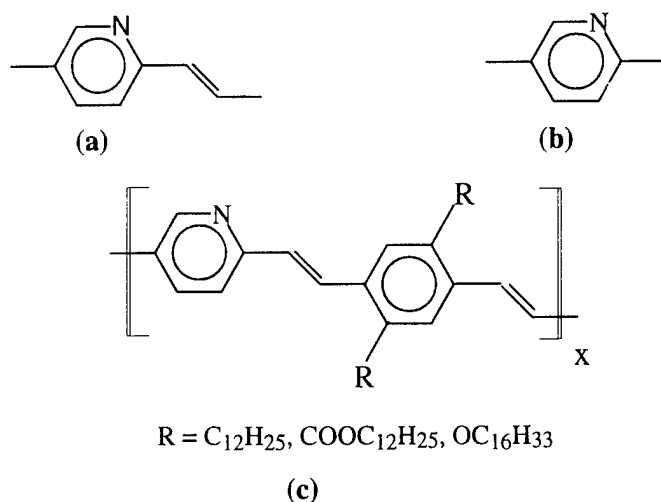
Fig. 1 Schematic structure of (a) poly( p -pyridyl vinylene) (PPyV), (b) poly( p -pyridine), and (c) copolymers of PPyV and PPV derivatives.
