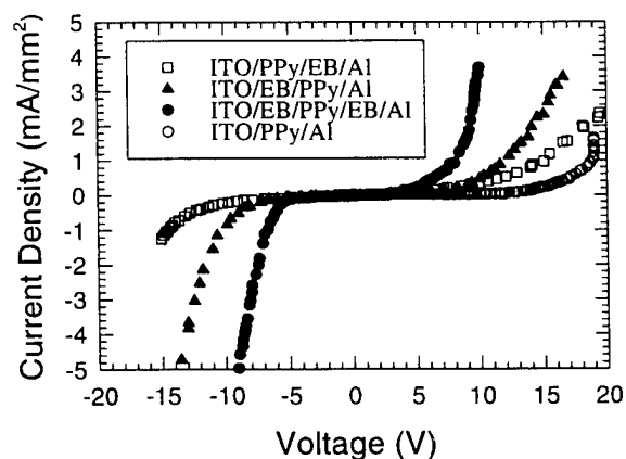
Fig. 5 I-V characteristics of four devices with different structures as shown in the figure. Note that the turn on voltage decreases as the total number of layers increases (From Ref. 20b).
