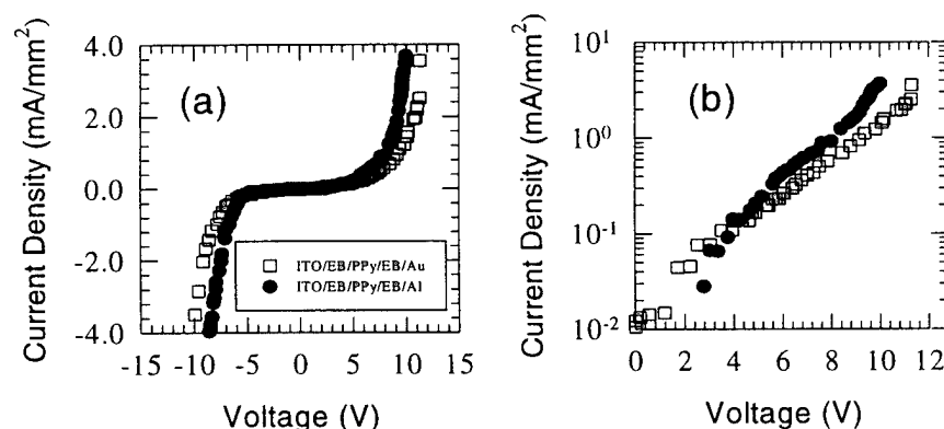
Fig. 6 I-V characteristics of ITO/EB/PPy/EB/Al and ITO/EB/PPy/EB/Au devices plotted in (a) linear scale in forward and reverse bias and (b) semi-log scale in forward bias.
