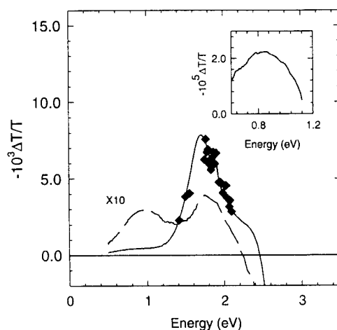
Fig. 4: The millisecond photoinduced absorption spectra of powders (—) and films (---) of PPyV at 80 K using a pump beam energy of 2.71 eV. The spectral response of the 1.9 eV ps PA at 1 ns time delay (◆) is also plotted. The inset shows the quadrature signal for powder samples.
