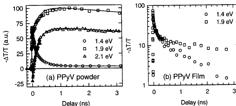
Fig. 3: (a) Decay of PA at 1.4 eV (○), 1.9 eV (□) and 2.1 eV (△) for PPyV powder. (b) Decay of PA at 1.4 eV (○) and 1.9 eV (□) for a PPyV film cast from HCOOH solution (Ref. 11).
