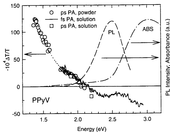
Fig. 2: The ps PA at 0 ps for powder (○) and \sim 10^{-2} M solution in HCOOH (□ and —). The PL (---) and absorption (— · —) spectra are shown for comparison (from Ref. 10).
