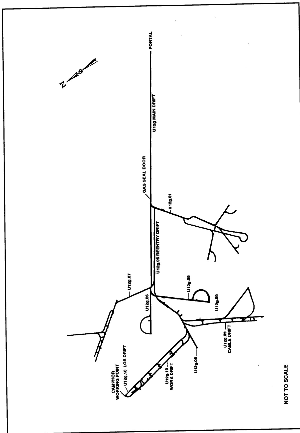
Figure 7-1. CAMPHOR event - tunnel layout.
