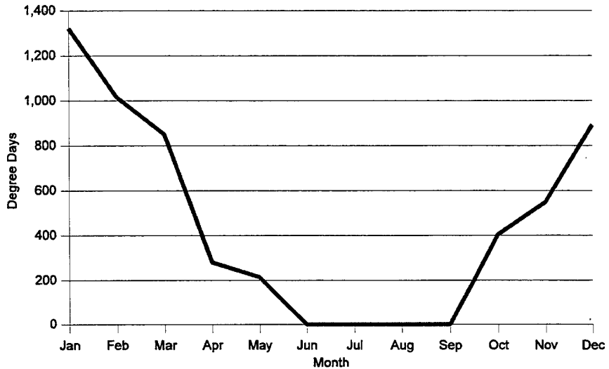
Figure 2.5.6.2, Heating Degree Days
