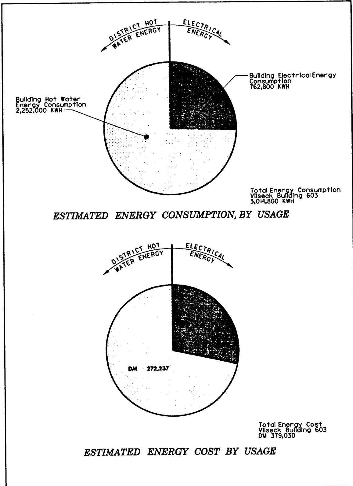
Figure ESF-2 Annual Energy Use - Vilseck Building 603
