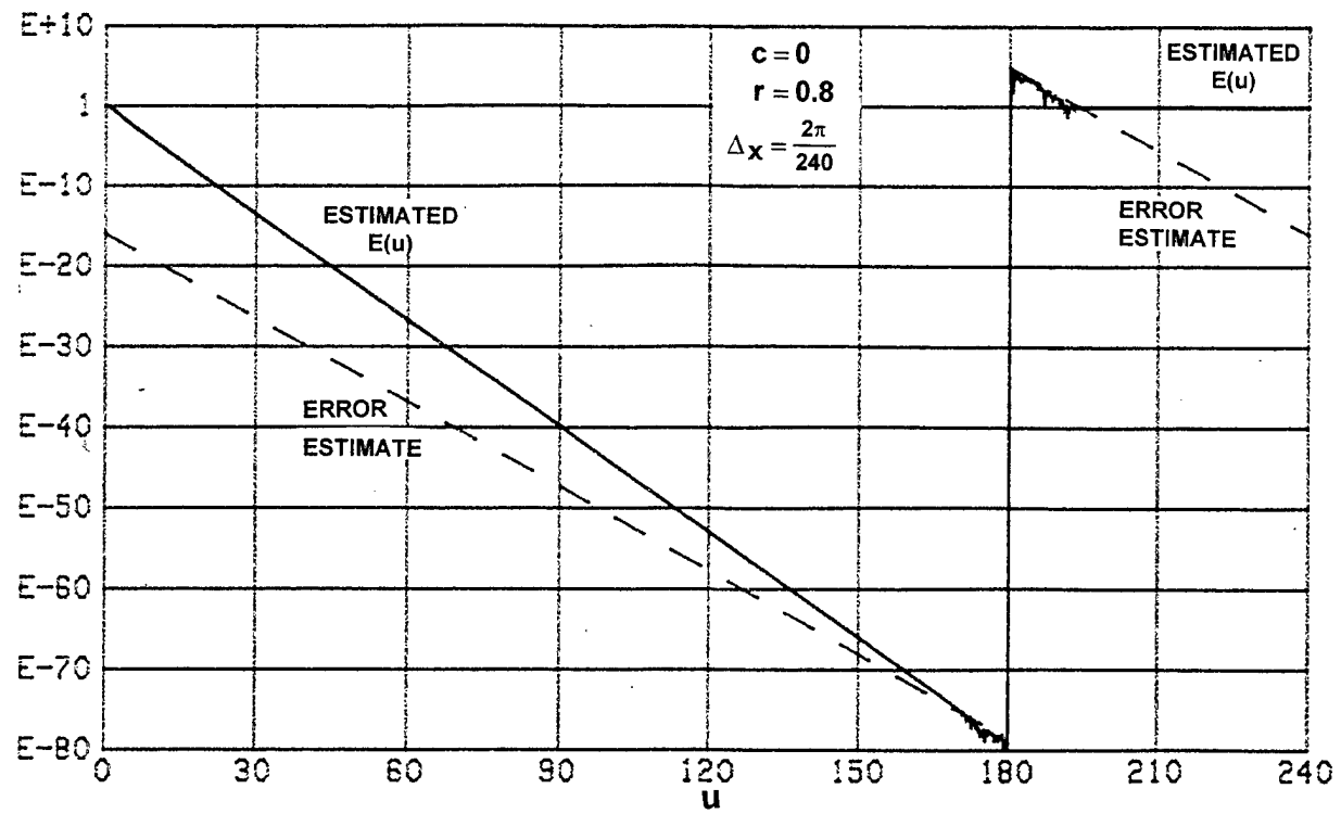
Figure 15. Branch Point E(u)
