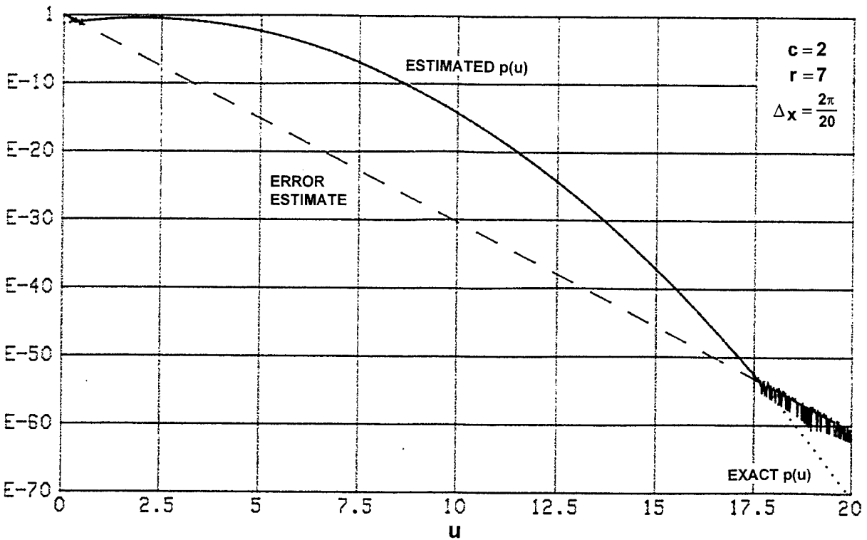
Figure 5. Gaussian p(u)
