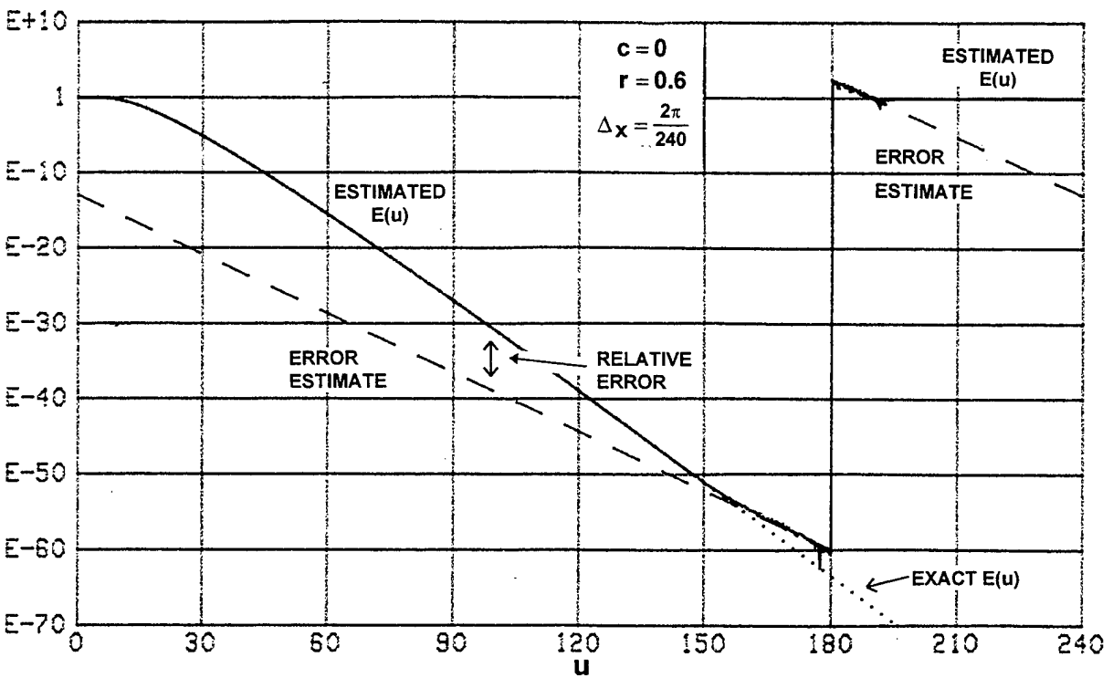
Figure 11. Chi-Square E(u)
