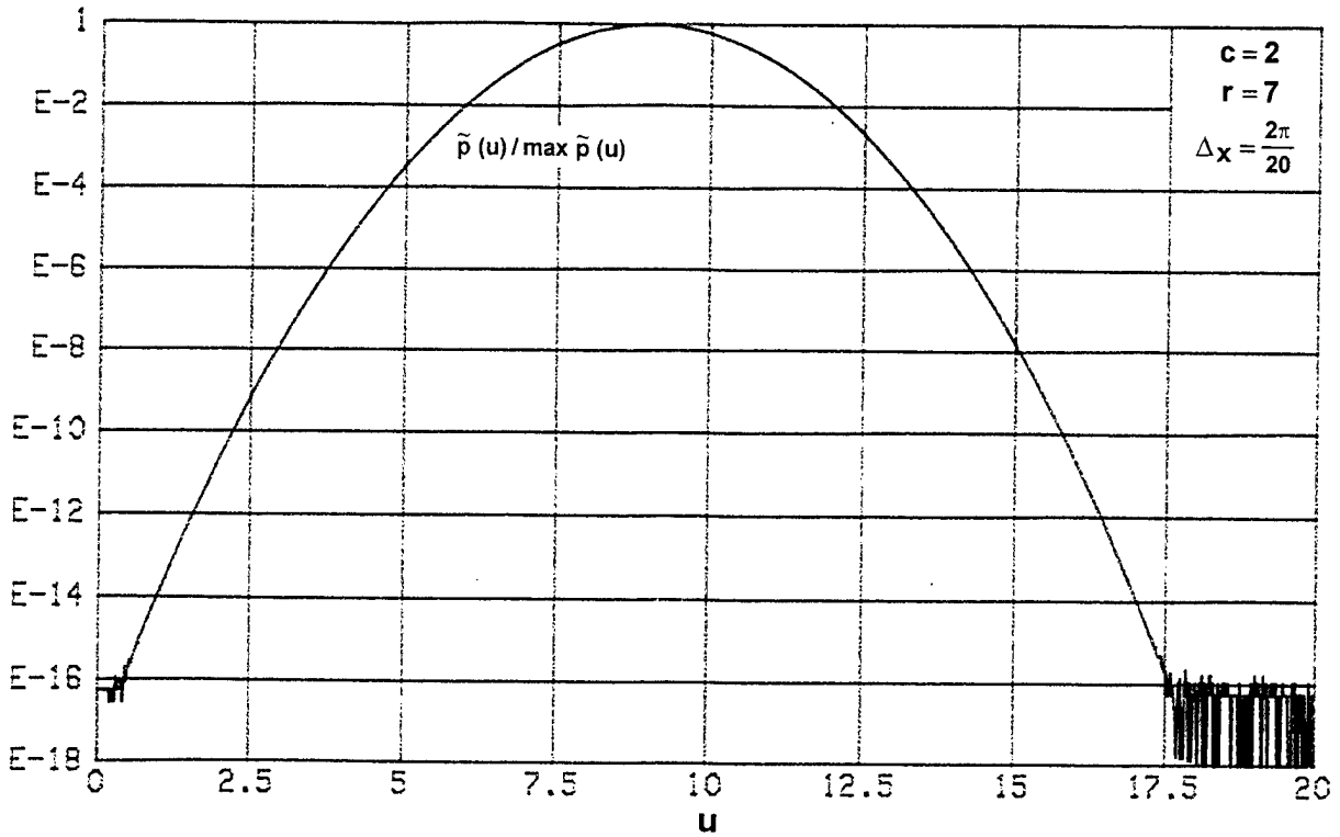
Figure 4. Gaussian \tilde{p}(u)
