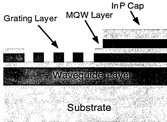
Fig. 4b. New device structure
