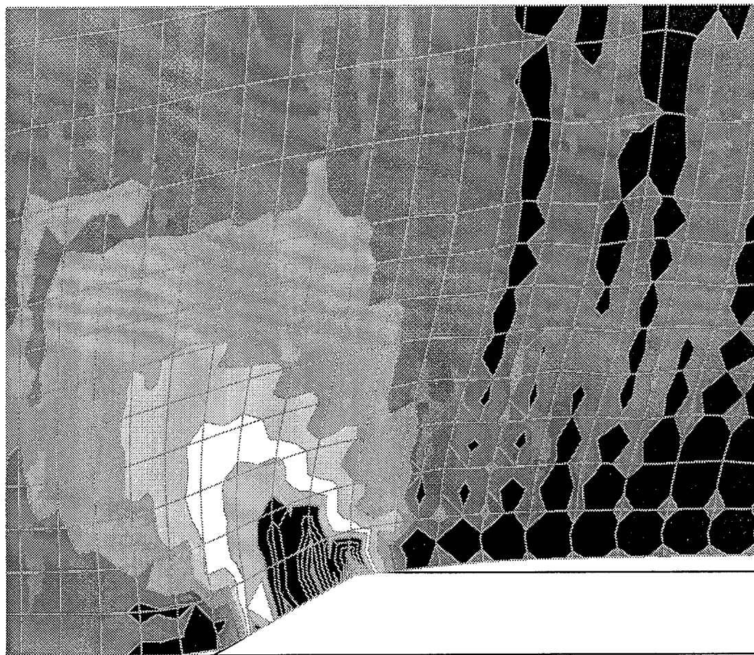
(a) Minimum principal stress SP1 distribution near plow tip. Figure 5-4. Principal stress components in soil at 10 fps steady-state plow velocity.
