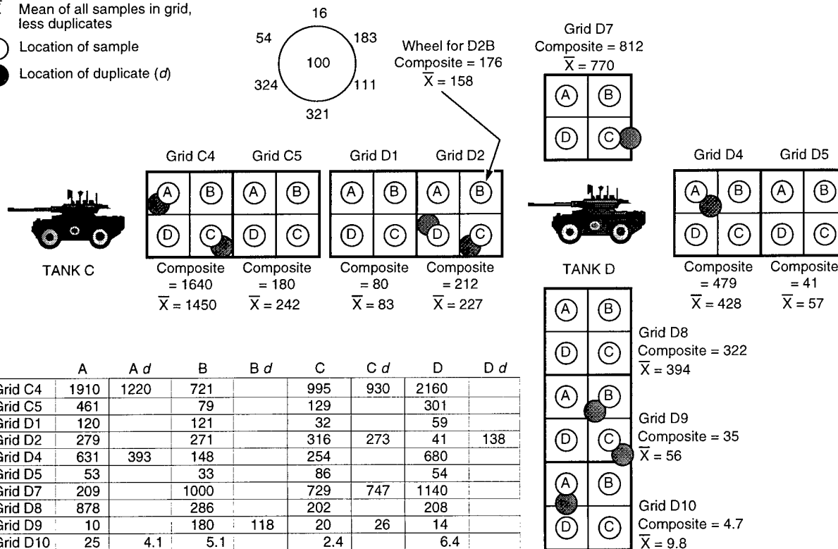
Figure 4. Sampling area at CFB-Valcartier firing range site, showing HMX concentrations from on-site measurements.
