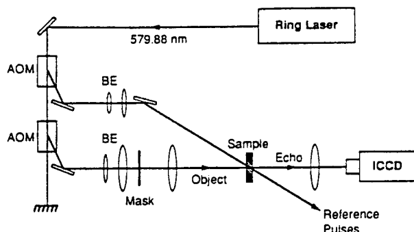
Fig. 2. Experimental setup for time-domain holographic image storage. AOM's, acousto-optic modulators; ICCD, intensified CCD camera; BE's, beam expanders.
