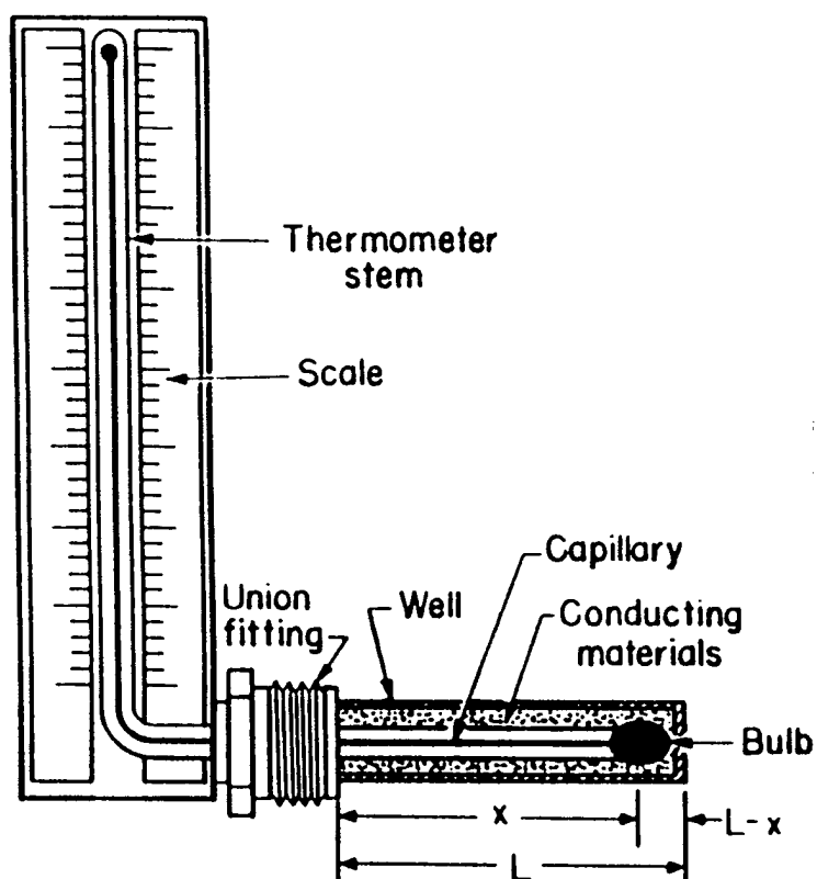
Industrial thermometer
