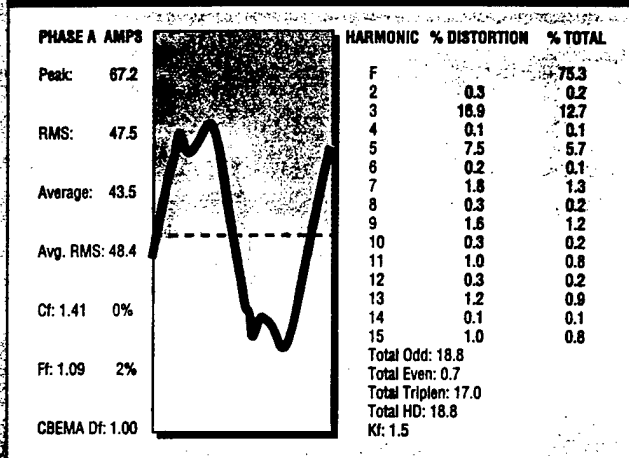
FIGURE 1 - HARMONIC CURVE VALUES (ELECTRONIC BALLASTS)
