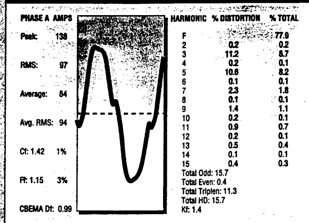
FIGURE 2 - HARMONIC CURVE VALUES (MAGNETIC BALLASTS)
