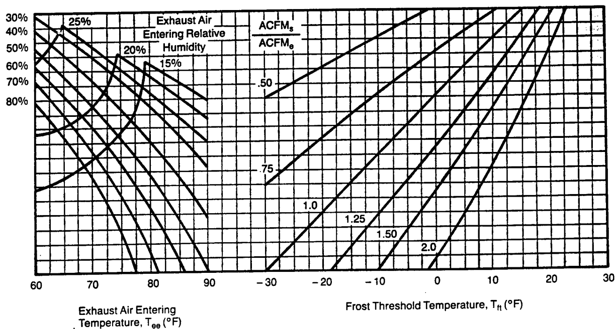
FIGURE 11 — TRU-125 FROST THRESHOLD TEMPERATURE (ANY ROWS)
