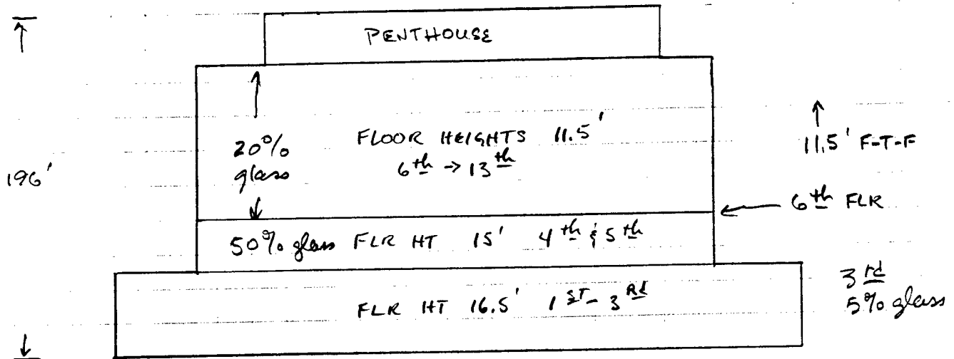
NORTH ELEVATION
