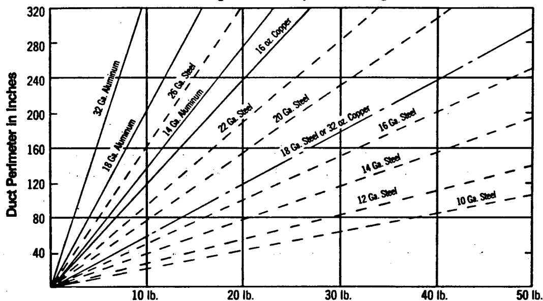
Duct Weight in Pounds per L.F., Straight Runs
