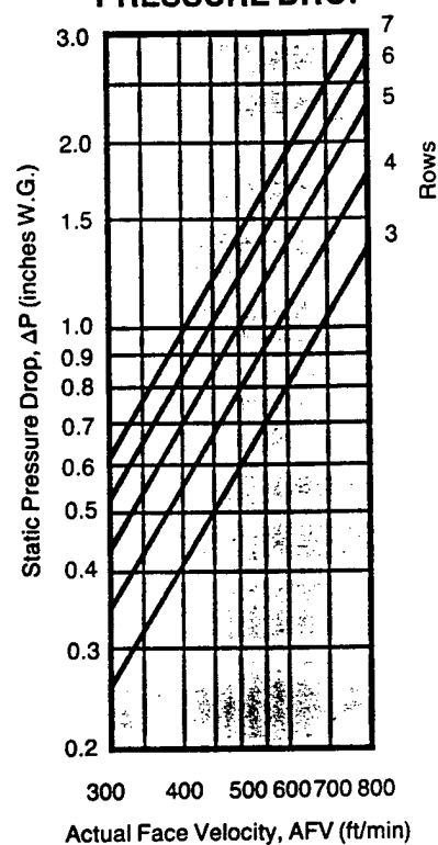
FIGURE 10 — TRU-125 PRESSURE DROP
