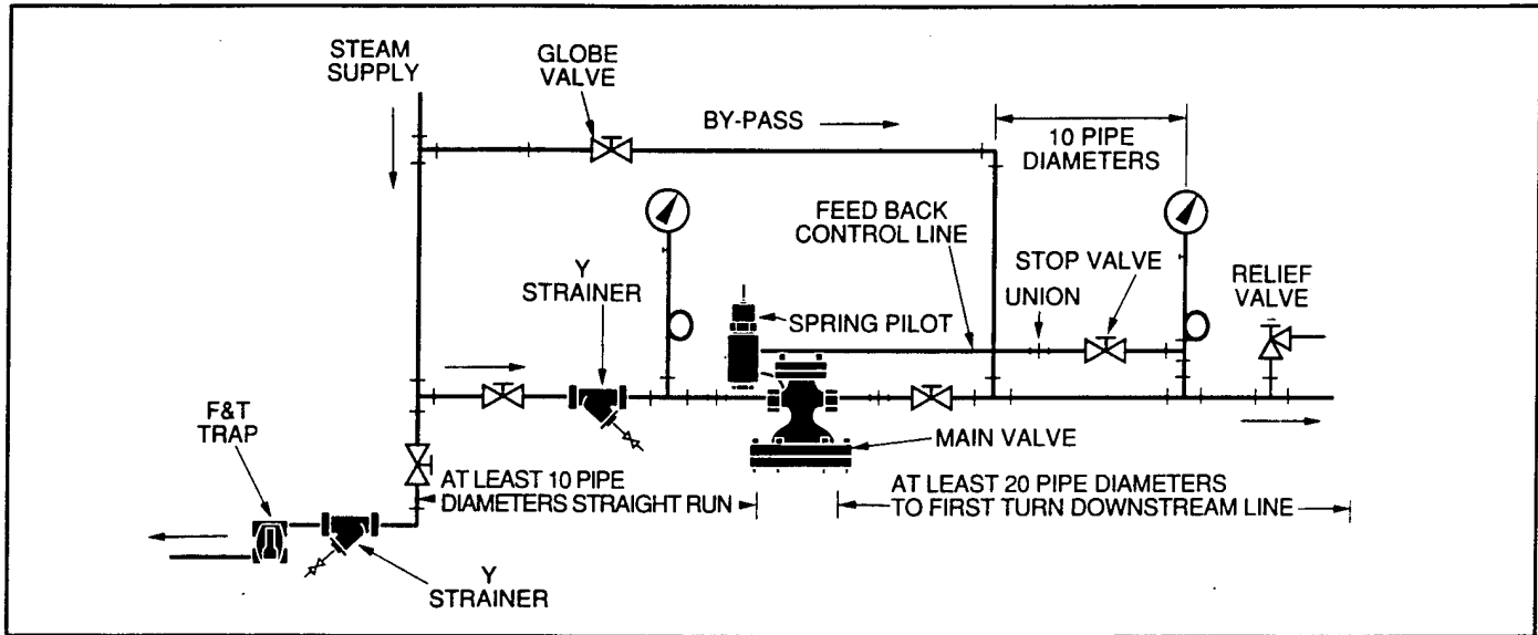
Series 2000 Pressure Regulator
