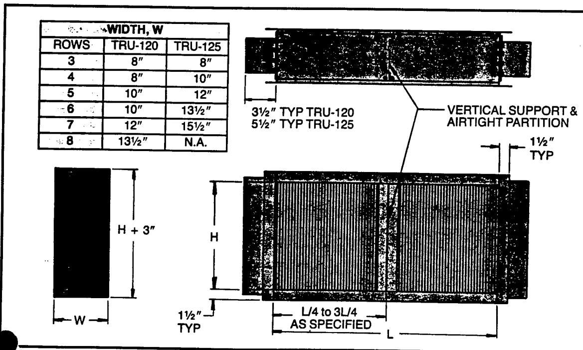
FIGURE 4 — TRU DIMENSIONS
