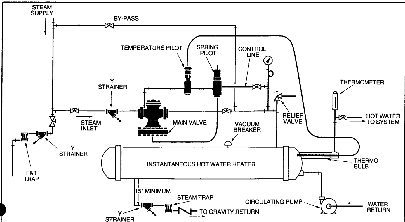
Series 2000 Temperature or Temperature/Pressure Regulator
