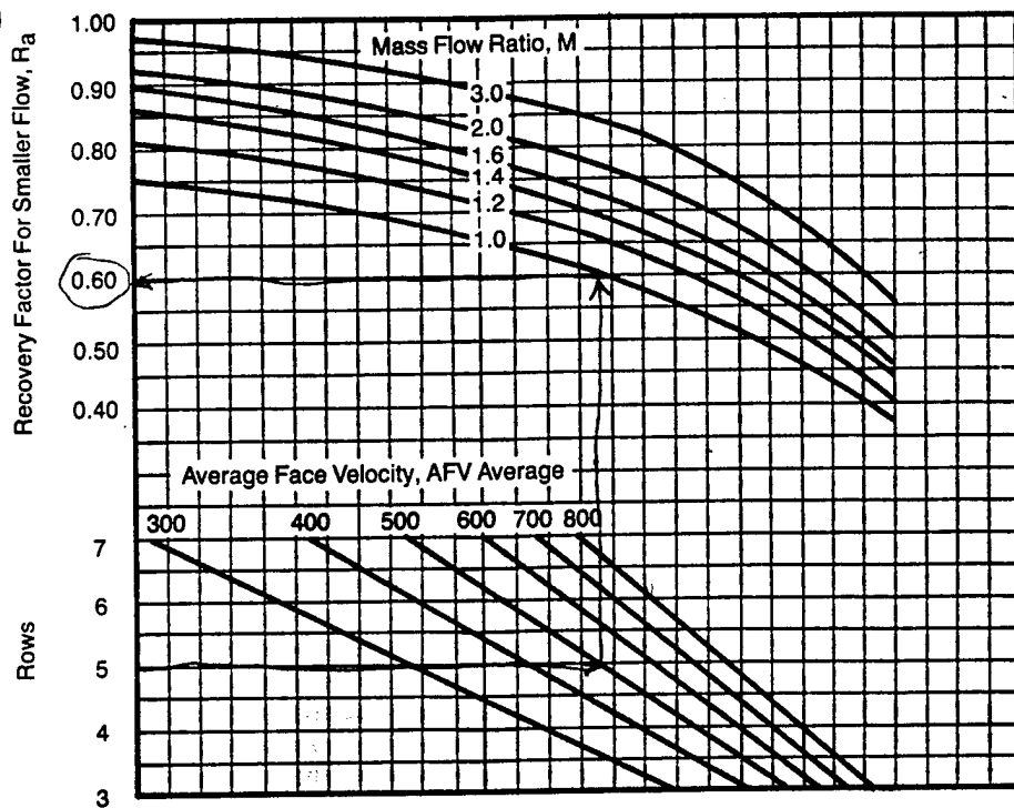
FIGURE 9 — TRU-125 RECOVERY PERFORMANCE
