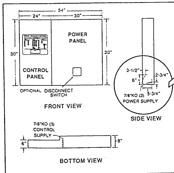
CONTROL PANEL
