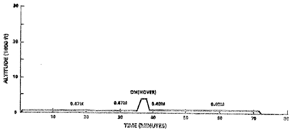
FIGURE 108. Type A V/STOL marine assault mission profile
