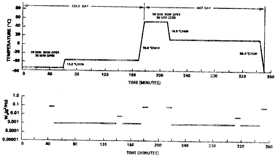
FIGURE 122. Type B V/STOL combat air patrol environmental profile
