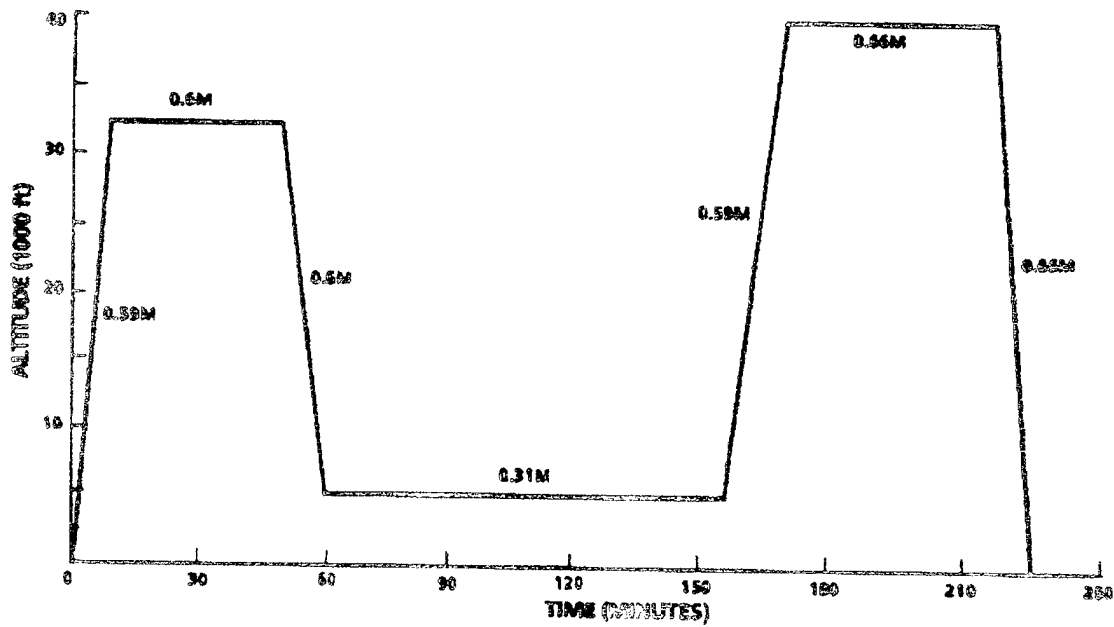
FIGURE 110. Type a V/STOL tanker mission profile
