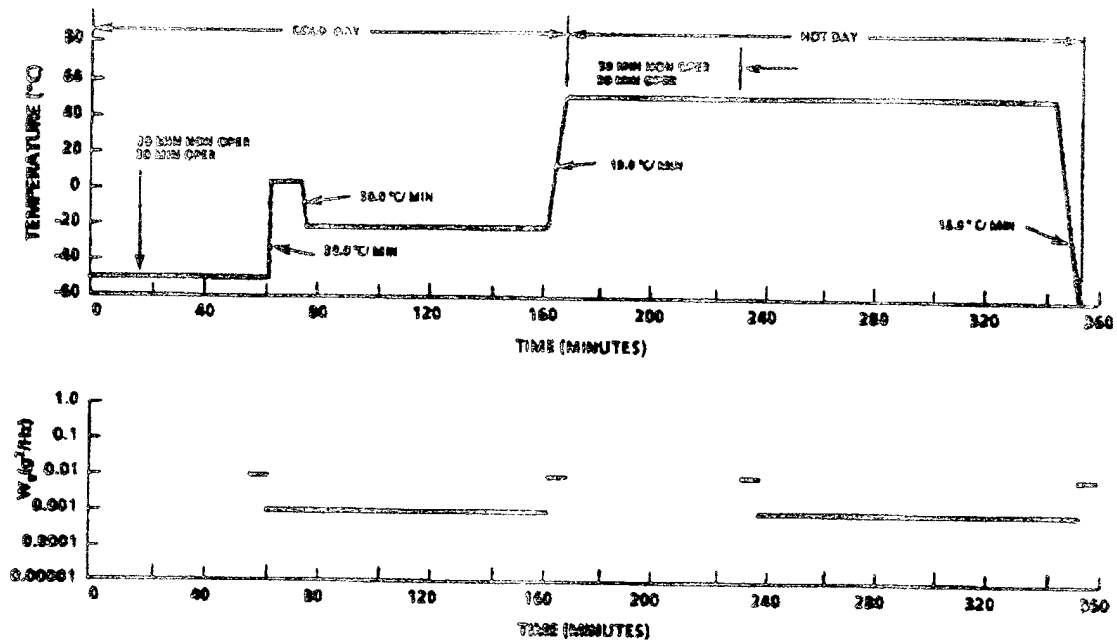
FIGURE 117. Type A V/STOL contact investigation environmental profile
