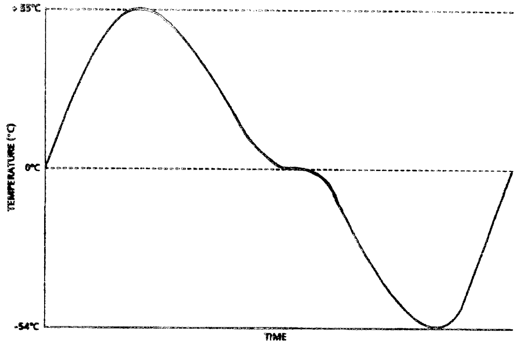
FIGURE 4. Typical thermal stress cycle
