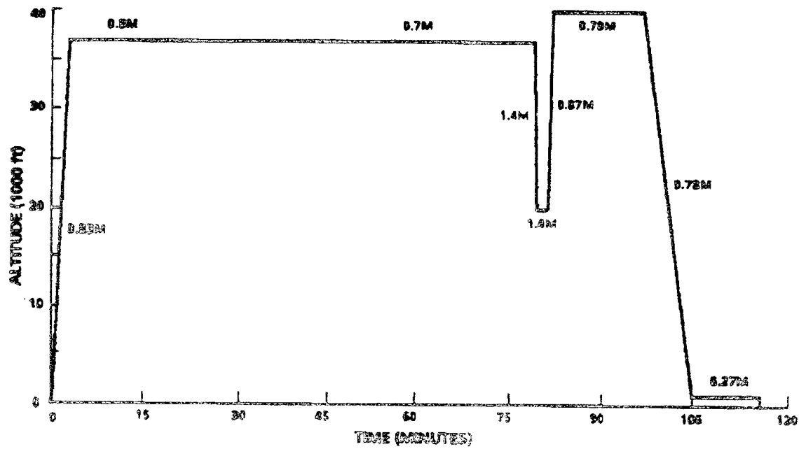
FIGURE 112. Type B V/STOL combat air patrol mission profile
