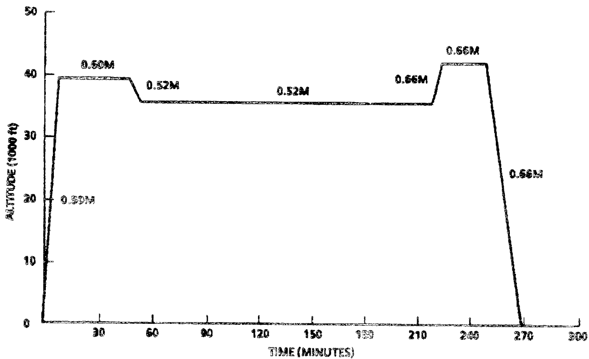
FIGURE 106. Type A V/STOL anti-submarine warfare mission profile
