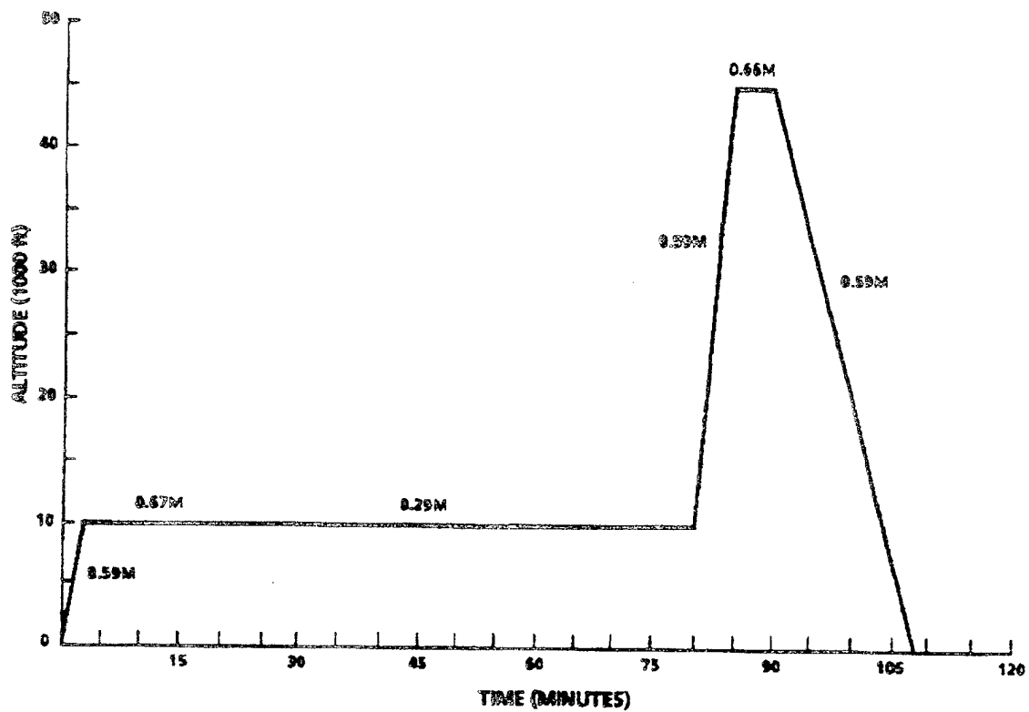
FIGURE 107. Type A V/STOL contact investigation mission profile
