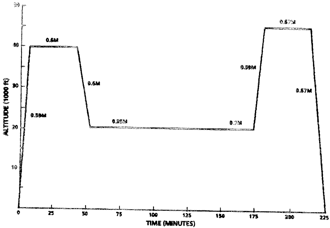
FIGURE 109. Type A V/STOL surface attack mission profile
