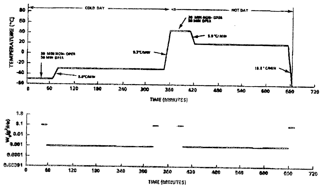
FIGURE 116. Type A V/STOL anti-submarine warfare environmental profile
