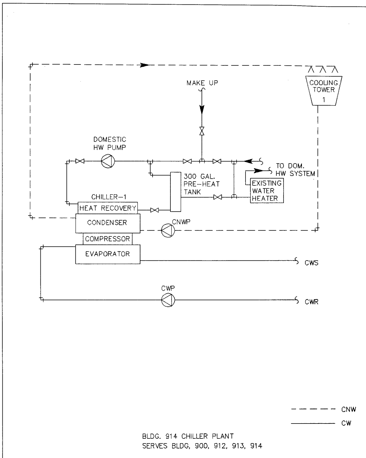
FIGURE 2-5. SCHEMATIC OF CHILLERS, CENTRAL PLANT 914
