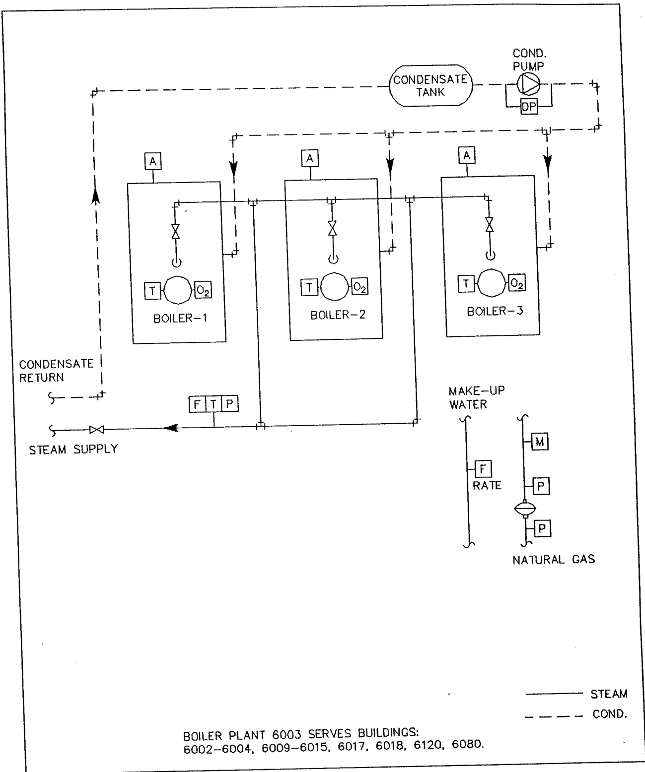
FIGURE 8-5. CONTROL SCHEMATIC OF BOILERS, CENTRAL PLANT 6003
