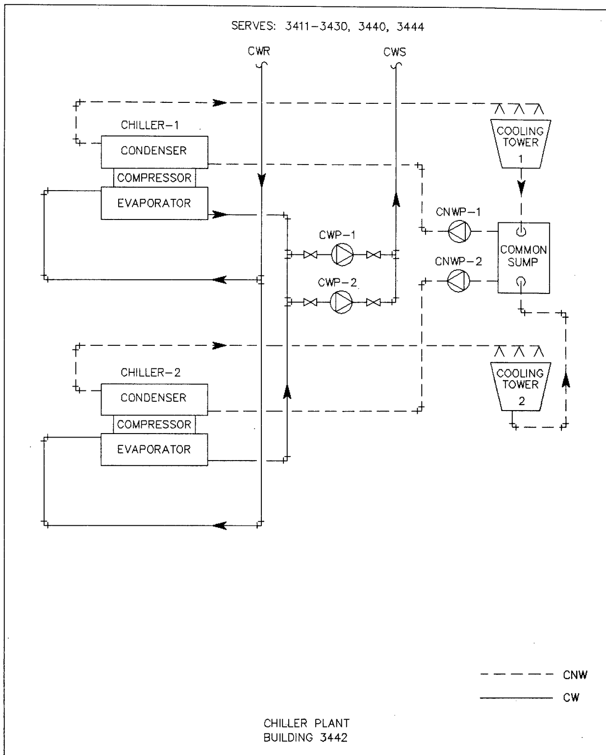
FIGURE 2-9. SCHEMATIC OF CHILLERS, CENTRAL PLANT 3442
