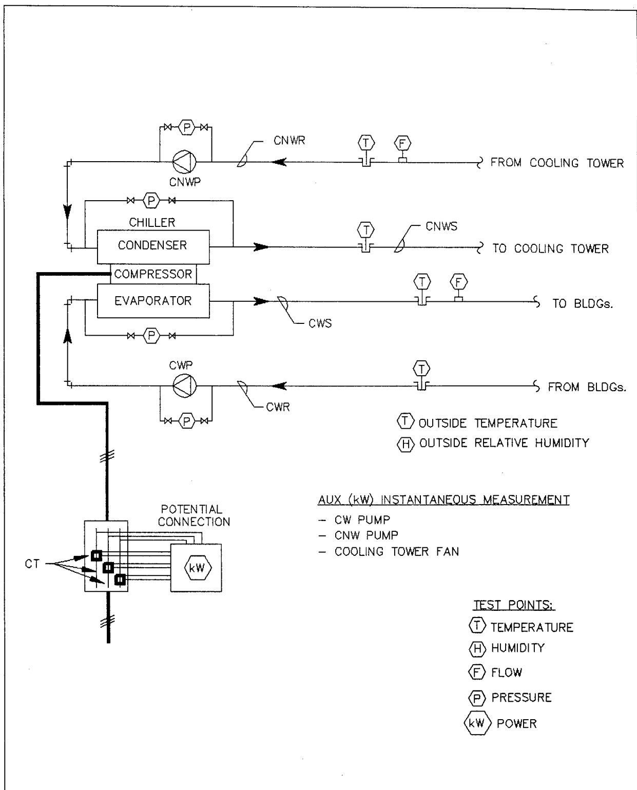
FIGURE 2-1. CHILLER TESTING
