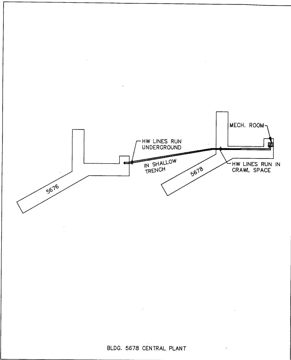
FIGURE 8-8. DISTRIBUTION PLAN, CENTRAL PLANT 5678
