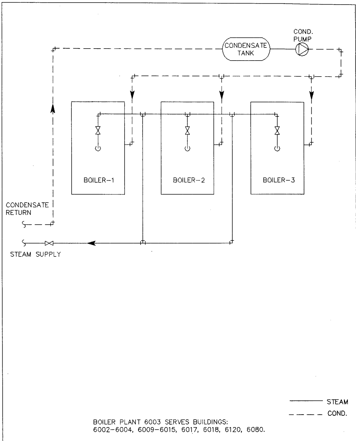
FIGURE 2-19. SCHEMATIC OF BOILERS, CENTRAL PLANT 6003
