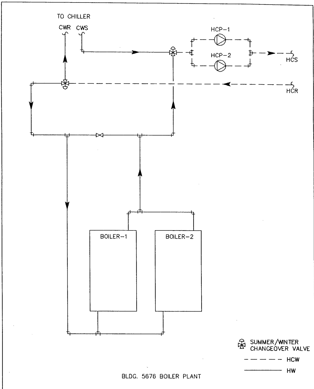
FIGURE 2-13. SCHEMATIC OF BOILERS, CENTRAL PLANT 5676
