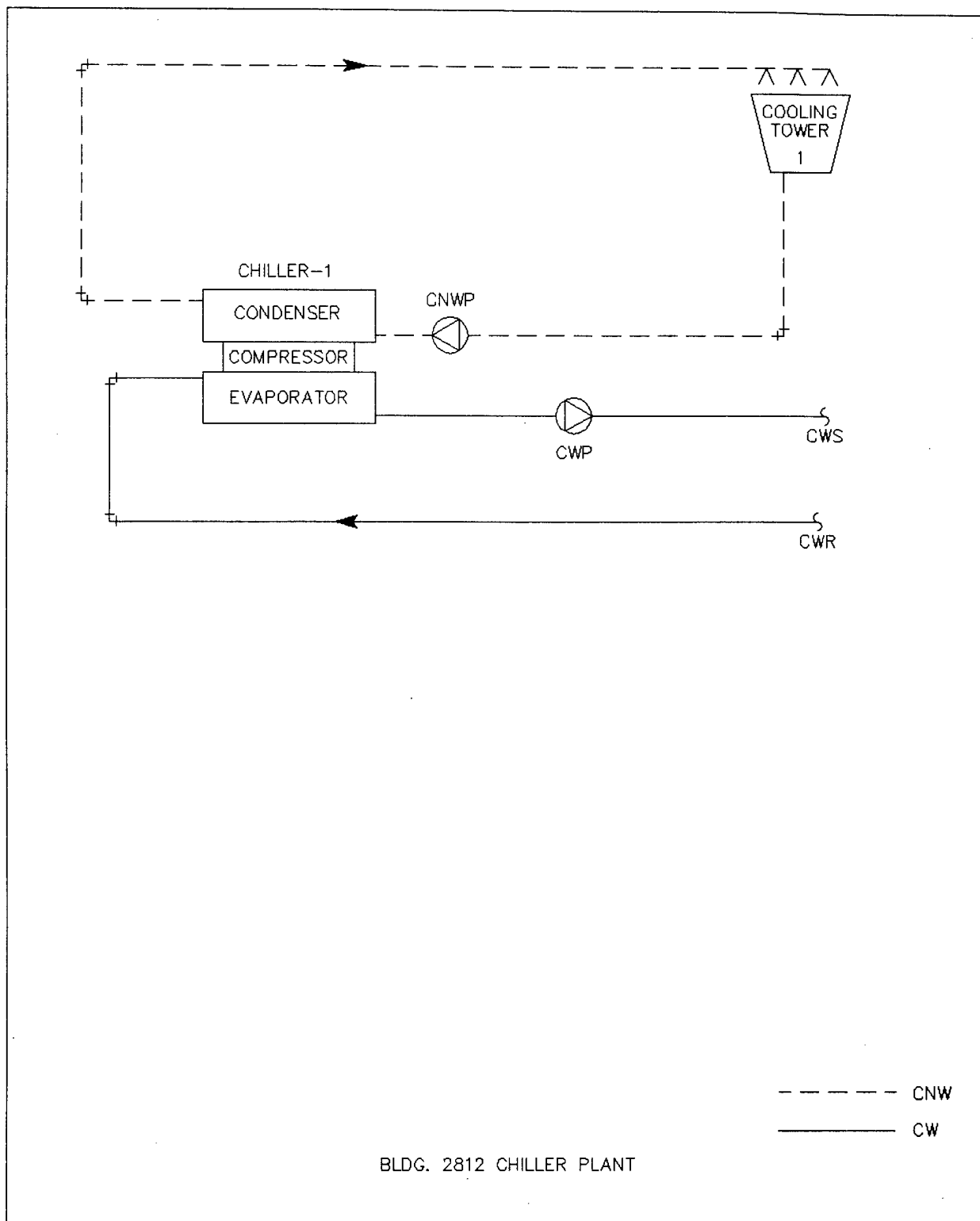
FIGURE 2-7. SCHEMATIC OF CHILLERS, CENTRAL PLANT 2812
