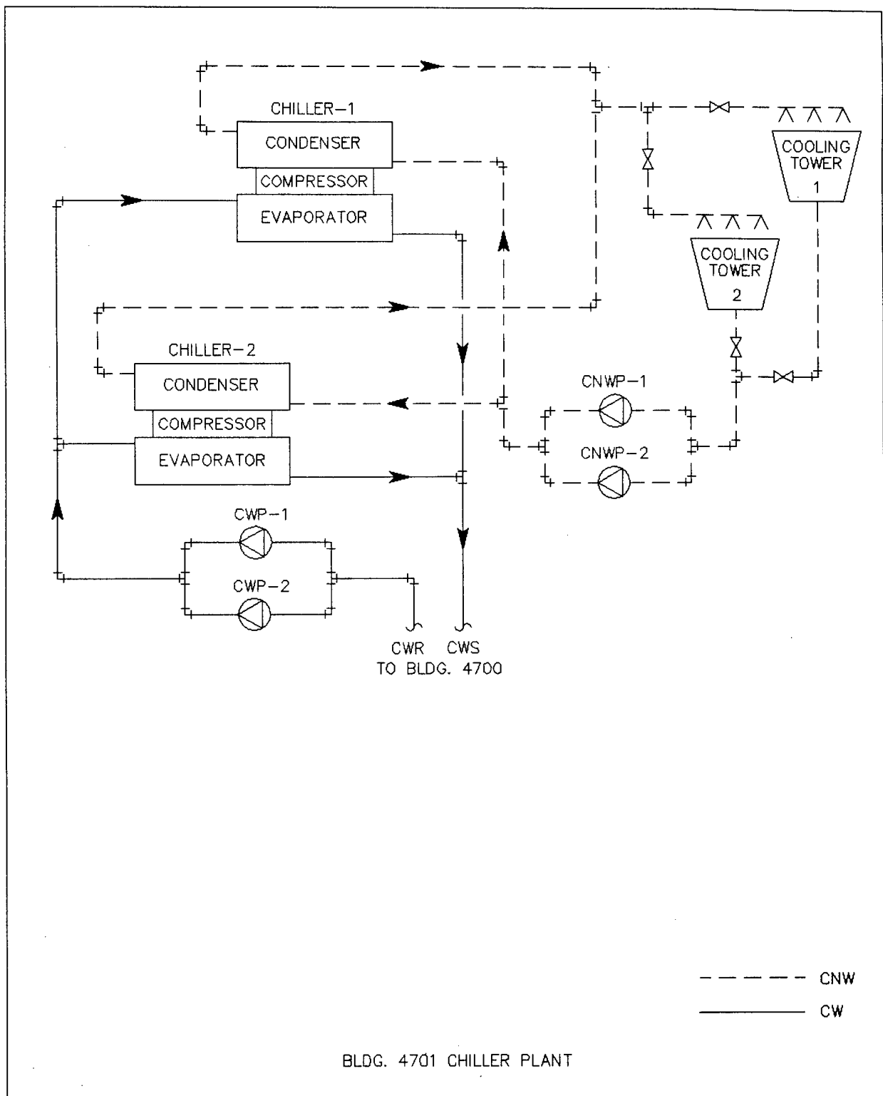
FIGURE 2-10. SCHEMATIC OF CHILLERS, CENTRAL PLANT 4701
