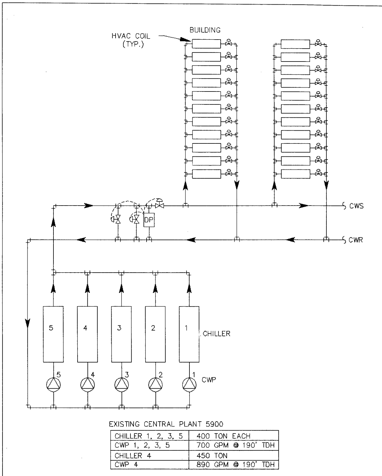
FIGURE 4-1, EXISTING CHILLED WATER PIPING
