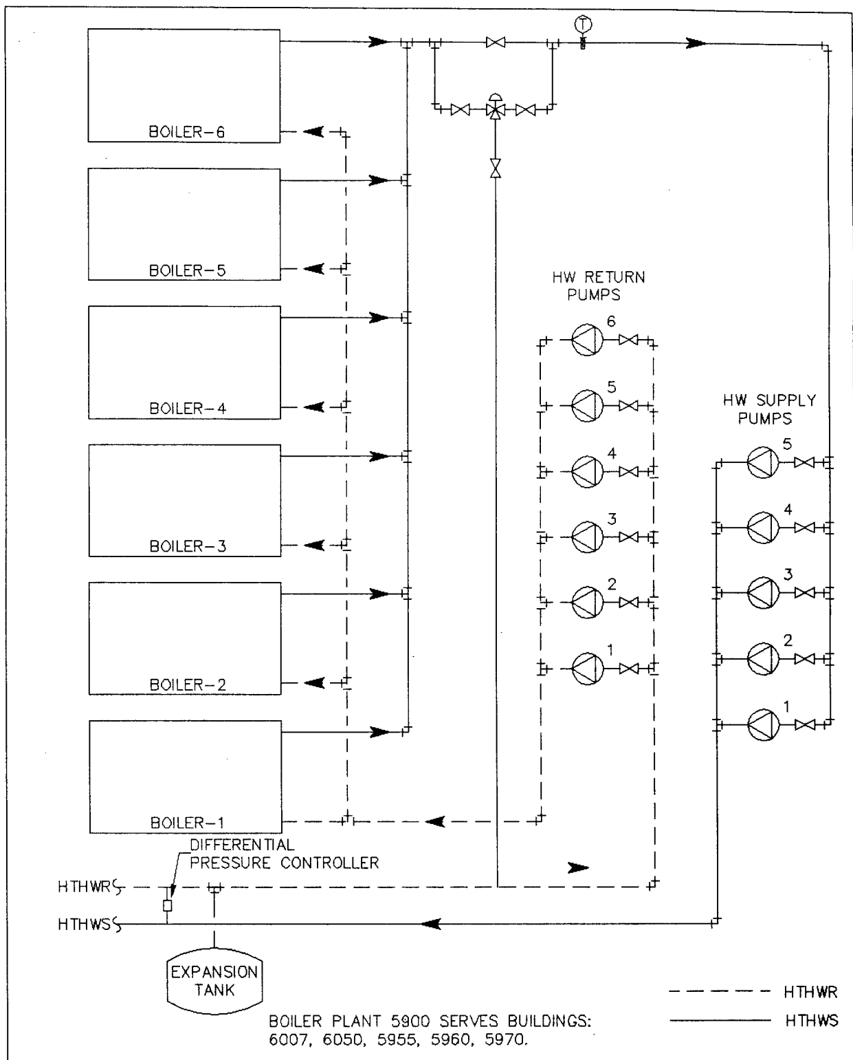
FIGURE 2-17. SCHEMATIC OF BOILERS, CENTRAL PLANT 5900
