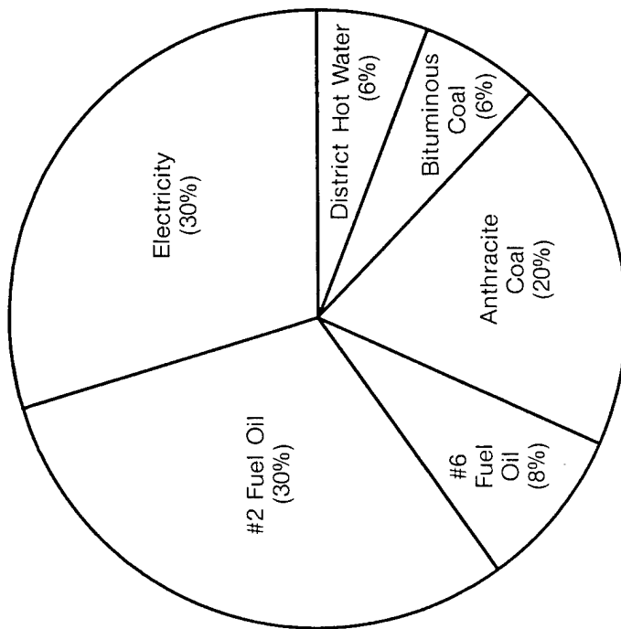
FY 81 Community Energy Use (Total = 1921.6 \times 10^9 Btu = 100%)
