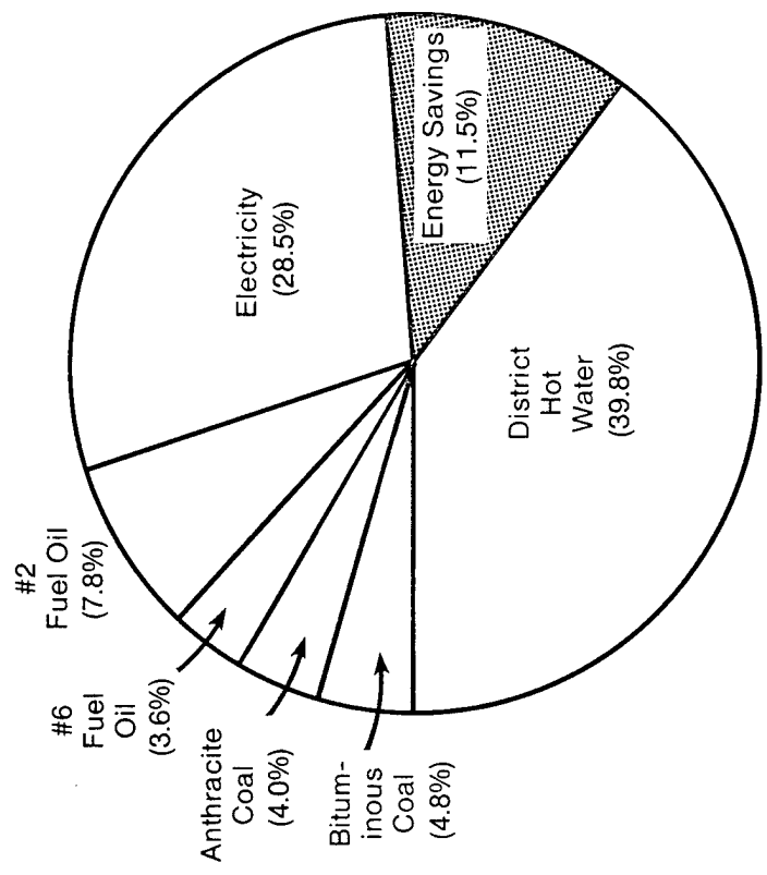
FY 85 Projected Energy Use with ECIP Projects (Total = 1699.9 \times 10^9 Btu = 88.5% of FY 81)
