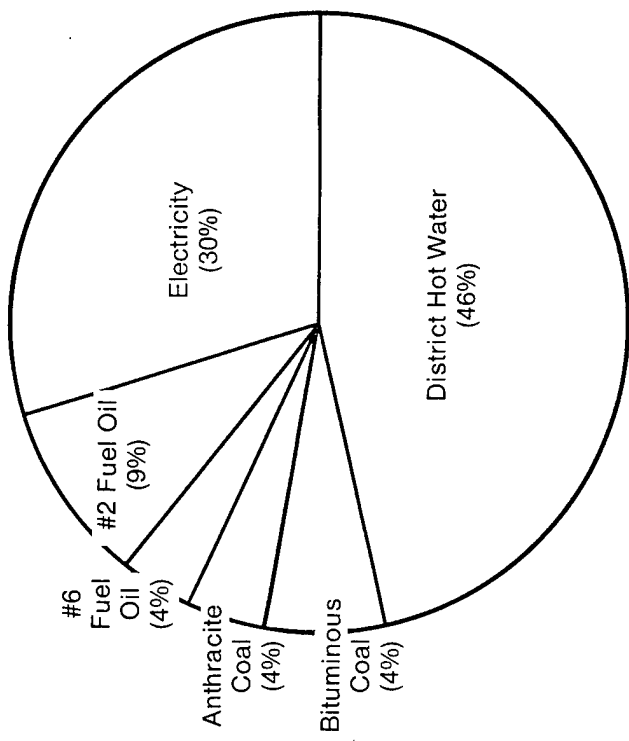
FY 81 Community Energy Use (Total = 1921.6 \times 10^9 Btu = 100%) (Adjusted For 1985 District Hot Water Distribution)
