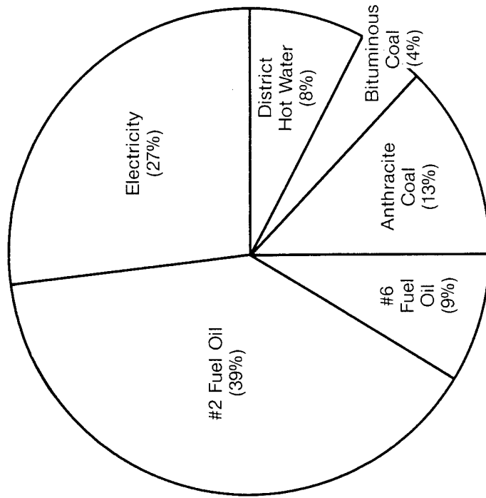
FY 81 Energy Cost (Total = $10,202,600 = 100%)
