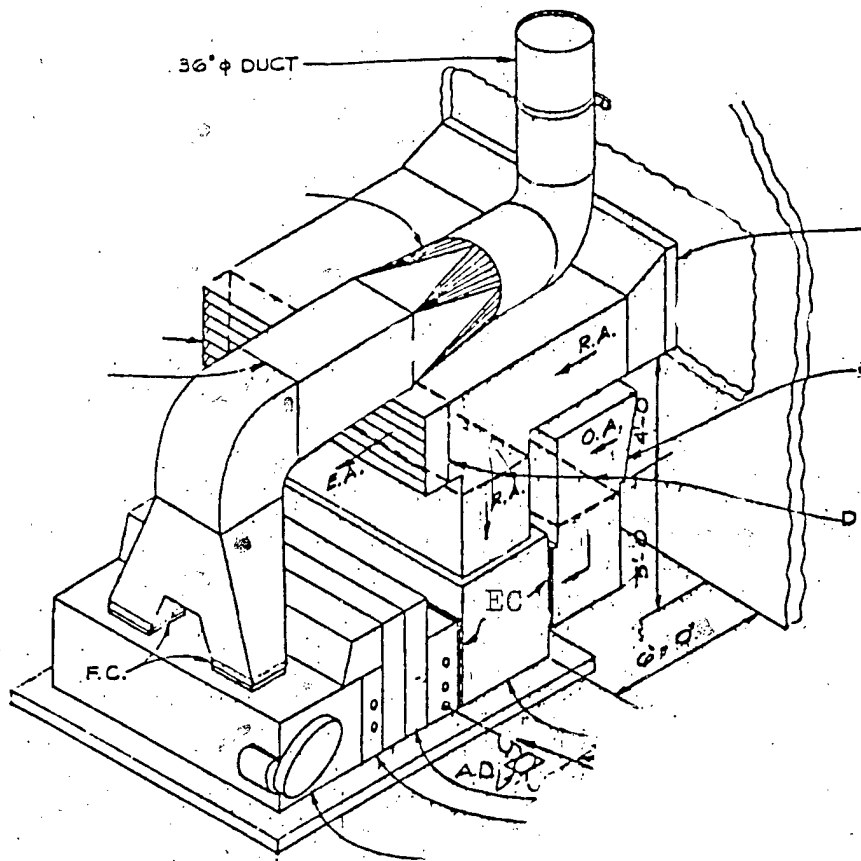
Existing Air Handler
