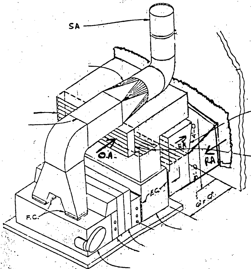
Air Handler With Proposed Changes
