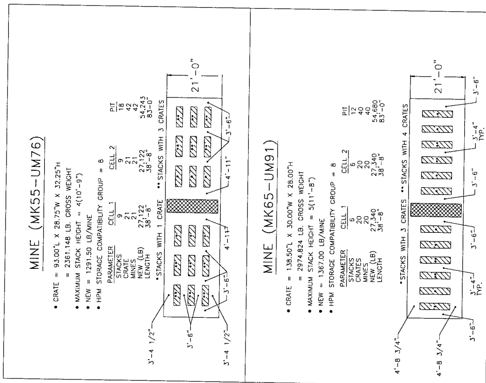
Figure 4-13. HPM storage plans: Mine (Mk55-UM76), and Mine (Mk65-UM91).
