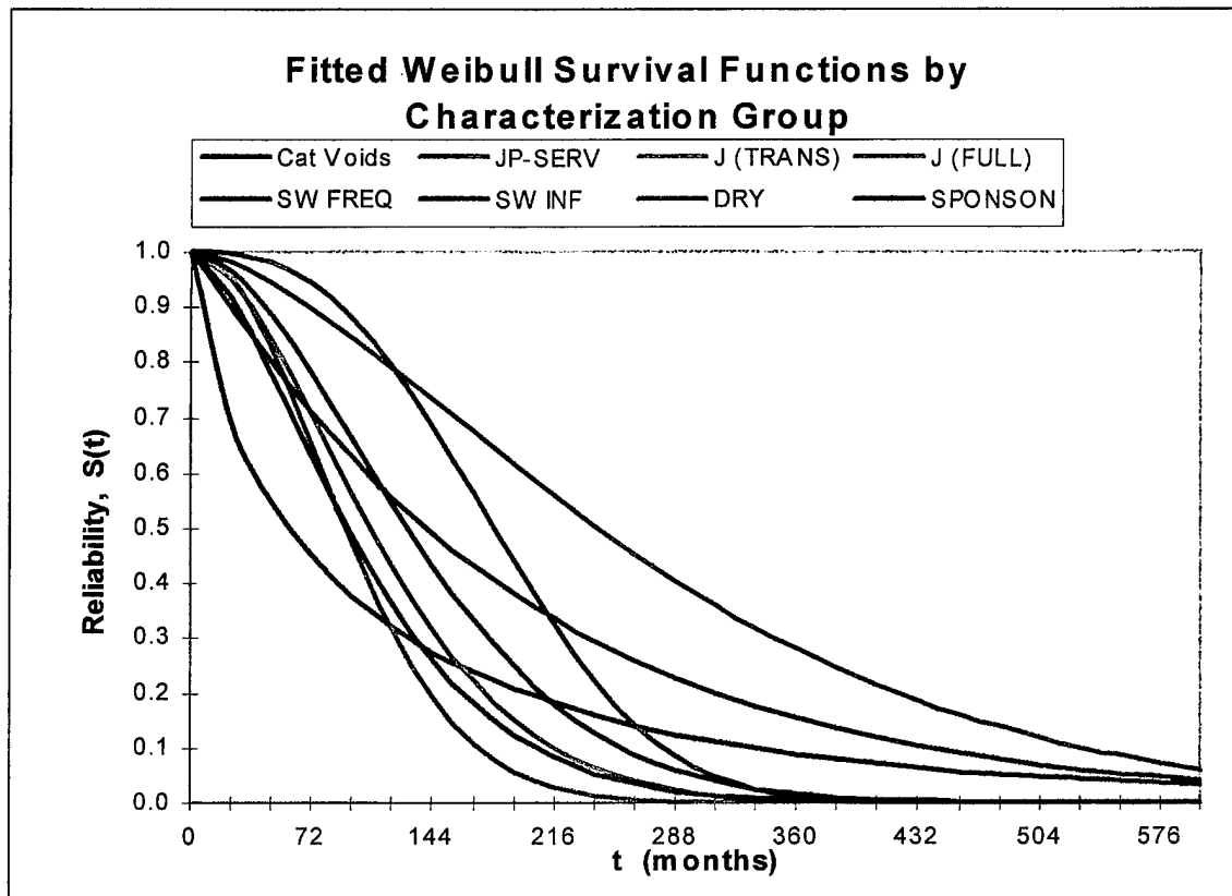
Figure V-4 Fitted Weibull survival functions for each tank characterization group.
