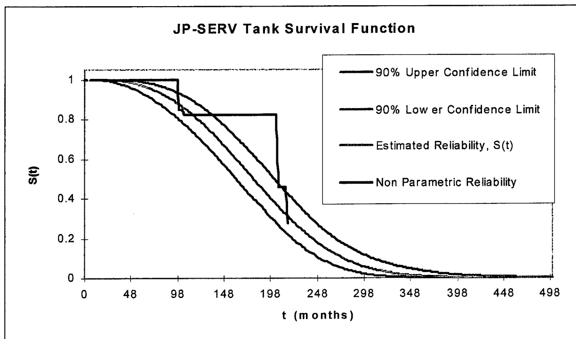
Figure V-5 JP-SERV Weibull Fit 90% Confidence Interval Bounds.
