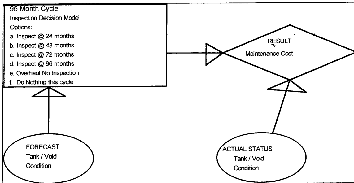
Figure VI-1 Influence Diagram for single 96 month period (between Overhaul opportunities) Tank Inspection Decision.
