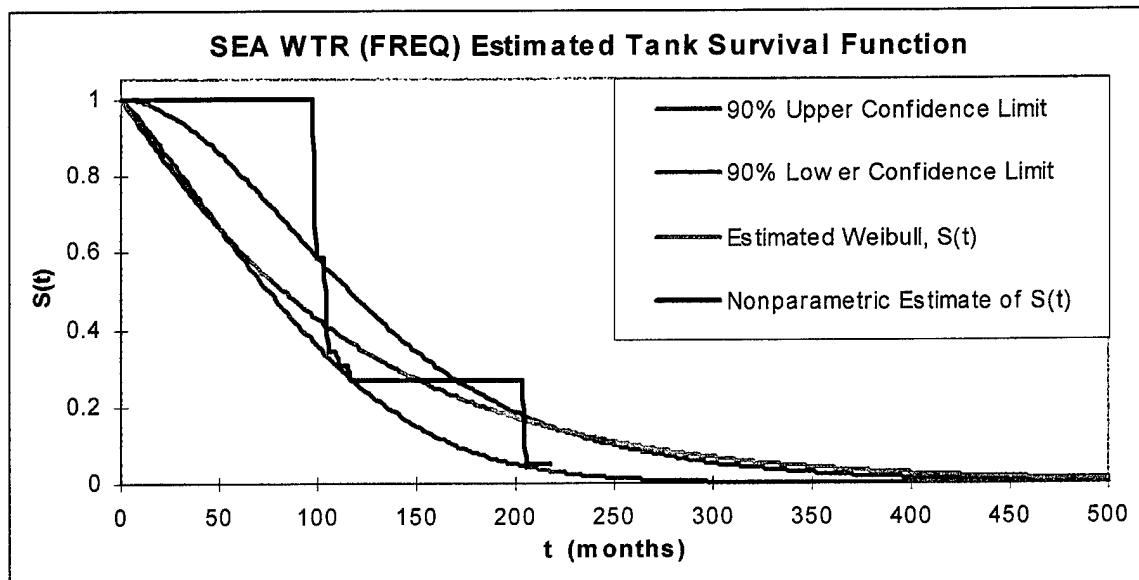
Figure H-5 Maximum Likelihood fit (with 90% confidence bounds) of Weibull distribution describing the survival function S(t) of tank coatings for SEA WTR (FREQ) Group tanks compared to the nonparametric survival distribution.
