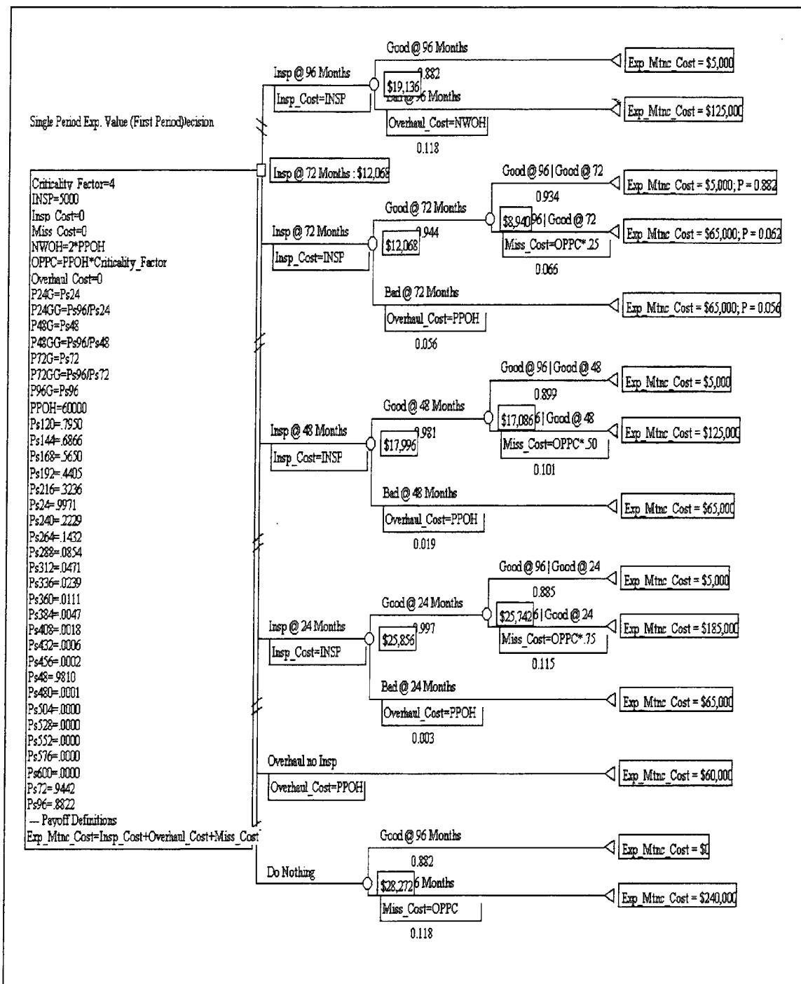
Figure VI-4 Roll-back of Tank Inspection Decision Model showing expected costs and recommended life to take in JP-SERVICE tanks during the first 96 month period of tank coating life.
