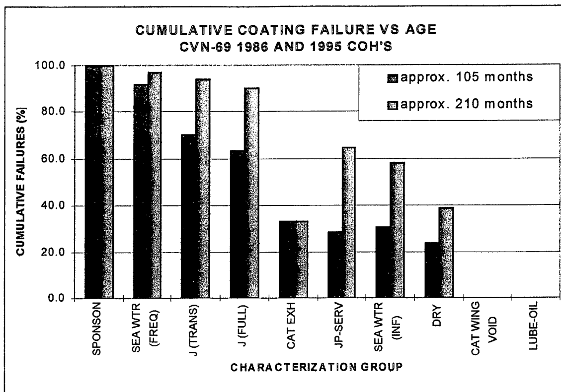
Figure A-3 Observed Cumulative Tank Coating Failure for CVN 69, by Characterization Group, for tanks inspected at approximately 105 and 210 months of Coating age.
