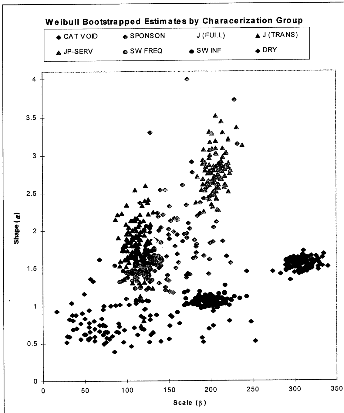
Figure V-6 Bootstrapped estimates for Weibull parameters by characterization group.
