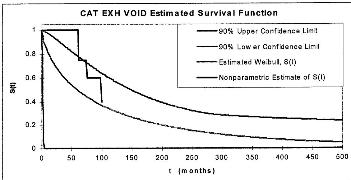
Figure K-5 Maximum Likelihood fit (with 90% confidence bounds) of Weibull distribution describing the survival function S(t) of tank coatings for CAT EXH VOID Group tanks compared to the nonparametric survival distribution.
