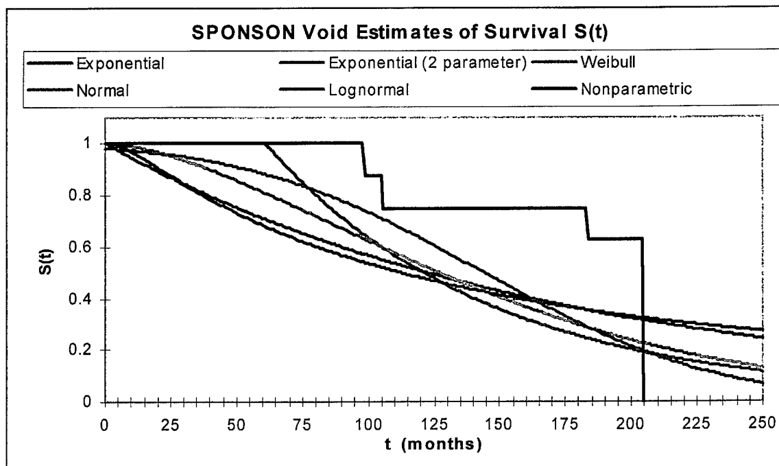
Figure M-6 Maximum Likelihood fits of parametric and nonparametric candidate distributions describing the survival function S(t) of tank coatings for SPONSON Group tanks.
