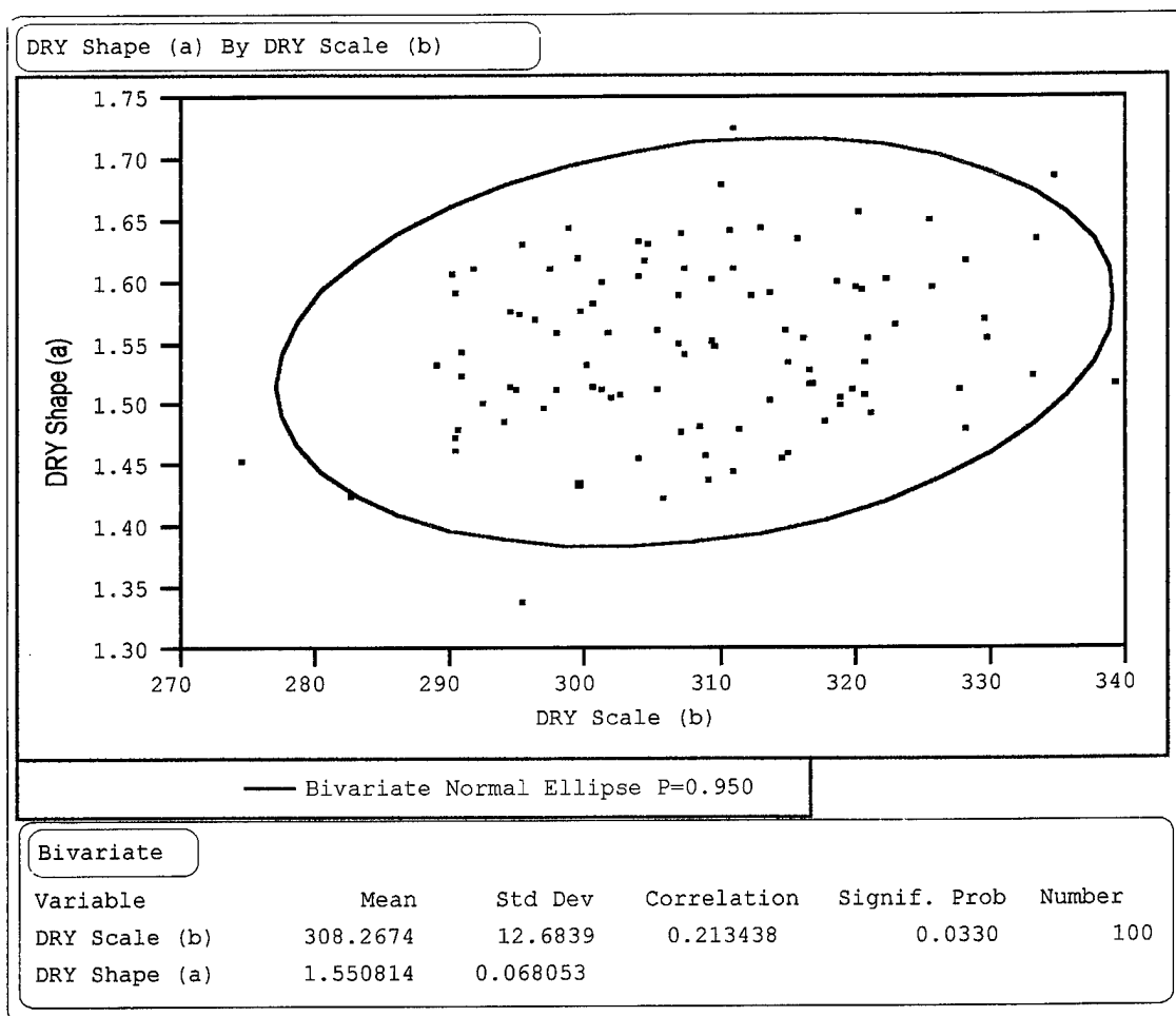
Figure L-4 Bootstrapped estimates and 95% confidence ellipse for Weibull parameters of Shape ( \alpha ) and Scale ( \beta ) for the DRY group. (This figure is a screen capture from JMP version 3.1.6 by SAS Institute Inc.)
