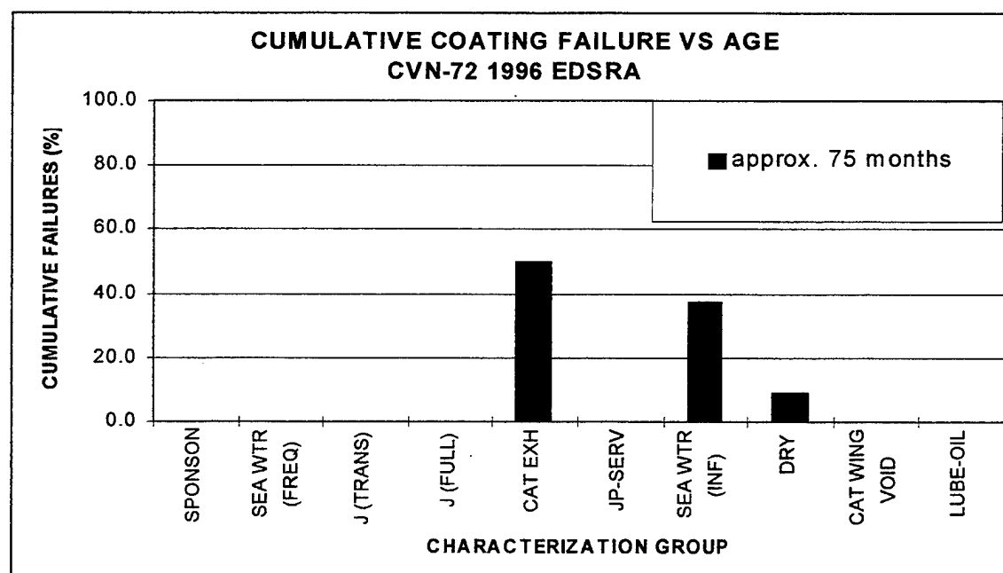
Figure C-2 Observed Cumulative Tank Coating Failure for CVN 72, by Characterization Group, for tanks inspected at approximately 75 months of Coating age.
