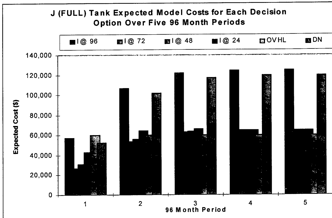
Figure F-9 Expected Model costs for various J(FULL) Group tank inspection decision options over the first five 96 month periods of tank coating life.
