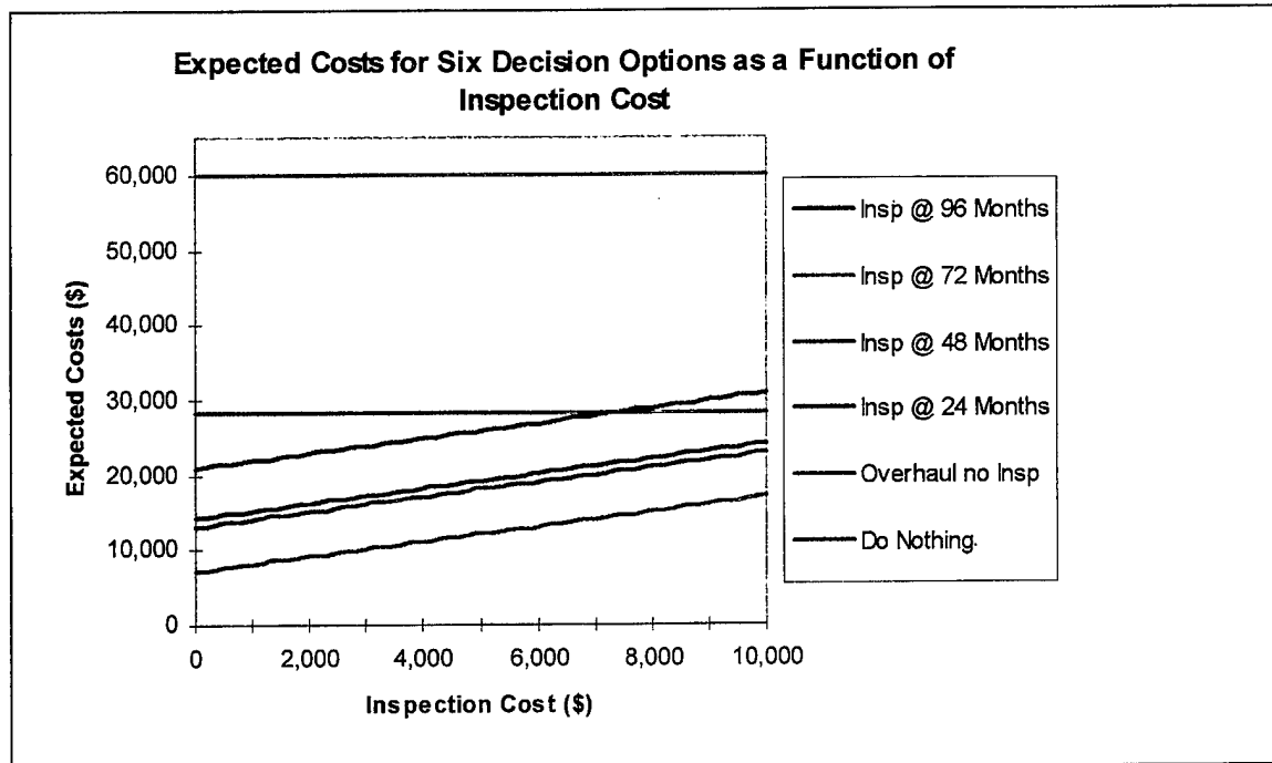
Figure VI-9 Sensitivity of the Inspection Decision Model to Inspection Cost.
