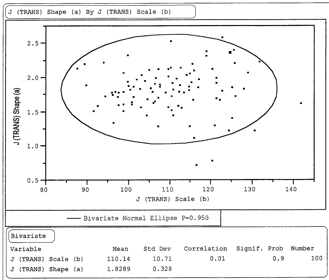
Figure E-4 Bootstrapped estimates and 95% confidence ellipse for Weibull parameters of Shape ( \alpha ) and Scale ( \beta ) for the J(TRANS) group. (This figure is a screen capture from JMP version 3.1.6 by SAS Institute Inc.)
