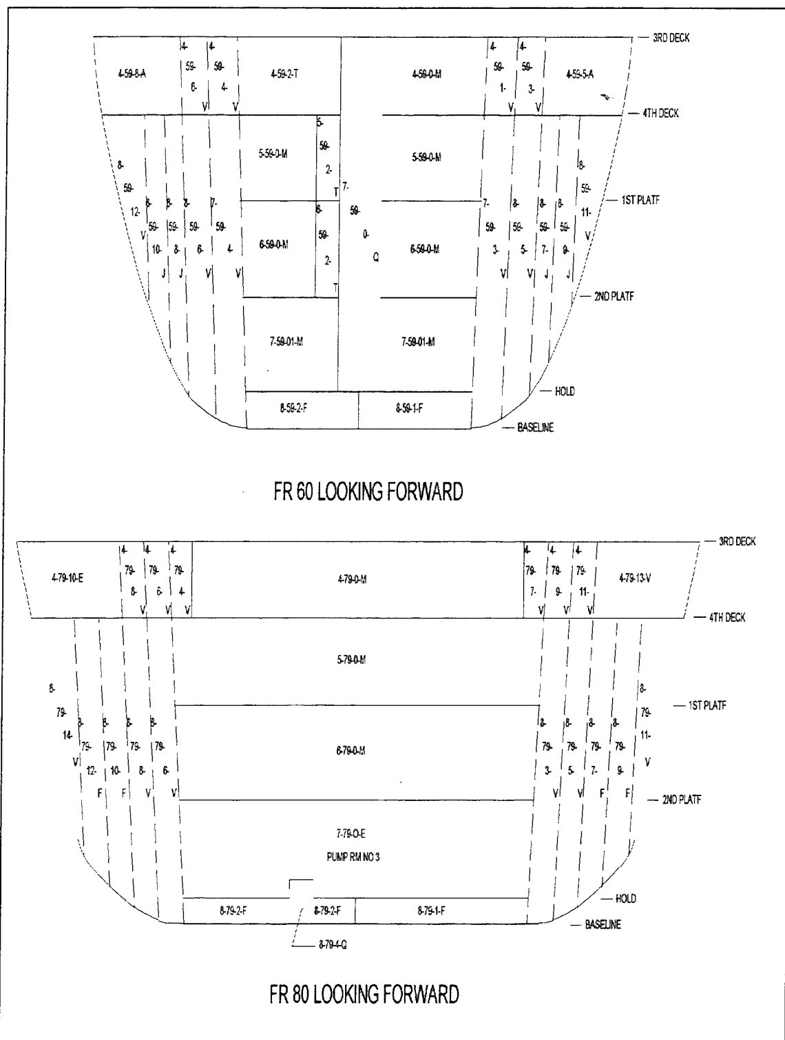
Figure IV-4 Forward looking layout of 4 th and 8 th deck tanks frames 60 and 80 of CV 64.
