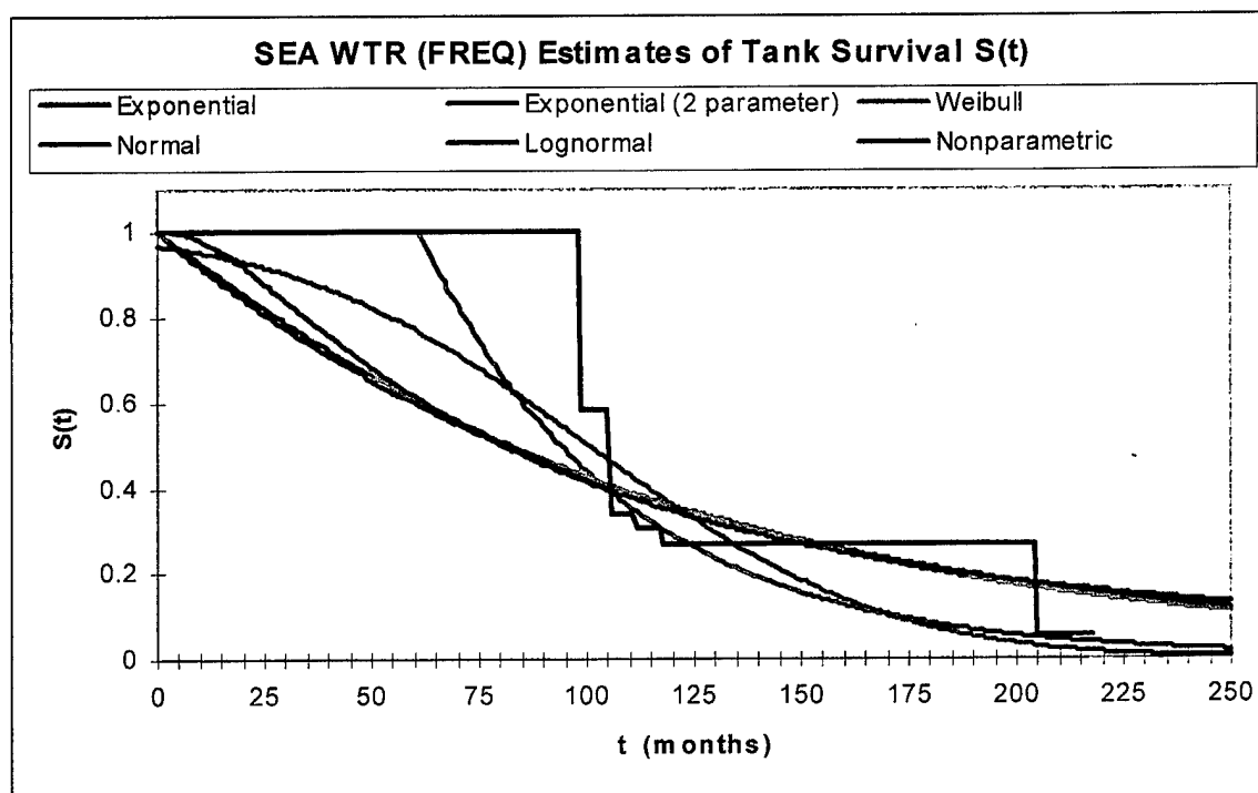
Figure H-6 Maximum Likelihood fits of parametric and nonparametric candidate distributions describing the survival function S(t) of tank coatings for SEA WTR (FREQ) Group tanks.
