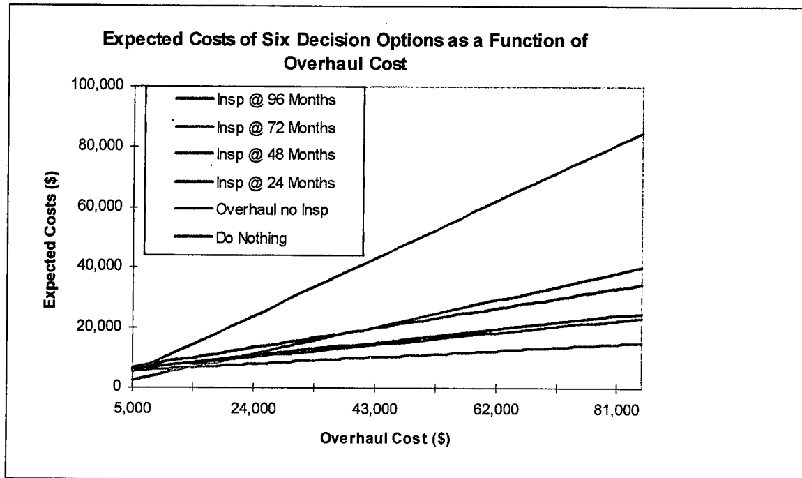
Figure VI-8 Sensitivity of the Inspection Decision Model to Overhaul Cost.
