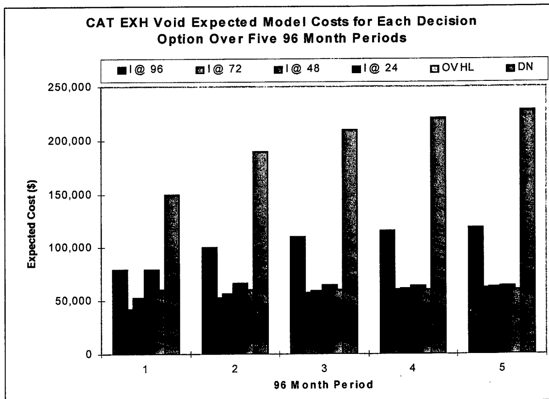
Figure K-9 Expected Model costs for various CAT EXH VOID Group tank inspection decision options over the first five 96 month periods of tank coating life.
