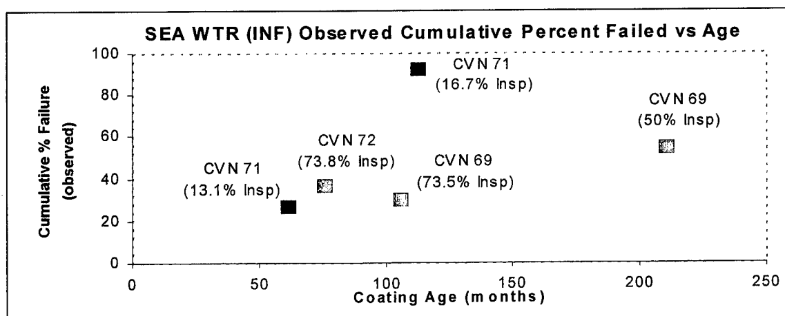
Figure V-2 Comparison of observed failures of SEA WTR (INF) tank coating at different coating ages for CVN 69, 71, and 72.
