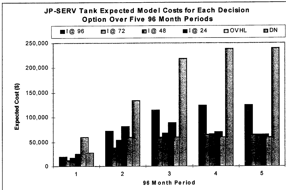
Figure D-9 Expected Model costs for various JP-SERV Group tank inspection decision options over the first five 96 month periods of tank coating life.
