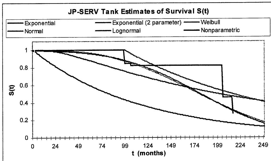
Figure D-6 Maximum Likelihood fits of parametric and nonparametric candidate distributions describing the survival function S(t) of tank coatings for JP-SERV Group tanks.
