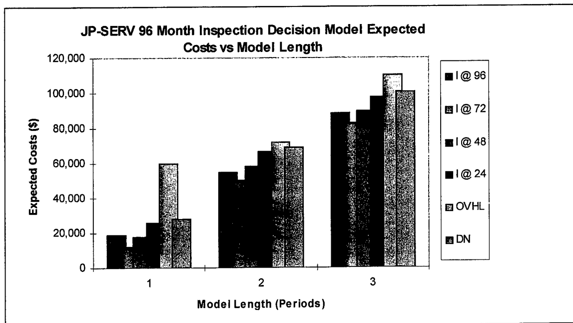
Figure VI-10 Comparison of decision option preferences for JP-SERV by period length of 96 month Inspection Decision Model.
