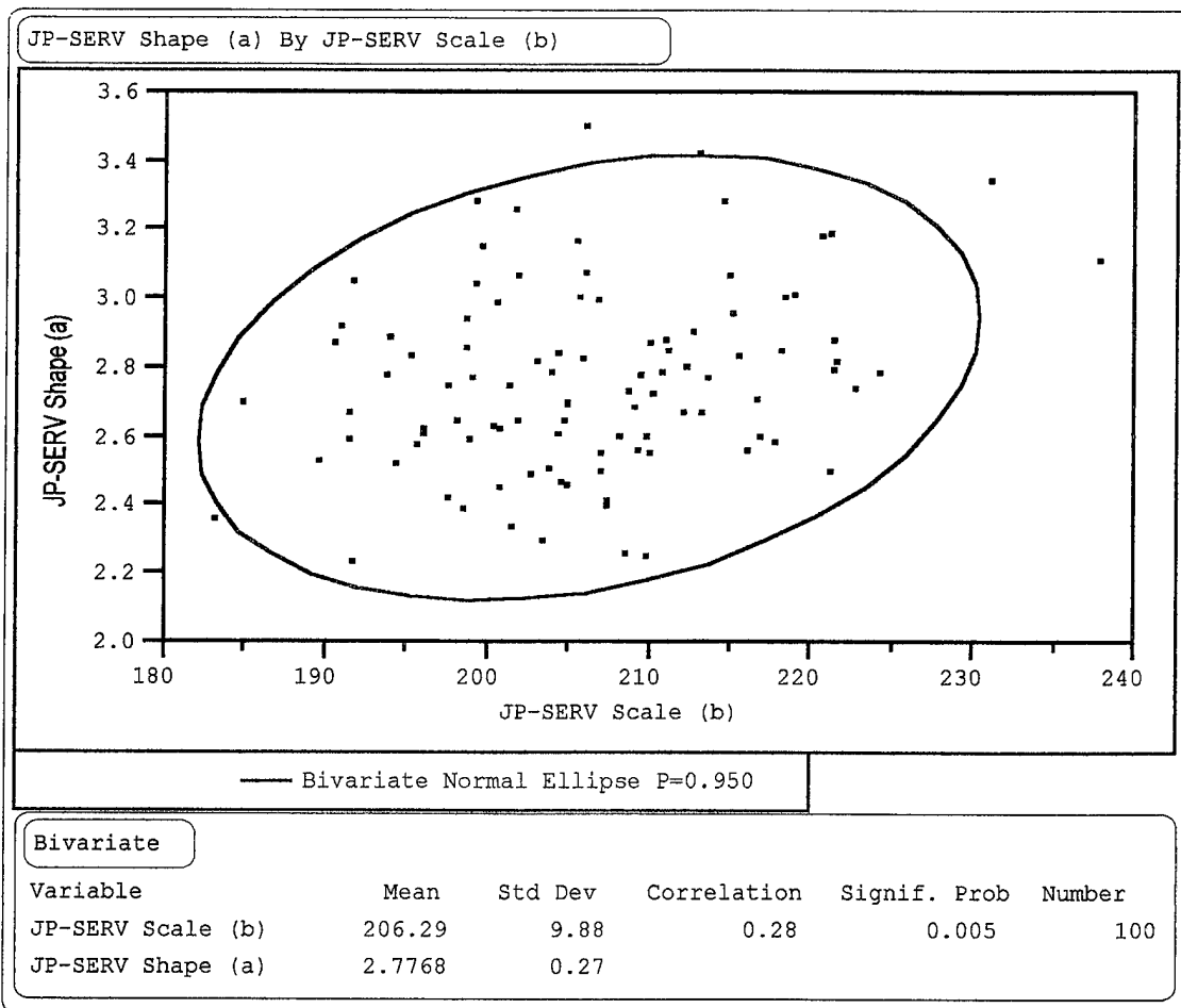
Figure D-4 Bootstrapped estimates and 95% confidence ellipse for Weibull parameters of Shape ( \alpha ) and Scale ( \beta ) for the JP-SERV group. (This figure is a screen capture from JMP version 3.1.6 by SAS Institute Inc.)
