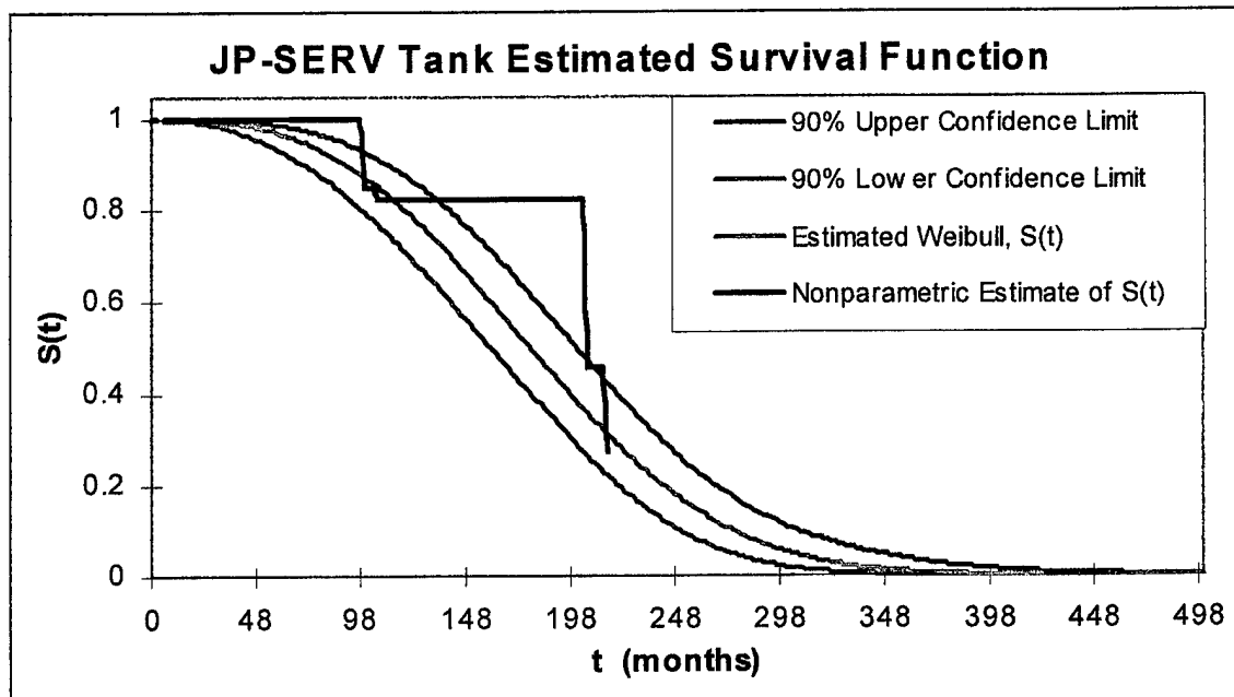
Figure D-5 Maximum Likelihood fit (with 90% confidence bounds) of Weibull distribution describing the survival function S(t) of tank coatings for JP-SERV Group tanks compared to the nonparametric survival distribution.
