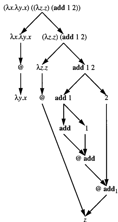
Figure 8.18: PSL computation graph for Example 8.3. The threads are numbered left-to-right, i.e. , the leftmost spine is \tau_0 , the next leftmost is \tau_1 , etc. Note that this is not the order of creation of the threads in this example.
