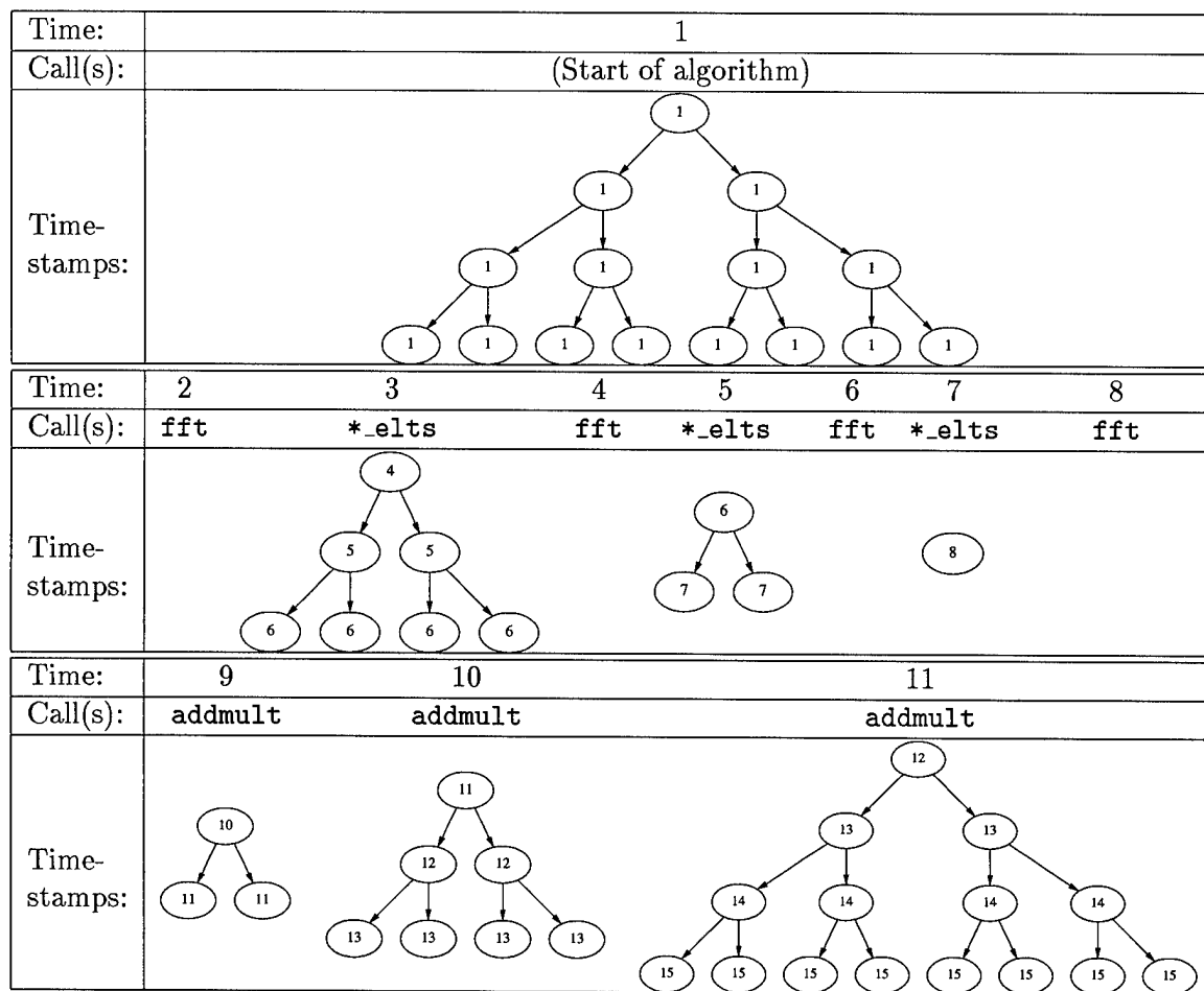
Figure 10.8: Time-stamps during PSL FFT algorithm. Tree nodes are labeled with their idealized time-stamps. The trees are the result of the given function call made at the given idealized time.
