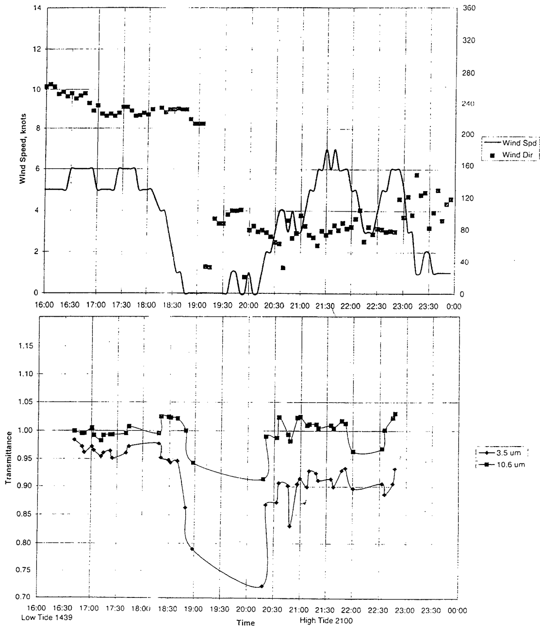
2 February 1996 Wind Speed and Direction, Scripps Pier
