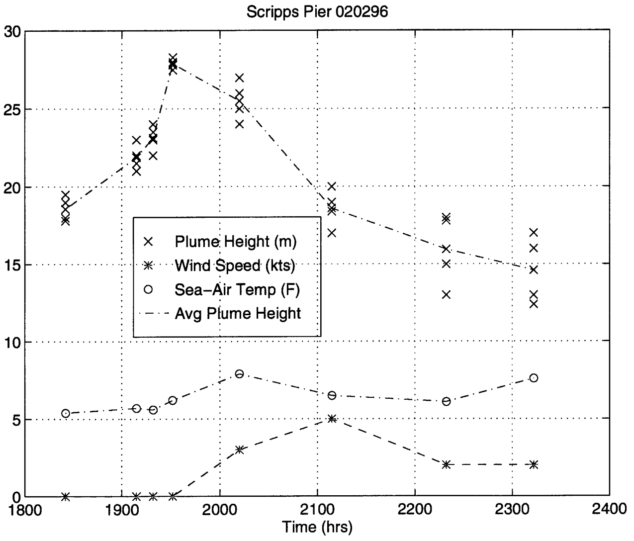
Figure 5.3 Scripps Pier data for 020296. Early observations indicate development of tall standing plumes. As wind speed increases, a corresponding decrease in plume height and increase in plume variability develop.
