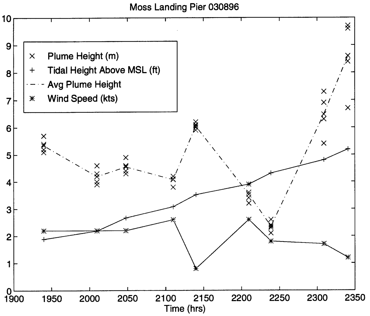
Figure 4.7 Moss Landing Pier data for 030896. Strong correlation between incoming tide on a steep beach face creating plunging breakers. The plunging breakers combined with decreasing wind speeds allow the plumes to grow to greater heights over time.
