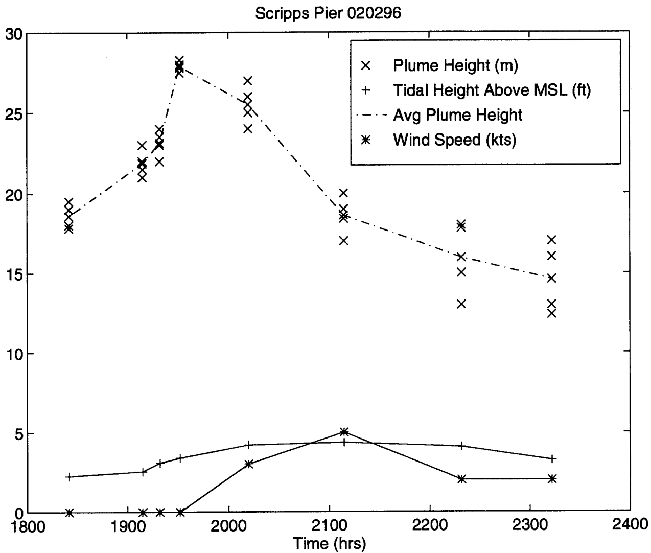
Figure 5.6 Scripps Pier plume height and tidal data for 020296. Minimal tidal variations associated with Scripps may indicate that plumes are more dependent on wind speed variations and temperature differences than breaker type for their development and structure.
