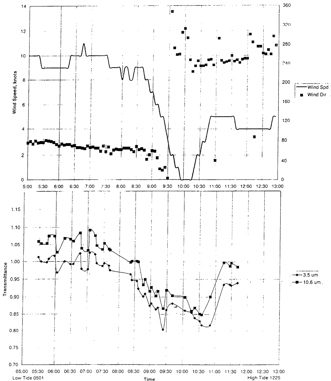
29 January 1996 Wind Speed and Direction, Scripps Pier
