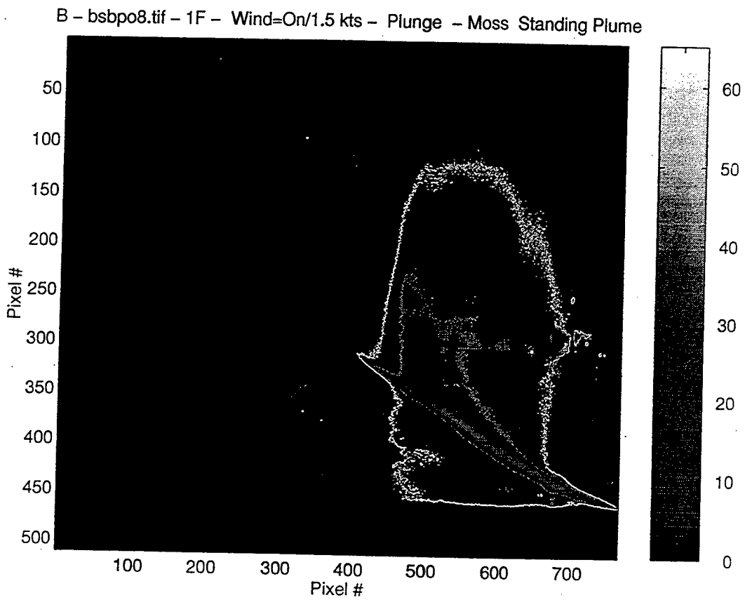
Figure 3.4a Pixel image of Moss Landing standing plume. The well defined finger structure observed in the Scripps Pier standing plumes (Figure 3.3b) are distorted by the light 1.5 kt onshore breeze.
