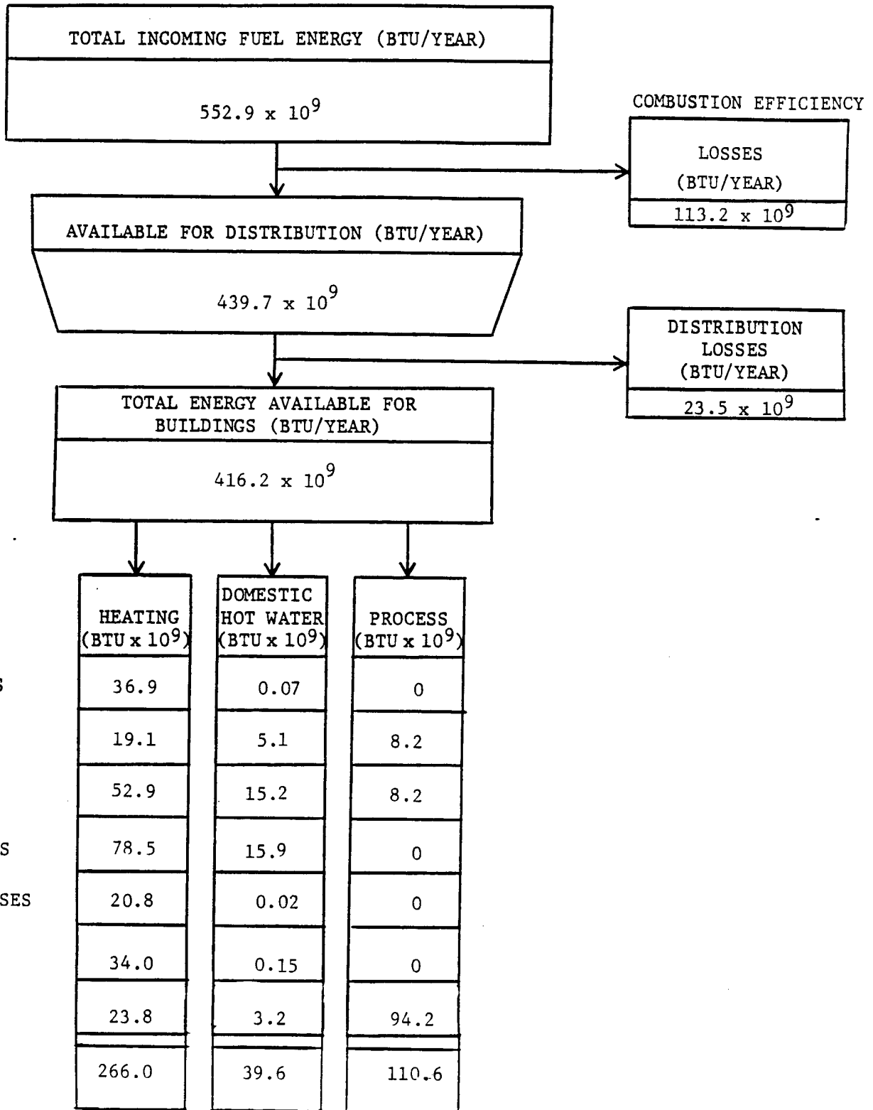
FIGURE 5. FOSSIL FUEL ENERGY PROFILE BY 1979 SOURCE: Appendix C, Increment A
