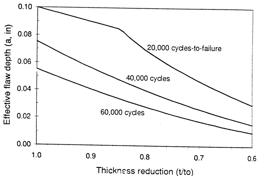
Figure 4. Constant-life diagram for the surface-cracked plate example
