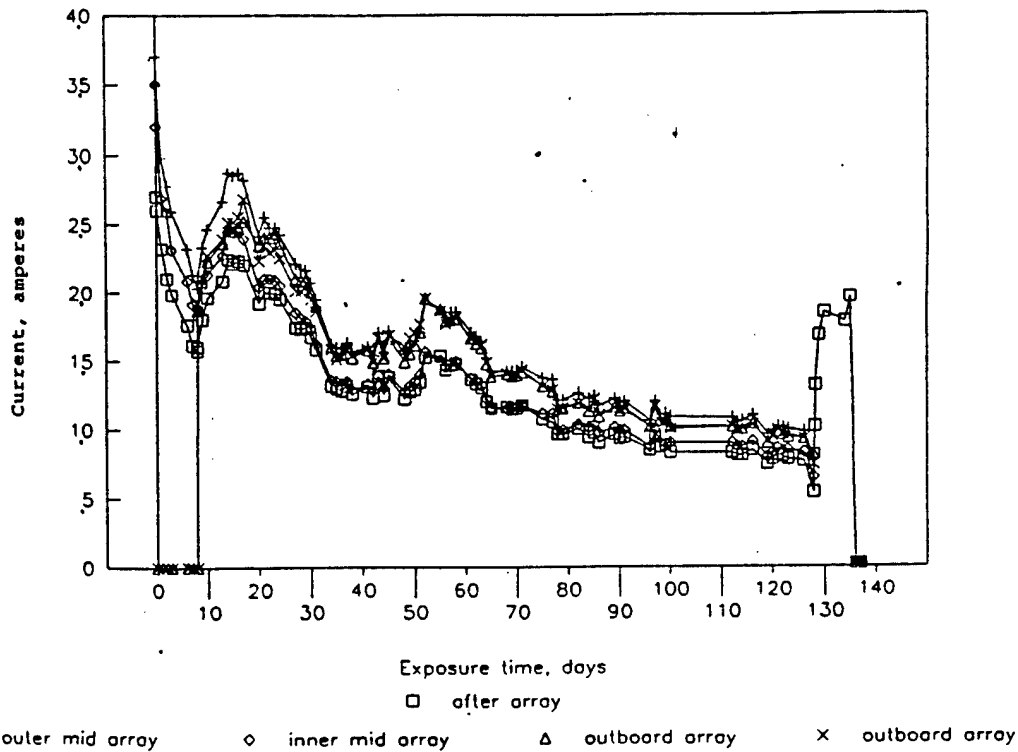
Figure 7 - Anode Currents
