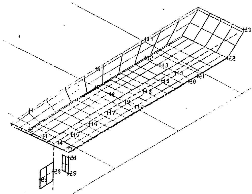
Figure 2 - Boundary Element Grid
