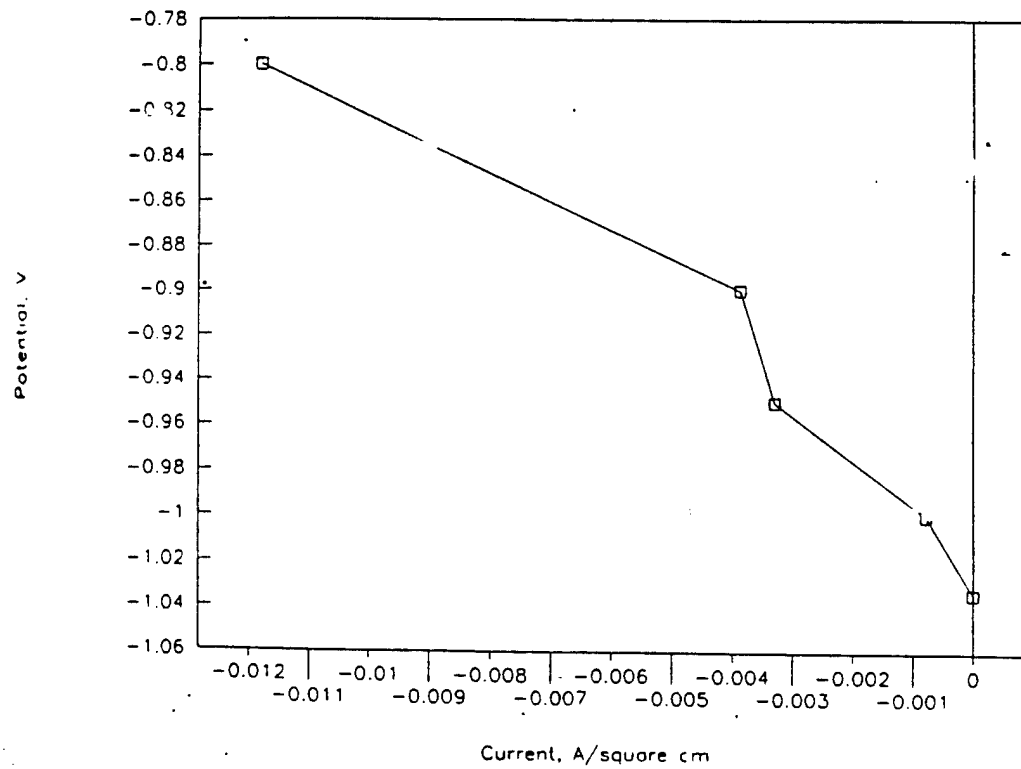
Figure 3 - Zinc Polarization Data
