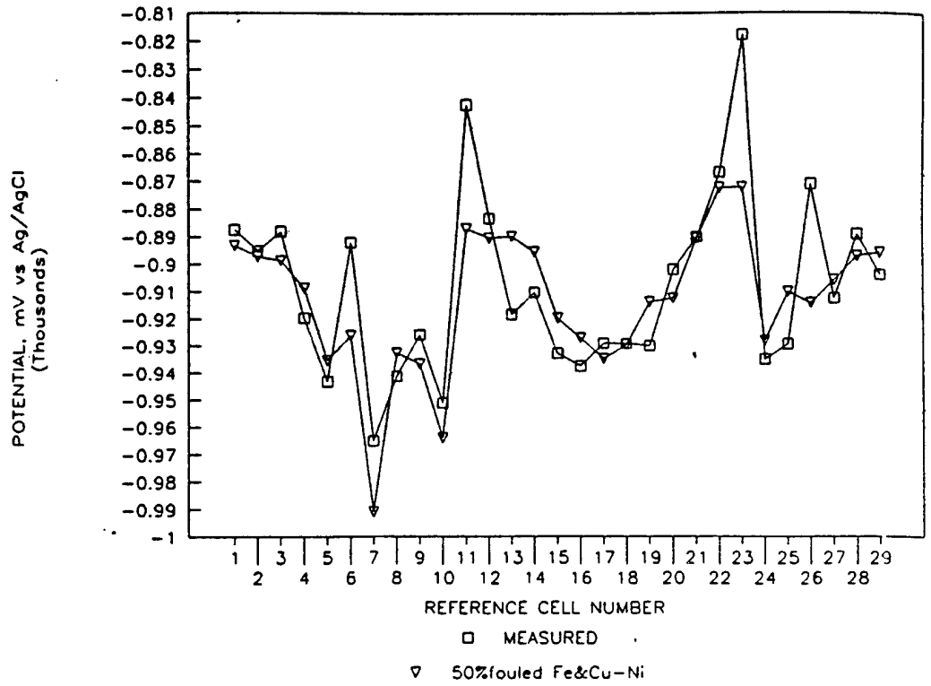
Figure 8 - Comparison of Model and Measured Potentials
