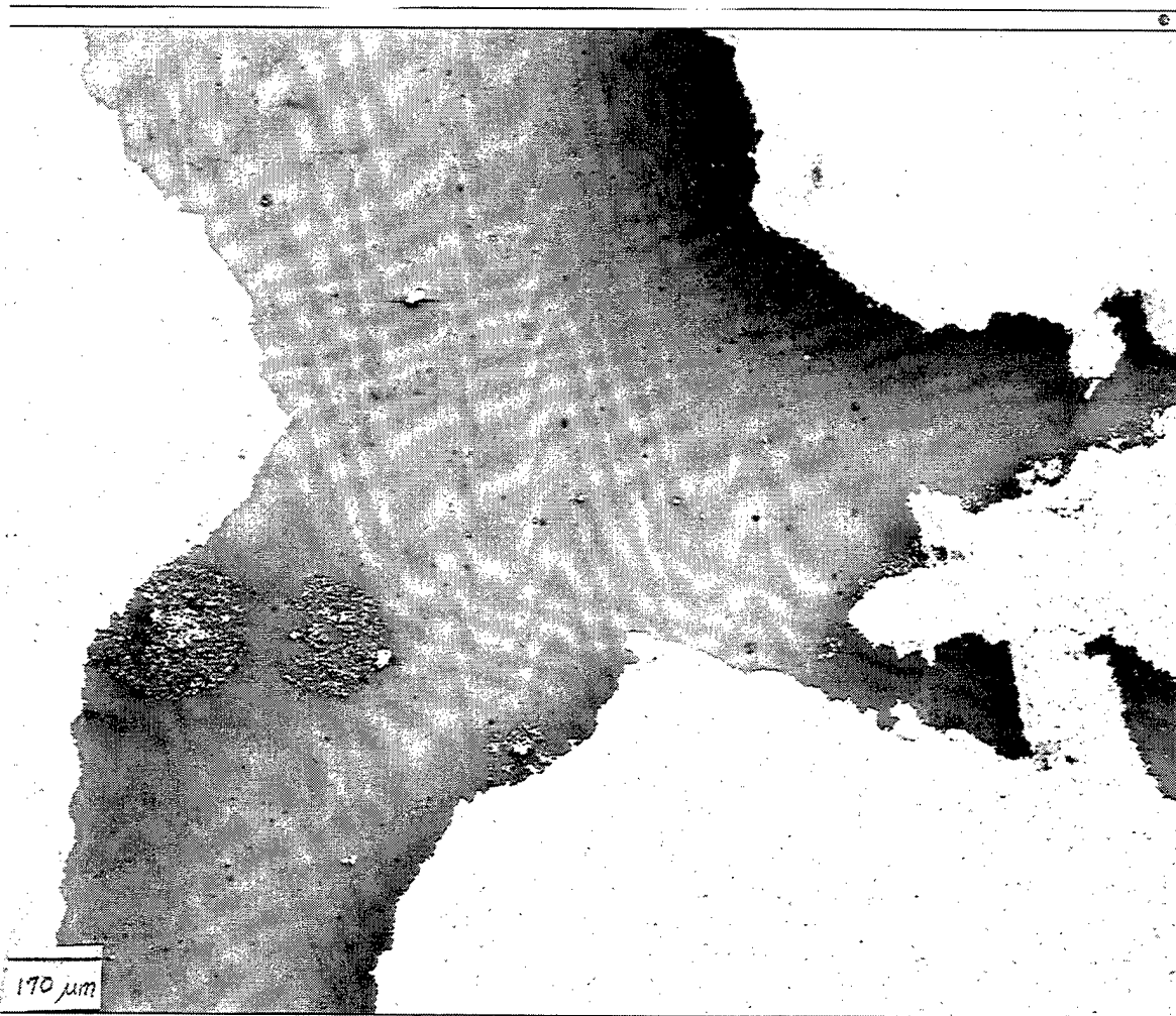
Figure 6: Secondary electron image of Ag metallization (light) on <100> CVDD (dark) without inter-layer clearly showing cracking and peeling of Ag paste following firing to 400 °C.
