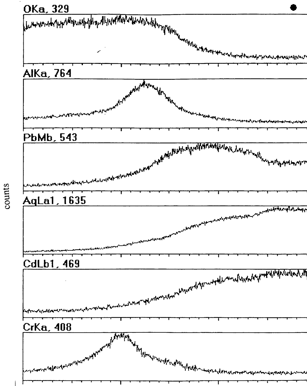
Figure 11: X-ray line scans from interfacial region of Ag-metallization (3350 FERRO) layer on 60nm Cr/150nm \text{Al}_2\text{O}_3 layer on glass substrate,
