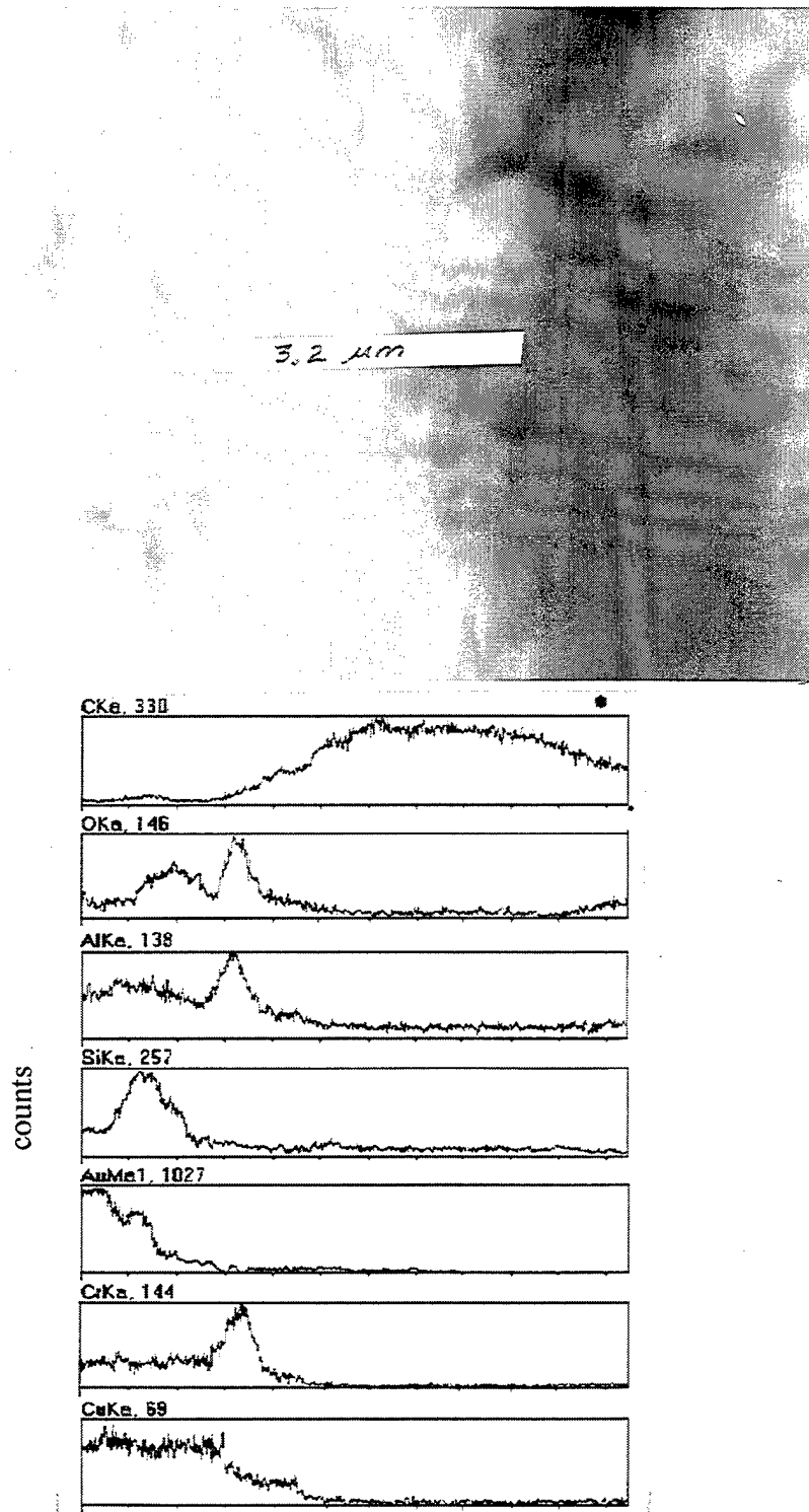
Figure 17: Secondary electron image and X-ray line scans from Au-metallization layer on 50nm Cr/165nm Al 2 O 3 layer on CVDD substrate. X-axis is 3.2 \mu\text{m} long.
