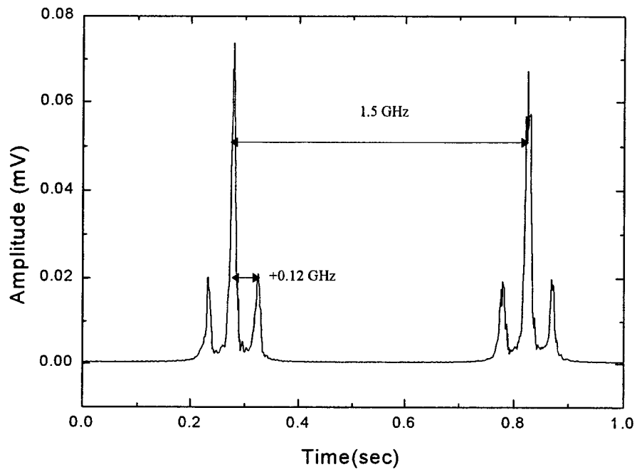
Figure 4.10. 60% modulation with 40 V p-p at 125 MHz.
