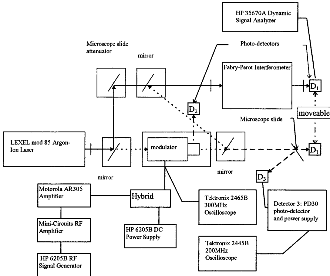
Figure 3.1. The modulator, the mirrors, and microscope slides were supported by kinematic mounts, allowing the beam path to be changed quickly. Detector 1 (D1) was alternated between the two positions indicated as required by the experiment.
