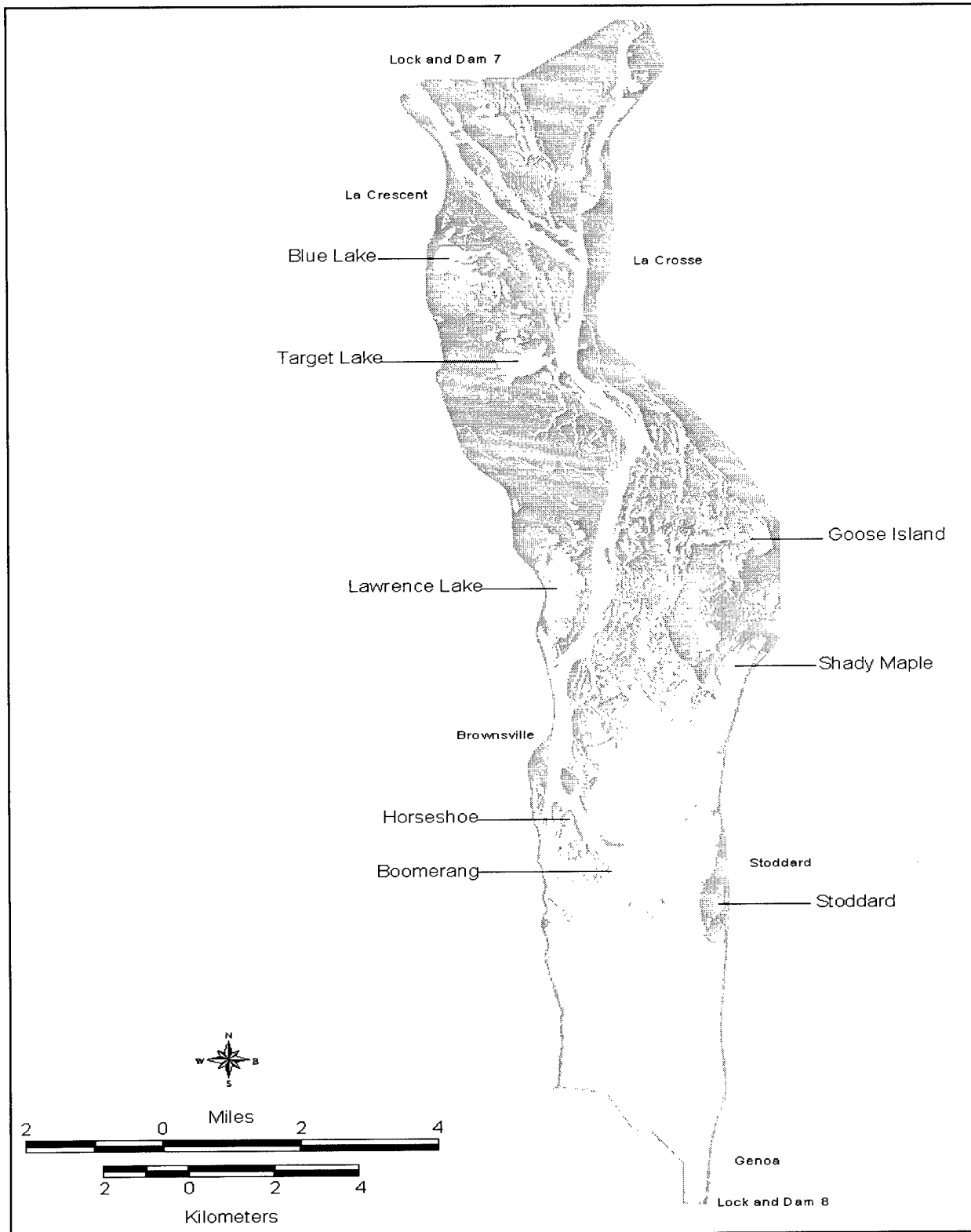
Figure 2. Transect locations in Pool 8, Upper Mississippi River System.
