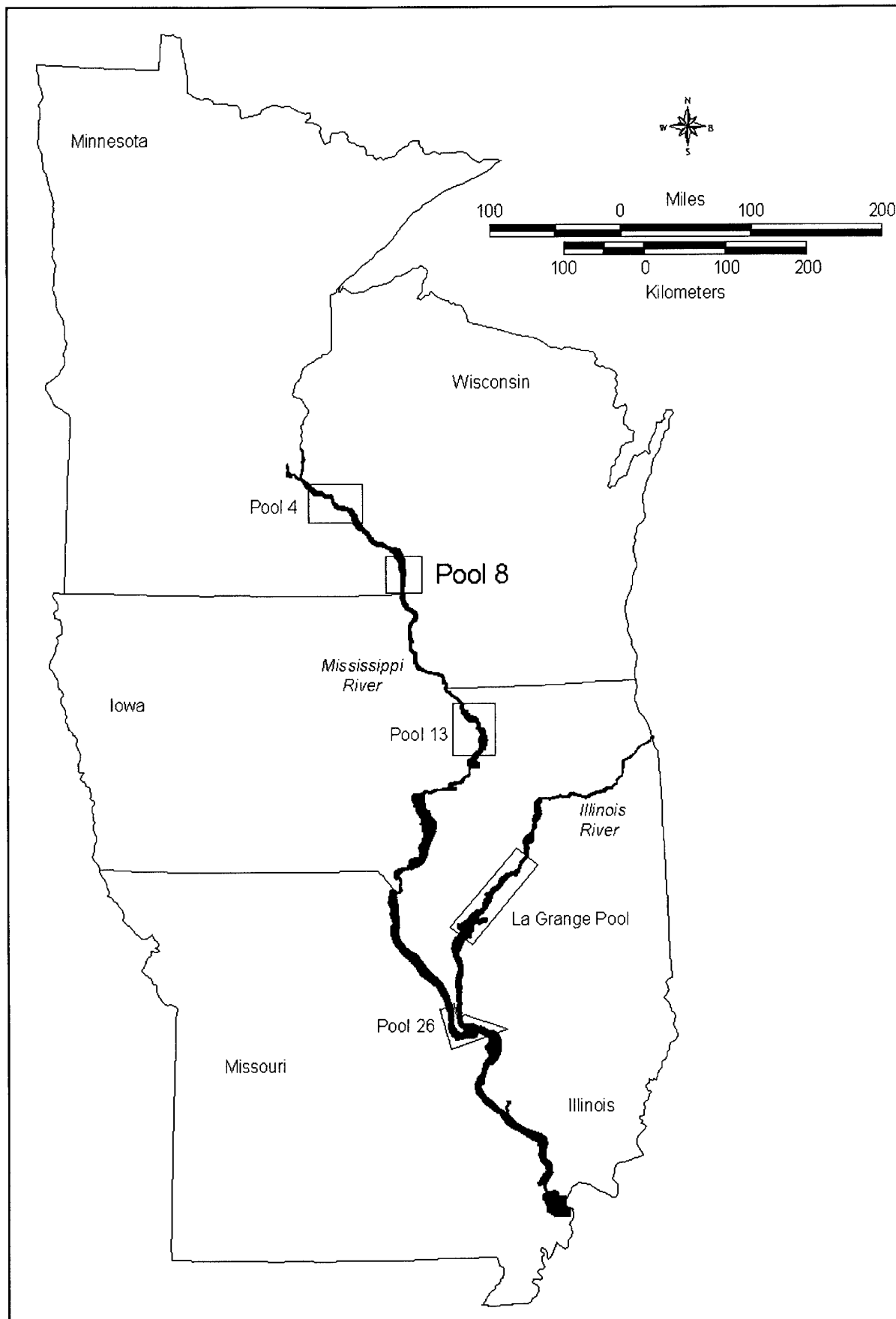
Figure 1. Mainstem of the Upper Mississippi River System and the Long Term Resource Monitoring Program study reaches for submersed aquatic vegetation.
