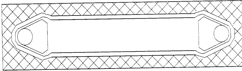
Figure 7.5: Redesigned Blank with Extended Glue Channels
