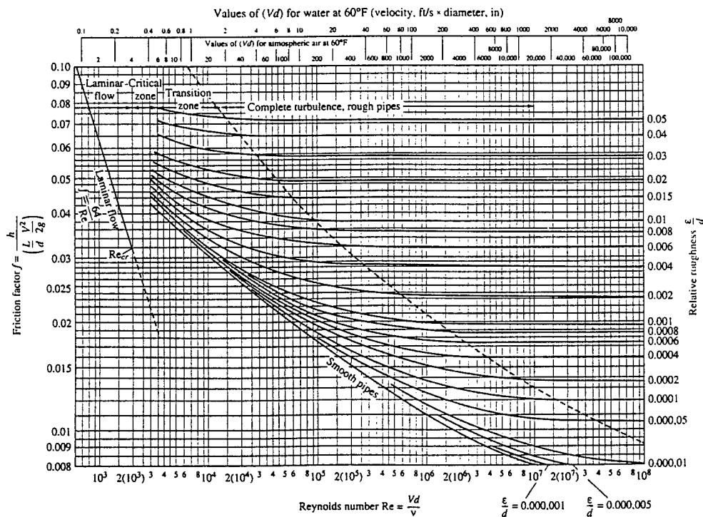
Figure 3.1: Moody Diagram
