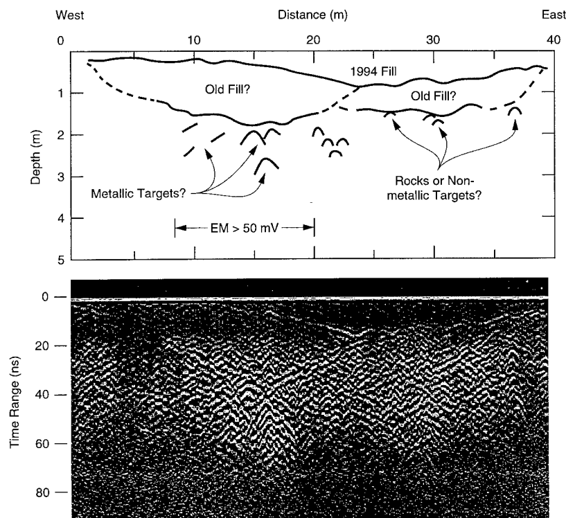
Figure 12. 400-MHz GPR profile and interpretative depth sections.
