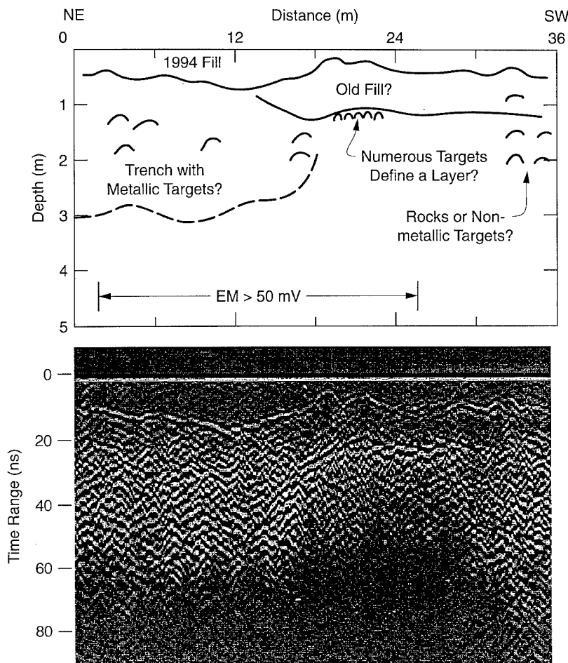
Figure 12 (cont'd). 400-MHz GPR profile and interpretative depth sections.
