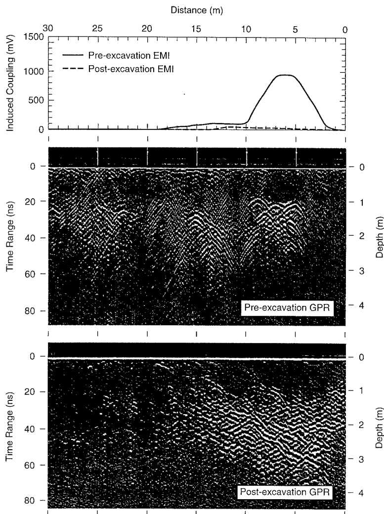
Figure 8. Profiles recorded along transect 11 (area A-3) with GPR and EMI. The excavation revealed fifty 55-gal. (208-L) steel barrels in the area distinguished by the broad EMI anomaly and the distinct GPR hyperbolic reflections.
