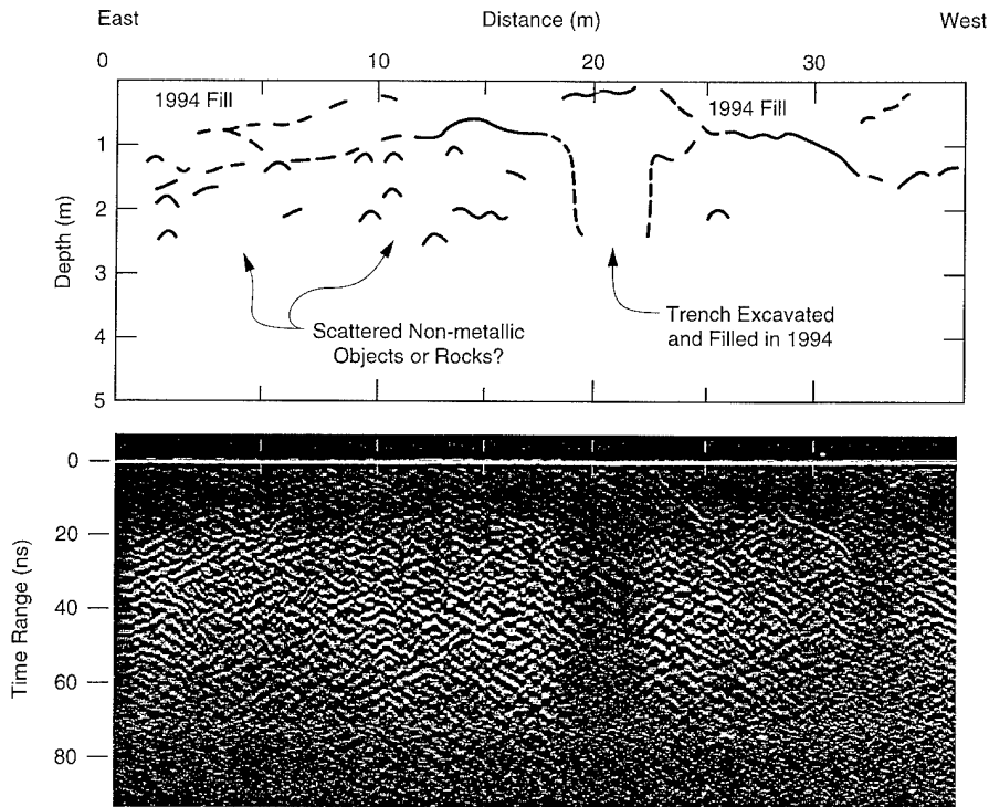
Figure 10. 400-MHz GPR profile recorded along transect 16 in June of 1995. A reflection from the original ground surface (before fill) is clearly visible from stations 24 to 35 m. Signal attenuation resulting from trench excavation and fill is apparent near station 20 m.
