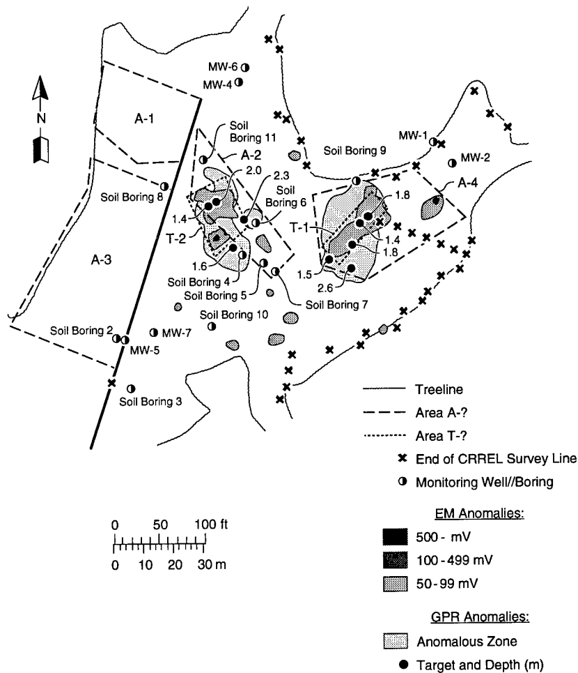
Figure 13. EMI and GPR anomalies east of the CRREL baseline as compiled from data recorded in June 1995. Interpreted depths to targets are in meters below the existing ground surface. CRREL survey lines run from northwest to southeast.
