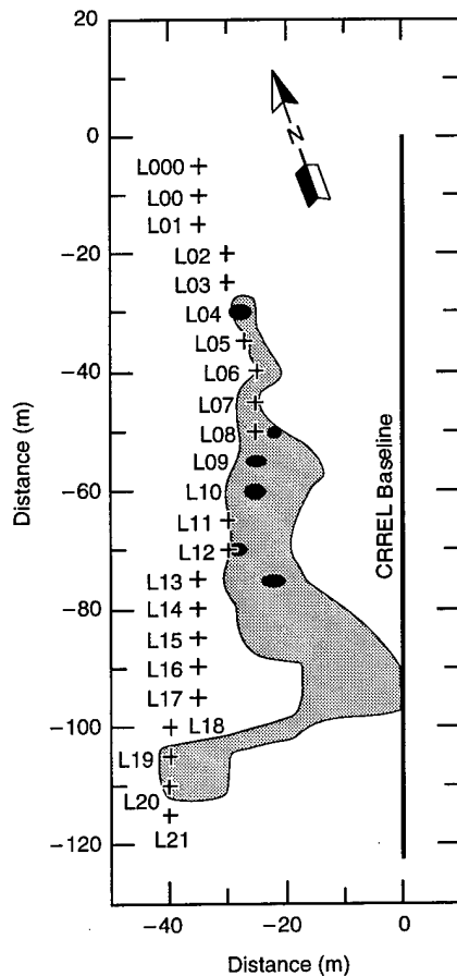
Figure 9. Anomalous zones west of the CRREL baseline as interpreted from the June 1995 survey. It is likely that this zone represents reflections from large boulders within the sands and gravels (transects are numbered L000 to L21).
