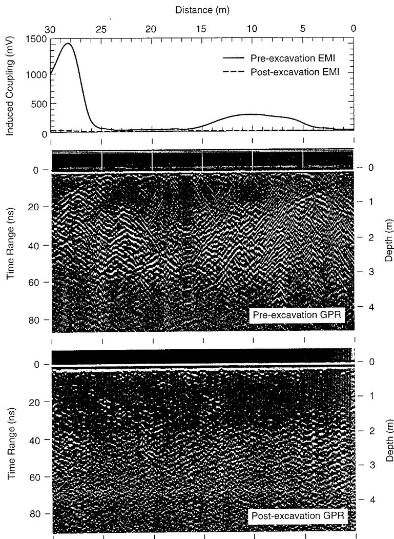
Figure 7. Profiles recorded along transect 02 (area A-4) with GPR and EMI. The data were recorded before (1994) and after (1995) excavation. The excavation, based on the 1994 survey results, revealed 5 yd 3 (3½ m 3 ) of scrap metal and other debris near the broad, low amplitude anomaly. Several 5-gal. (19-L) pails, funnels, and oil-contaminated soil areas were revealed near the sharp anomaly at station 28 m.
