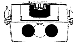
4' or 8' - 1 or 2 Lamp RS
