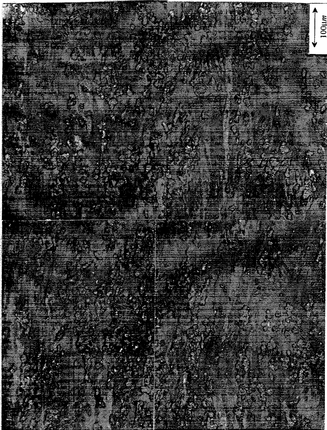
Figure 26: A montage of the 6061 Al - 10 vol. pct. Al 2 O 3 MMC after hot forging to a true strain of 0.51 followed by addition cold deformation to a total strain of 1.20 (McNelley, T.R. and Ballou, M. A., 1995).
