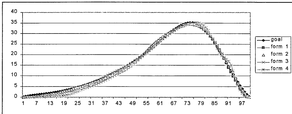
Figure 28: Graphical Results for the MK-Test. This figure shows results obtained for the MK-Test with information on the vertical axis and the percentiles on the horizontal axis. Form 1 to form 4 are the information curves for each form.
