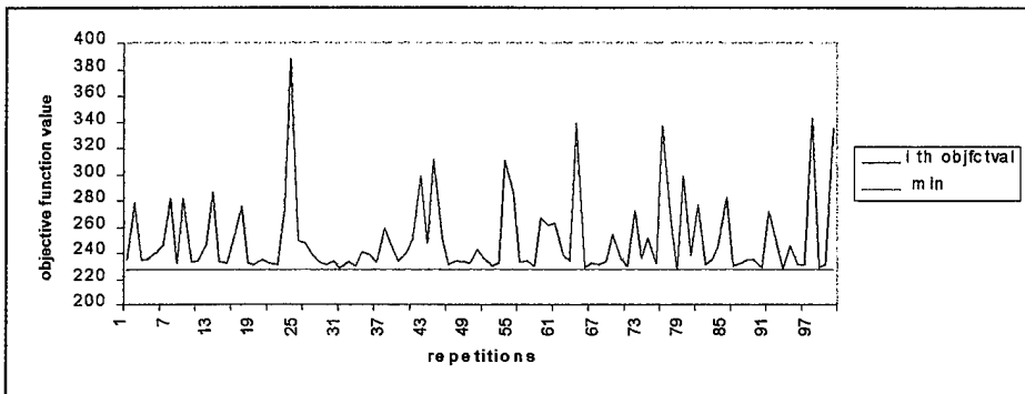
Figure 21: Objective Function Values for each Random Restart.
