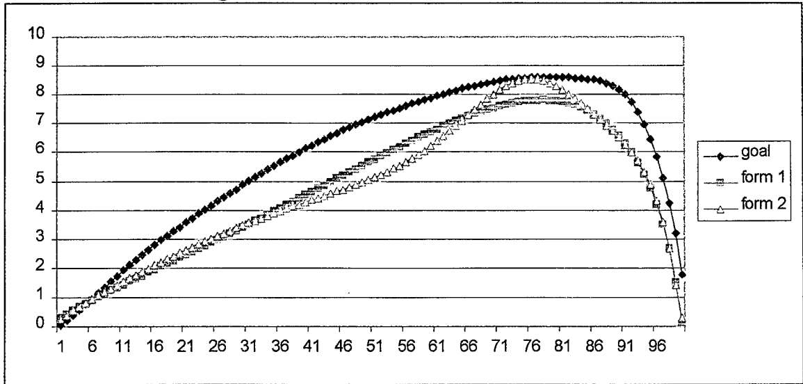
Figure 12: Graphical Results for the EI-Test.
