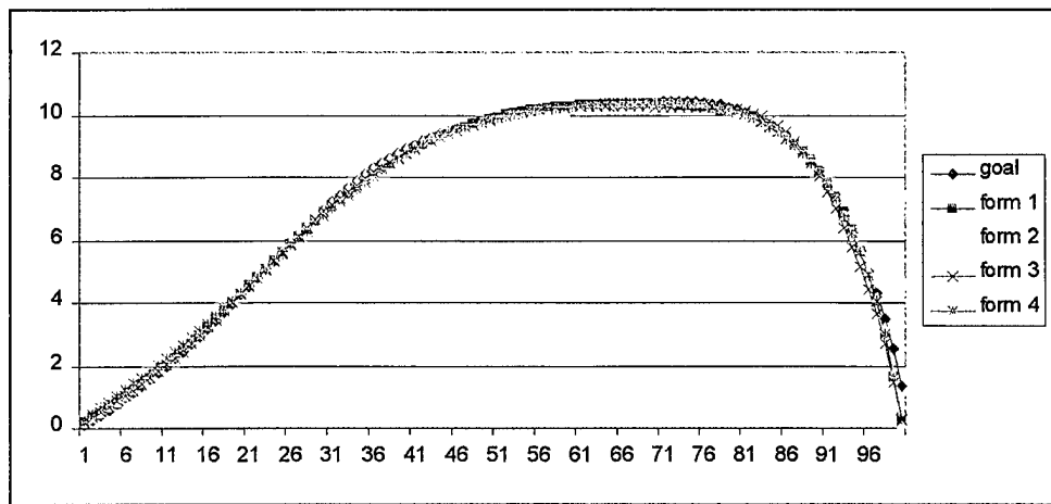
Figure 26: Graphical Results for the MC-Test. This figure shows results obtained for the MC-Test with information on the vertical axis and the percentiles on the horizontal axis. Form 1 to form 4 are the information curves for each form.
