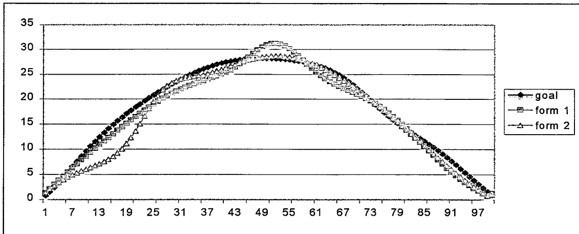
Figure 30: Graphical Results for the WK-Test. This figure shows results obtained for the WK-Test with information on the vertical axis and the percentiles on the horizontal axis. Form 1 and form 2 are the information curves for each form.
