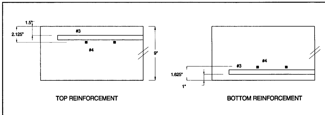
Figure 7. Reinforcement detail.
