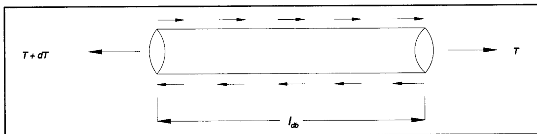
Figure 5. Bond anchorage.
