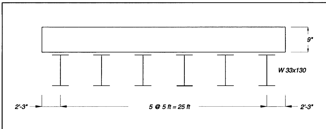
Figure 6. Slab dimensions.
