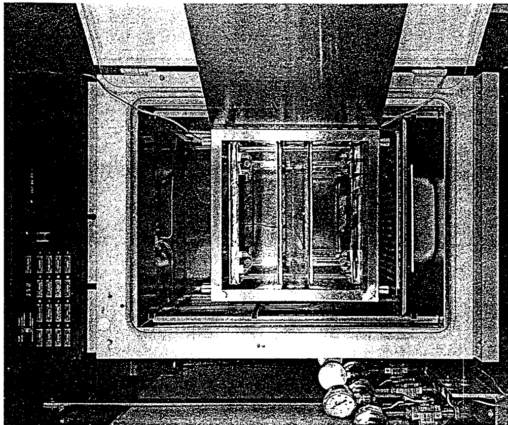
FIG. 3. Cell culture exposure system. Shown is the combination of the four-square Merritt coil and the mu-metal chamber, which are both placed inside a commercial cell culture incubator. Also shown is a thermistor temperature probe, which is threaded through one of the ventilation holes into the mu-metal chamber and placed inside the chamber at the position where cell culture plates are typically located.
