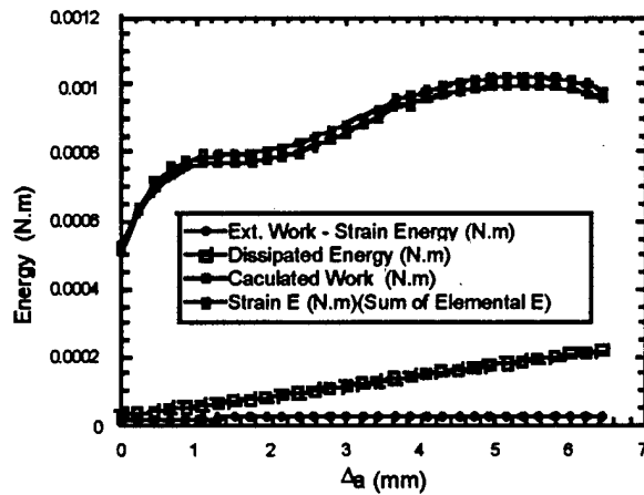
Fig. 7 Energy vs crack extension of alumina
