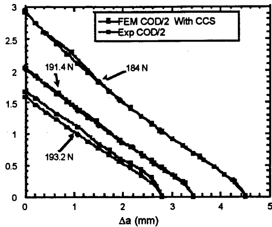
Fig. 6 COD profile vs crack extension of alumina
