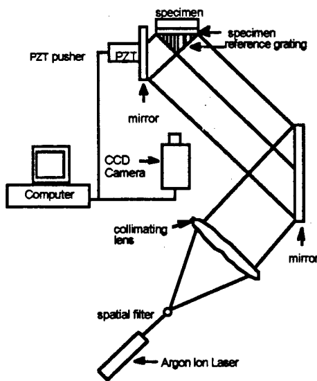
Fig. 4 Phase shifting Moiré interferometry setup
