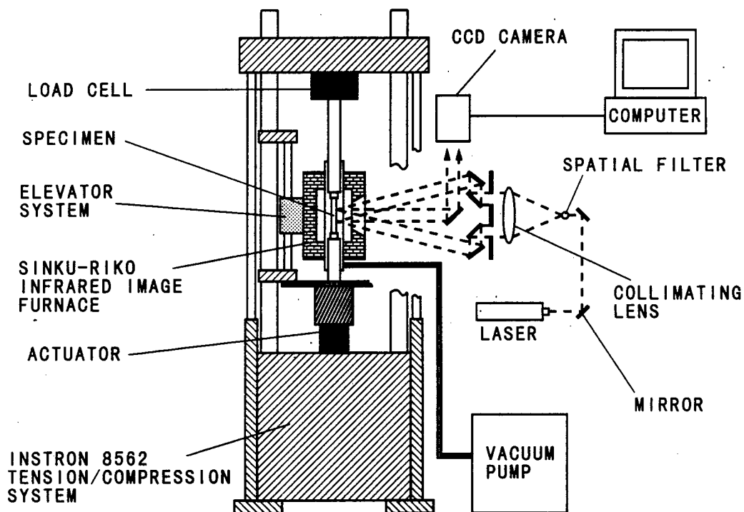
Fig. 1 High temperature testing system
