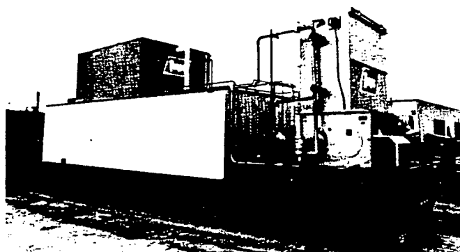
HP200SCE – A complete packaged system with an HP200SCE, evaporative condenser and insulated steel storage tank.
