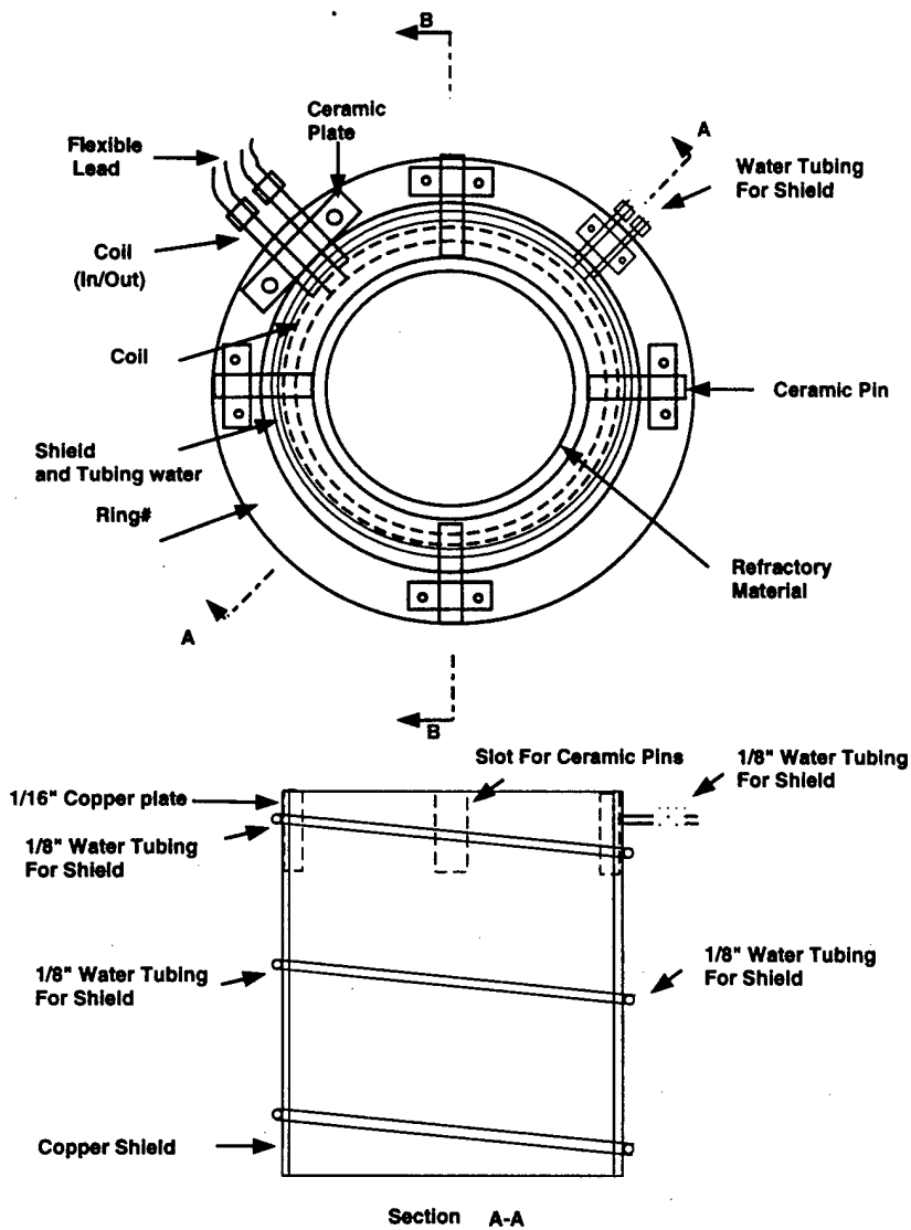
Fig. 1: Schematic of target holder-section A-A.
