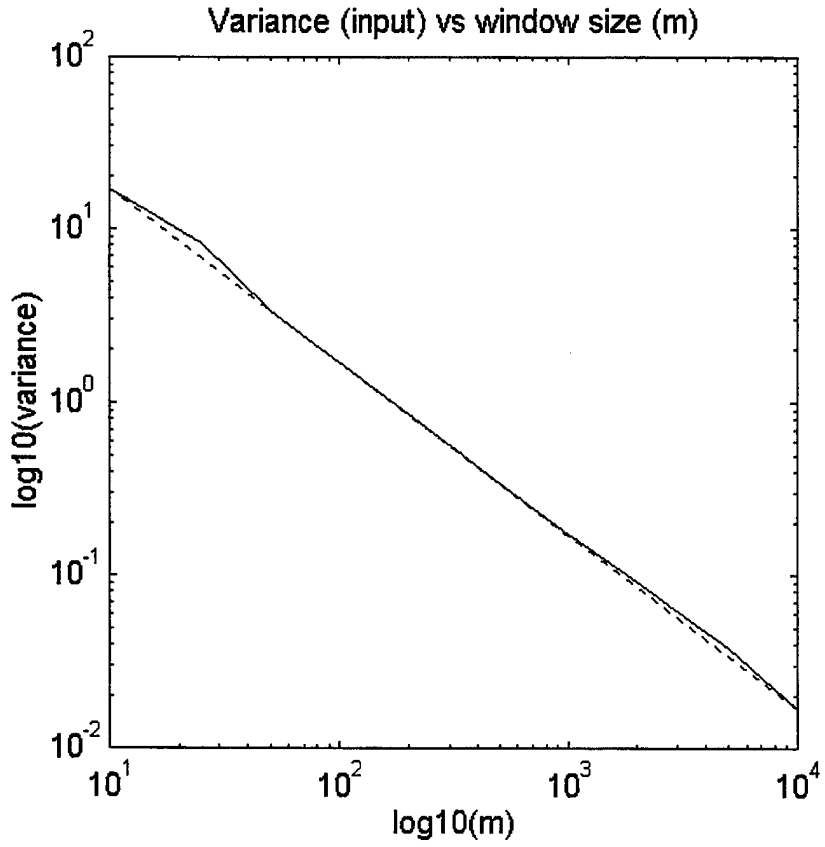
Figure 5.12: Variance-Time Curve, Video/Audio Traffic (Measured)
