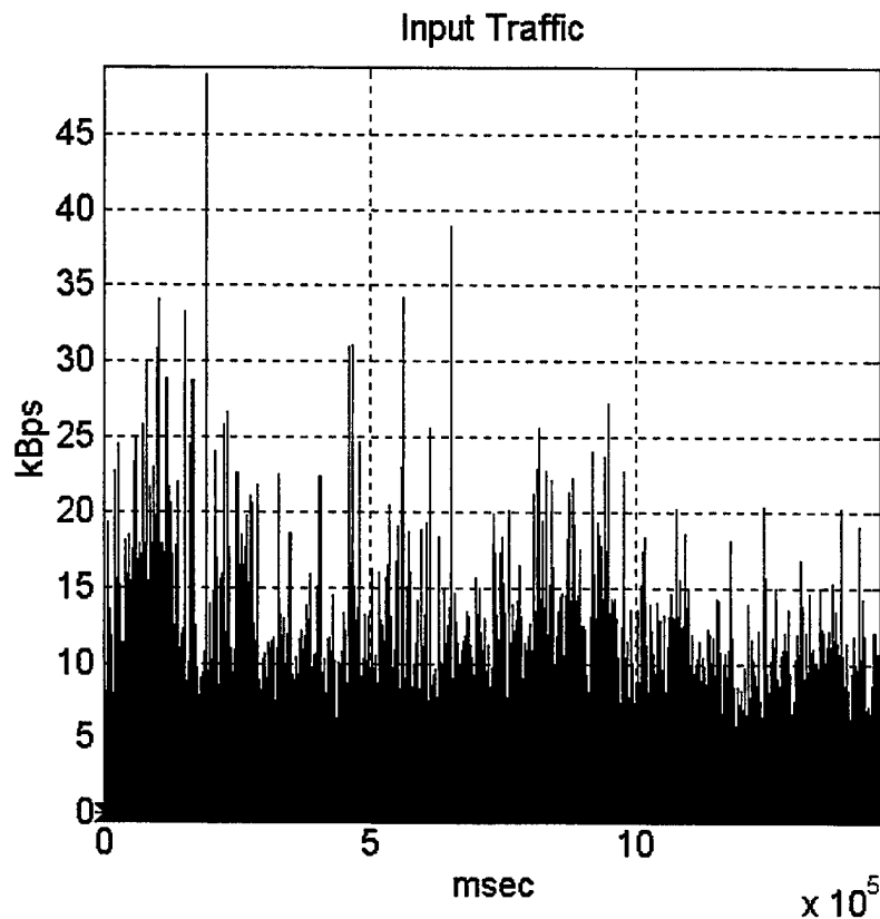
Figure 5.8: Input Traffic at Computer Interface, Video/Audio
