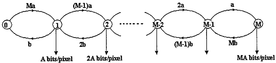
Figure 4.2: Markov Chain Representation of VBR Source
