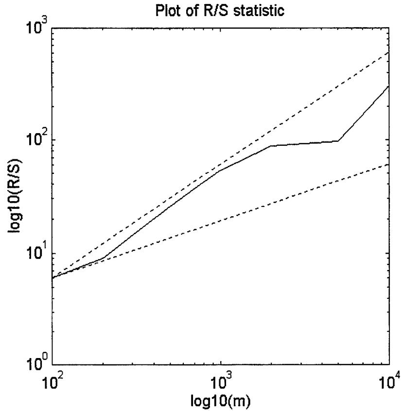
Figure 5.3: Plot of R/S Statistic, Video-Only Traffic (Measured)
