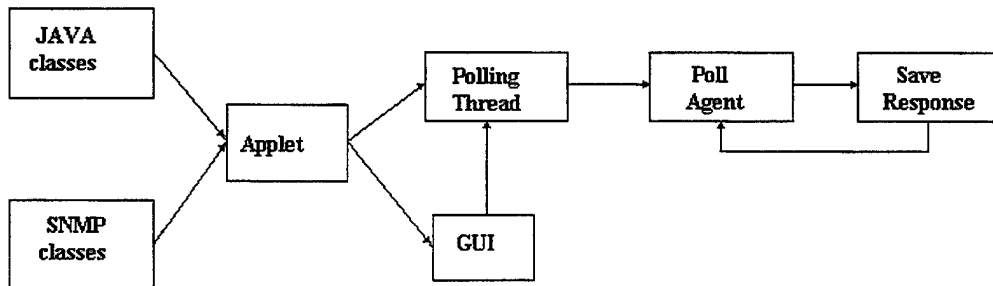
Figure 3.7: Java-SNMP Applet Flow Diagram
