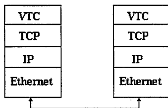
Figure 3.3: Layered Model
