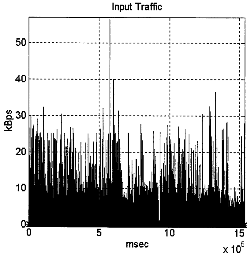
Figure 5.1: Input Traffic Into Computer Interface, Video Only
