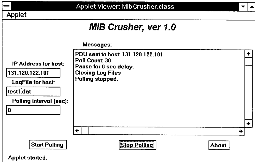
Figure 3.8: Graphical User Interface for Java-SNMP Applet
