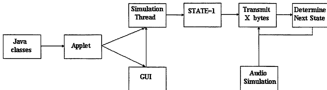
Figure 4.5: Audio/Video Simulation Applet Flow Diagram
