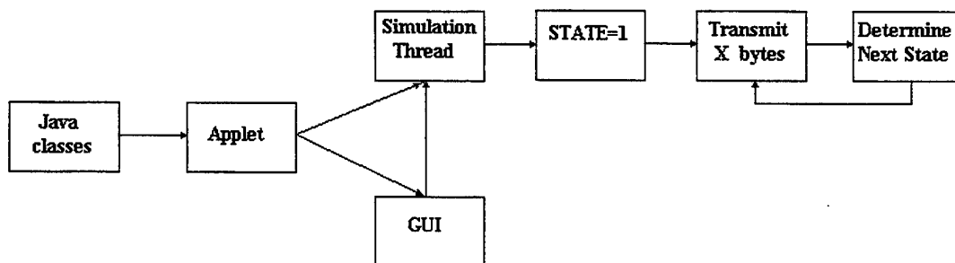
4.3: Video Source Simulation Applet Flow Diagram
