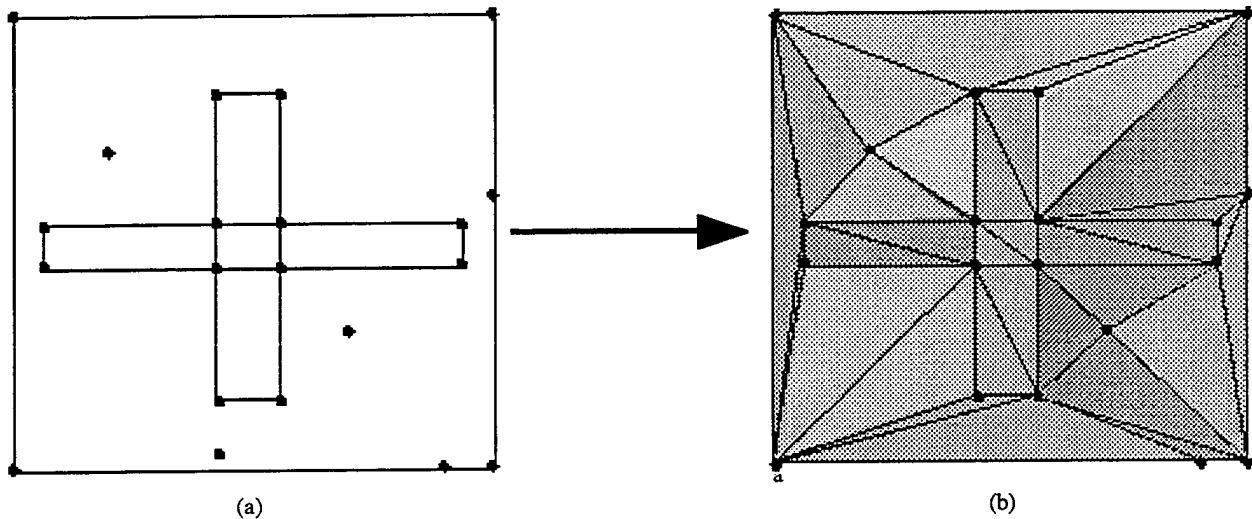
Figure 5. Terrain Triangulation.
