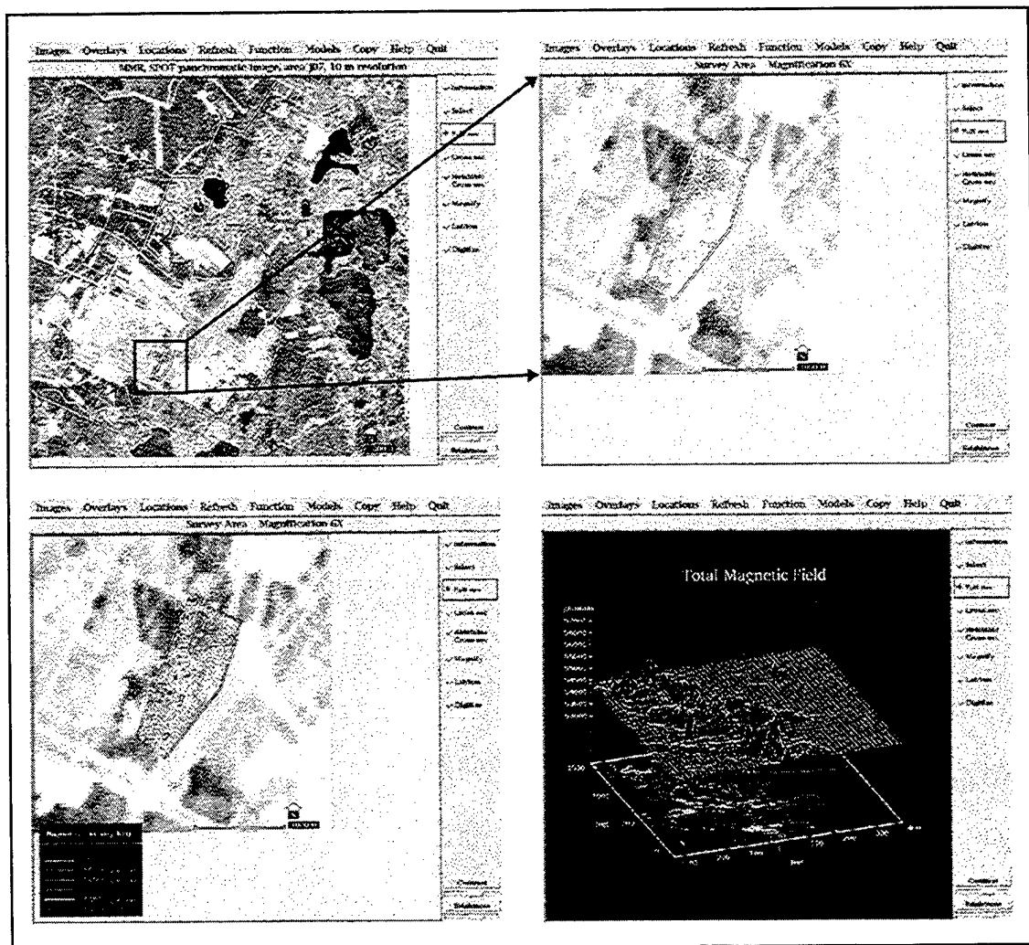
Figure 16. Magnetic Survey
