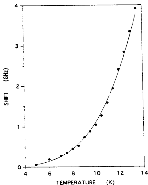
FIG. 1 Observed temperature shift of the frequency. The solid line shows the curve \delta\nu(T) = 8.893 \times 10^{-2} T^{4.096} MHz, which was obtained by least squares fit of the observed \delta\nu .
