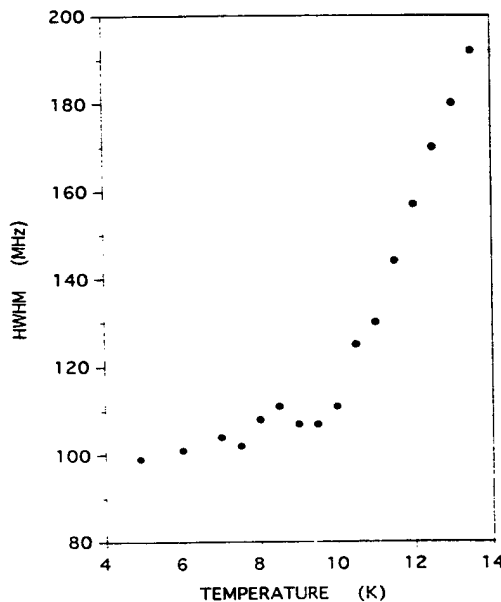
Observed temperature dependence of the linewidths.
