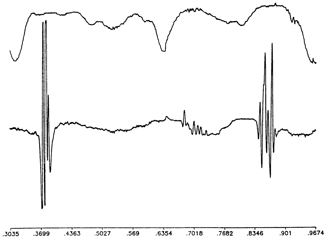
FIGURE 2 The entire Q_3(0) absorption spectrum recorded with toneburst modulation for the laser polarization parallel to the c -axis. The zero of the x -axis corresponds to 11758.000 \text{ cm}^{-1} . The upper trace gives iodine reference lines.
